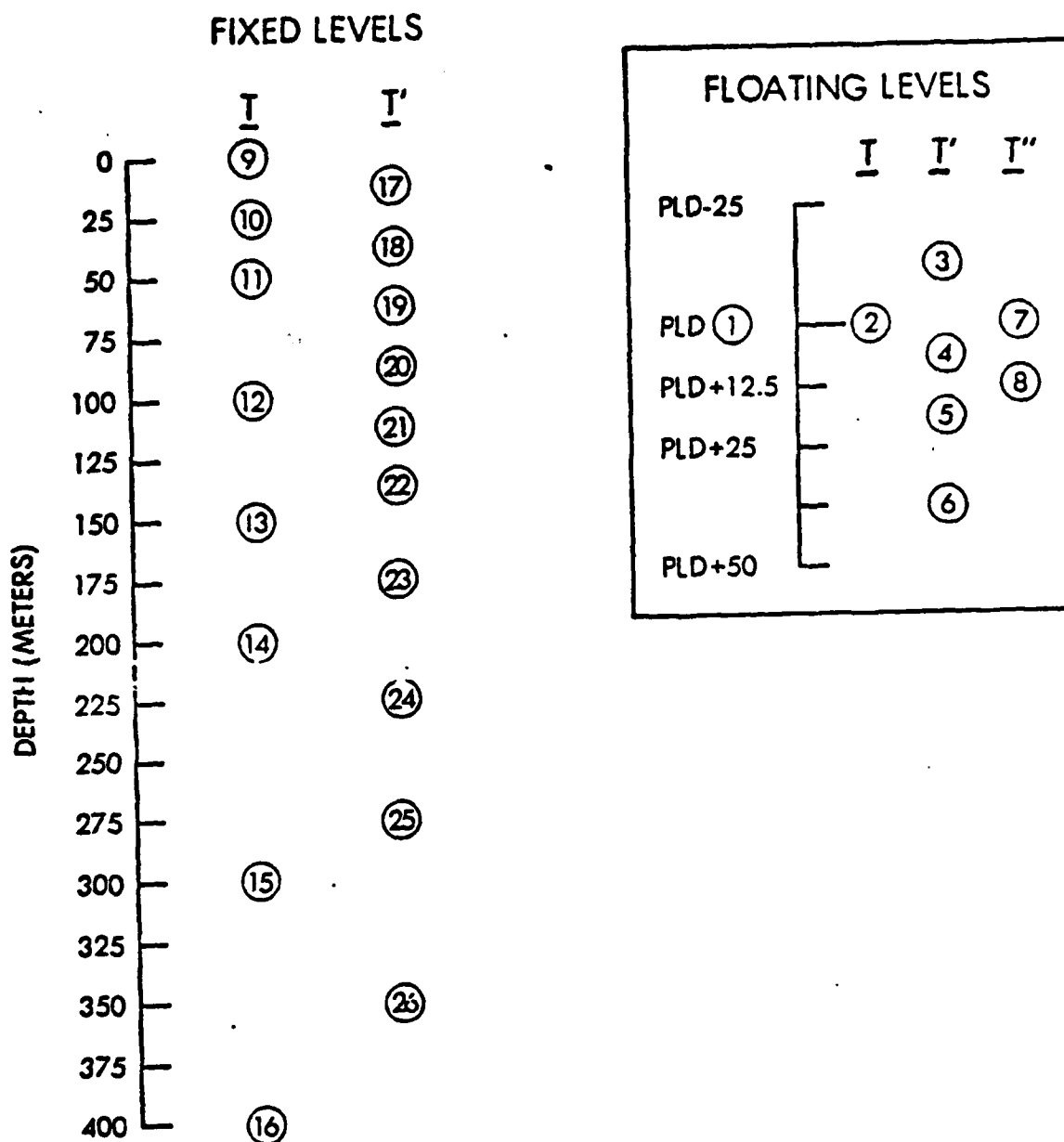
Figure 40. The twenty-six TOPS-EOTS ocean thermal structure parameters. Labeled T , T' and T'' are temperature, first vertical temperature difference and second vertical temperature difference, respectively. Parameters 2-8 are associated with floating levels defined relative to parameter 1, Primary Layer Depth (PLD). Parameters 9-26 are associated with fixed levels. [Clancy and Pollack, 1982]
