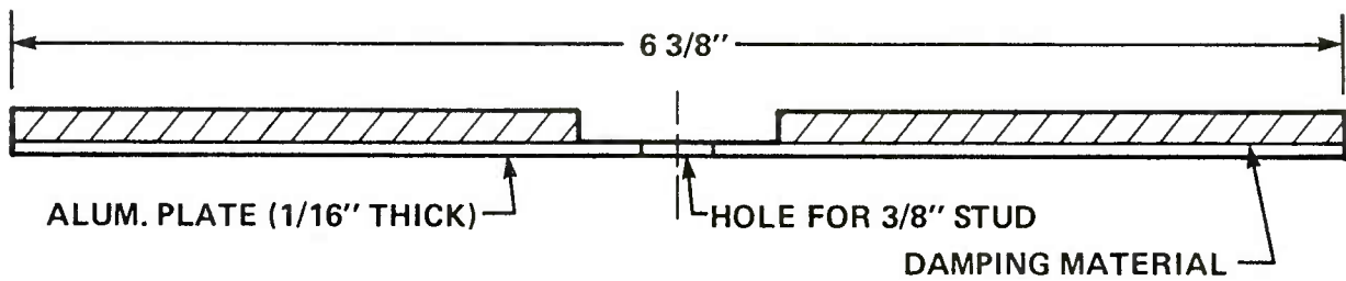
FIG. 7. PATTERN FOR 8-SPIRAL DISK.
