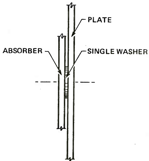
c. ABSORBER EPOXIED TO PLATE
