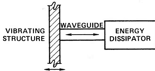
FIG. 2. SCHEMATIC DIAGRAM OF WAVEGUIDE ABSORBER ACTION
