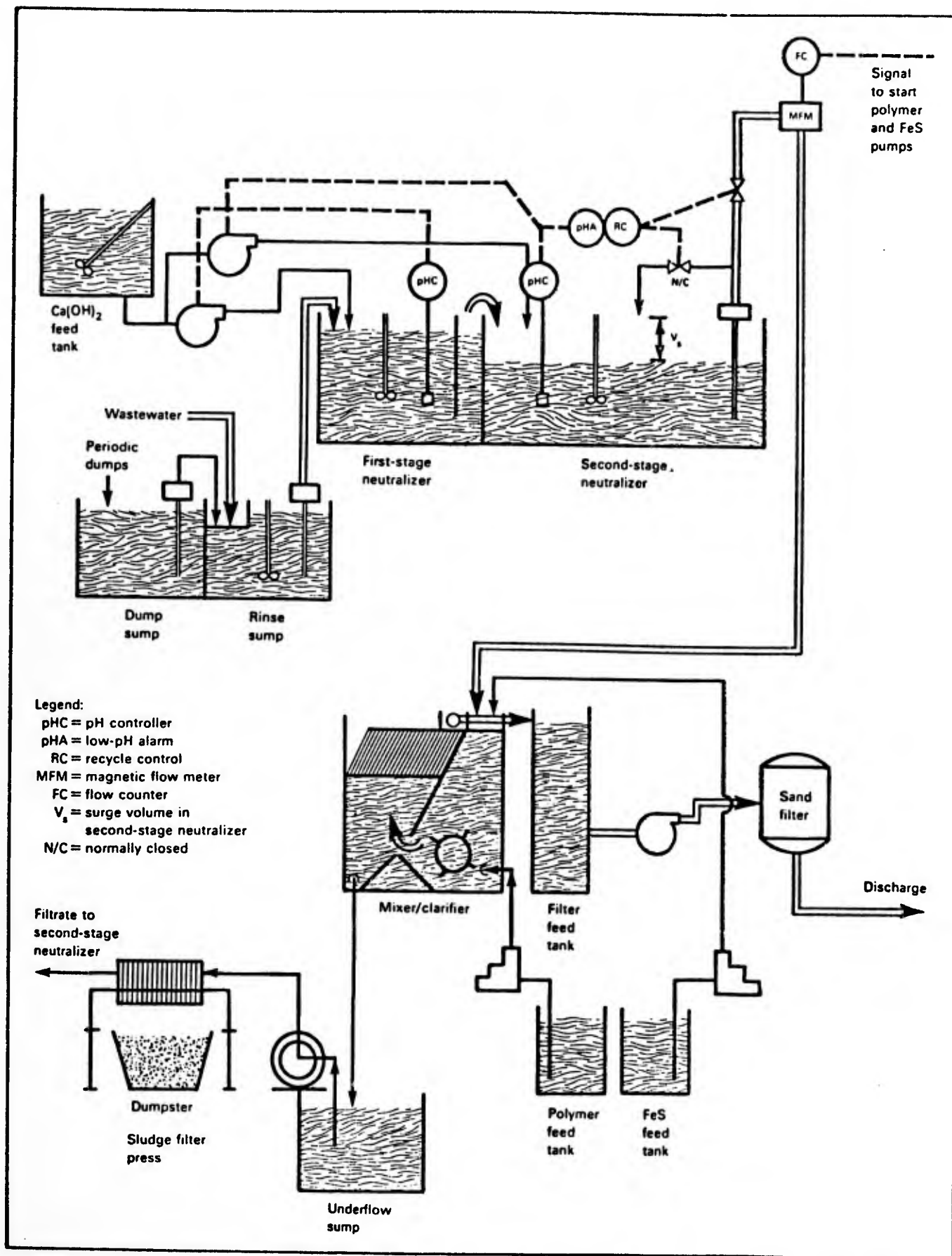
Figure 30. Insoluble Sulfide Treatment Process Components
