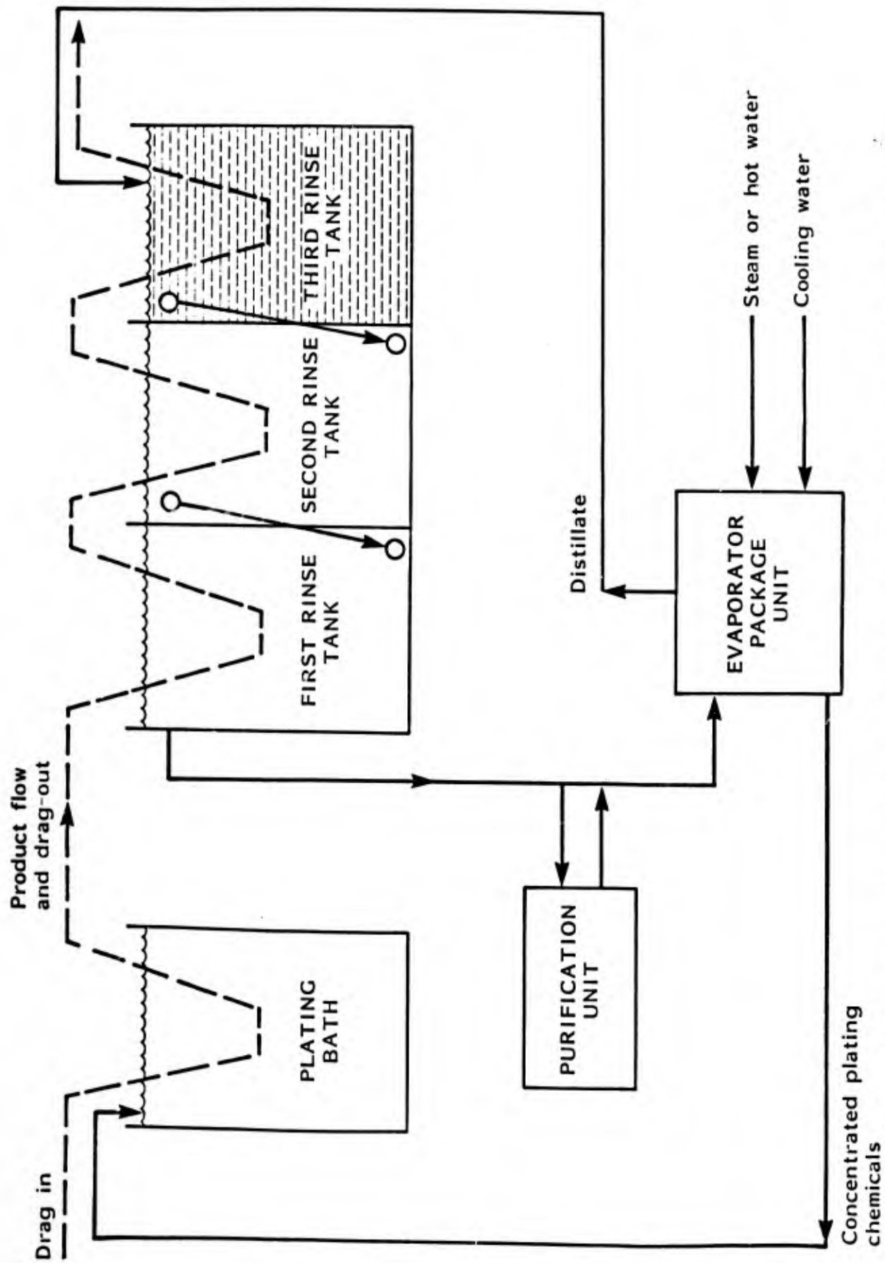
Figure 51. Closed-Loop Evaporative Recovery of Plating Chemicals from Drag-Out
