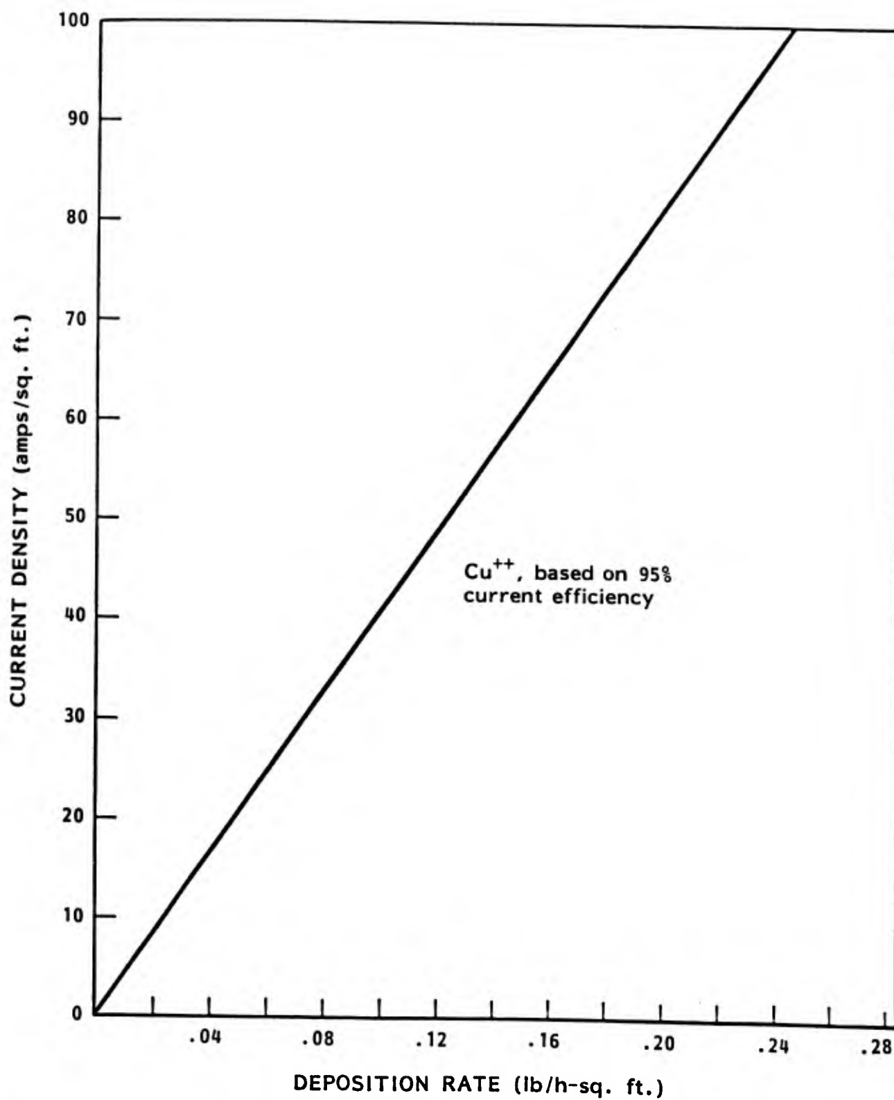
Figure 74. Maximum Current Density for Copper Electrowinning
