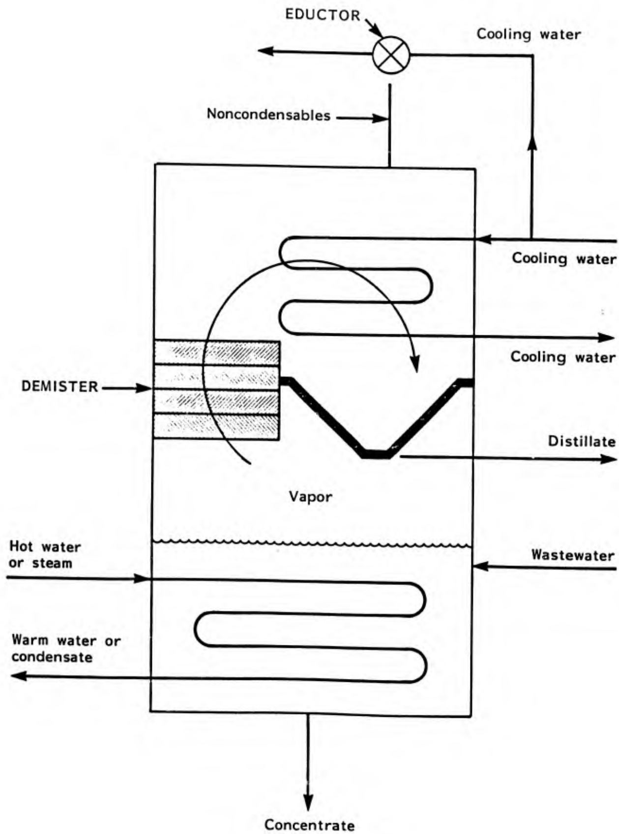
Figure 54. Submerged Tube Evaporation for Chemical Recovery
