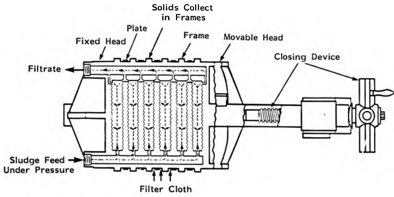
Figure 24. Plate-and-Frame Filter Press
