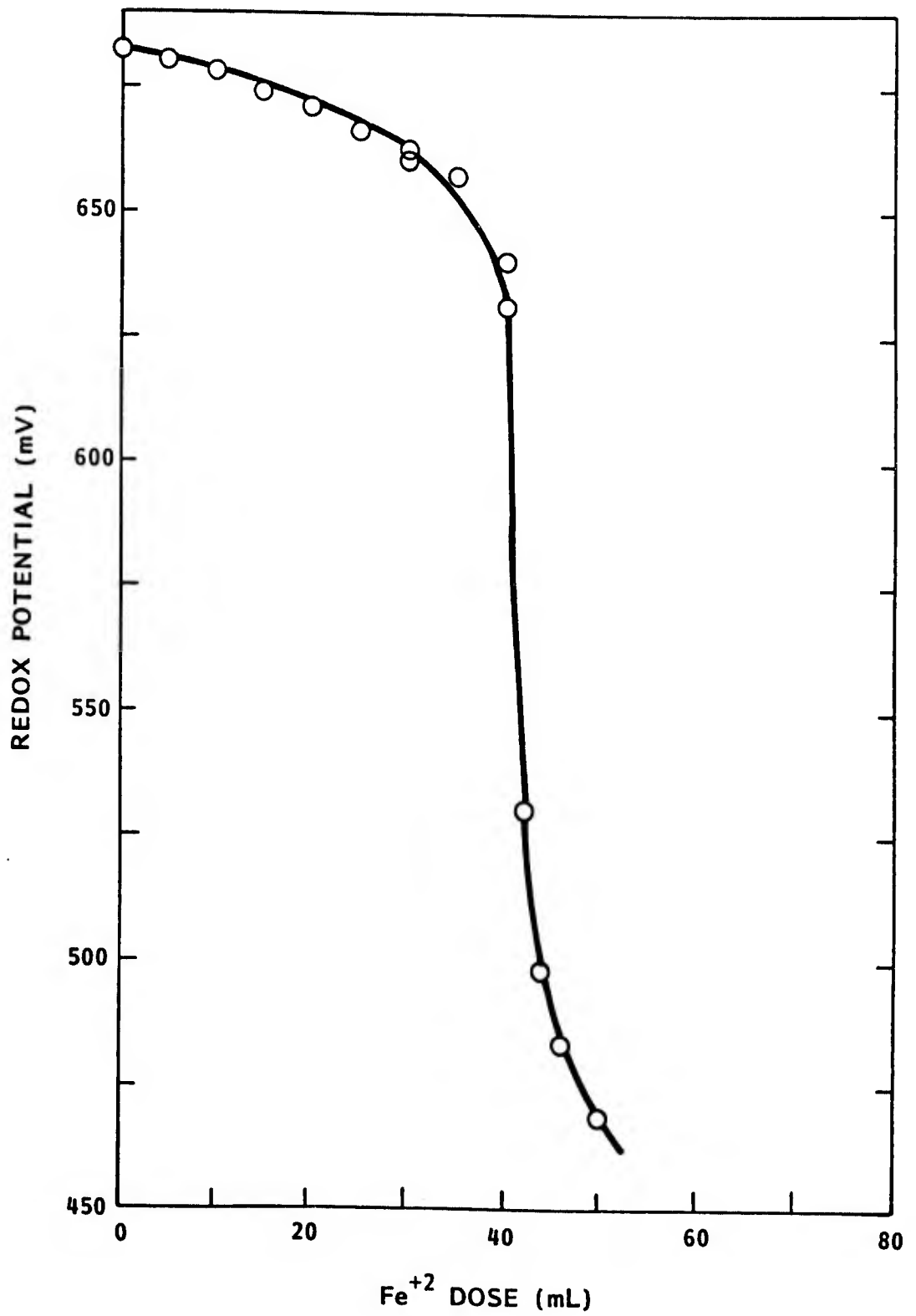
Figure 46. Redox Potential Control Set Point for FeSO 4 Chromium Reduction
