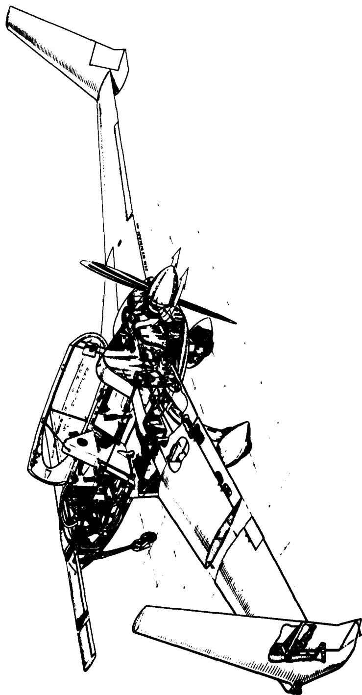
Figure 2. General Construction
