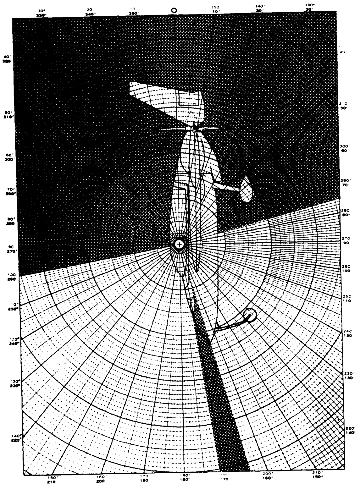
Figure 50. Longitudinal Field-of-View
