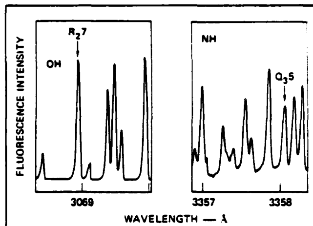
Fig. 2. Excitation scans through portions of the (0, 0) bands of the A^2\Sigma^+ - X^2\Pi_1 system of OH and the A^3\Pi_1 - X^3\Sigma^- system of NH. The medium is the reaction zone of a CH_4/N_2O flame at atmospheric pressure. From the relative intensities and an estimate that Q/A is the same for each species, it was found that [NH]/[OH] \approx 0.04 .
