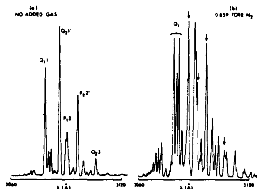
Figure 5. Fluorescence scans of the (0,0) band of the A^2\Sigma^+-X^2\Pi_1 system of the OH molecule, following pumping of the N=1, J=1\frac{1}{2} level. a , No added gas. The five rotational lines marked are those emitted by the pumped level (a few small lines are due to collisions with the background gases H_2O and NO_2 ; also, laser scatter is partially responsible for the width of the feature in the P_1(2) region). b , Spectrum with added N_2 , at 0.86 torr. The Q_1 series is marked as are (with arrows) the remaining four branches noted in ( a ). The new lines are fluorescence emitted from other rotational levels, populated by energy transfer collisions with the N_2 . [Reprinted from the Journal of Chemical Physics ]
