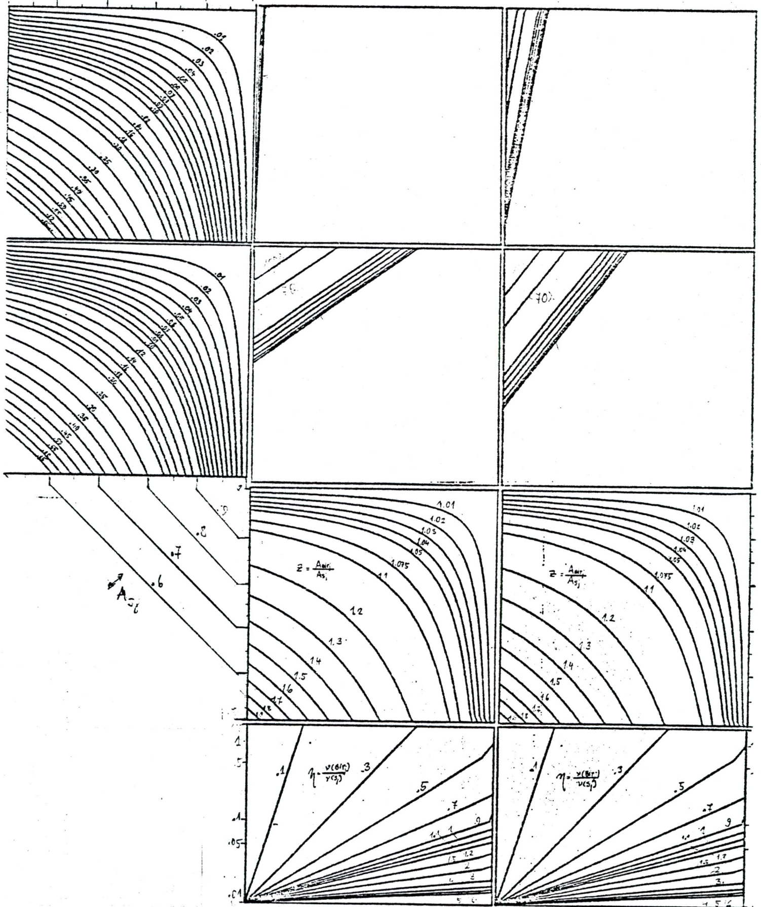
Figure 15: Case 2 and 3. Nomogram for % of improvement of A_j .
