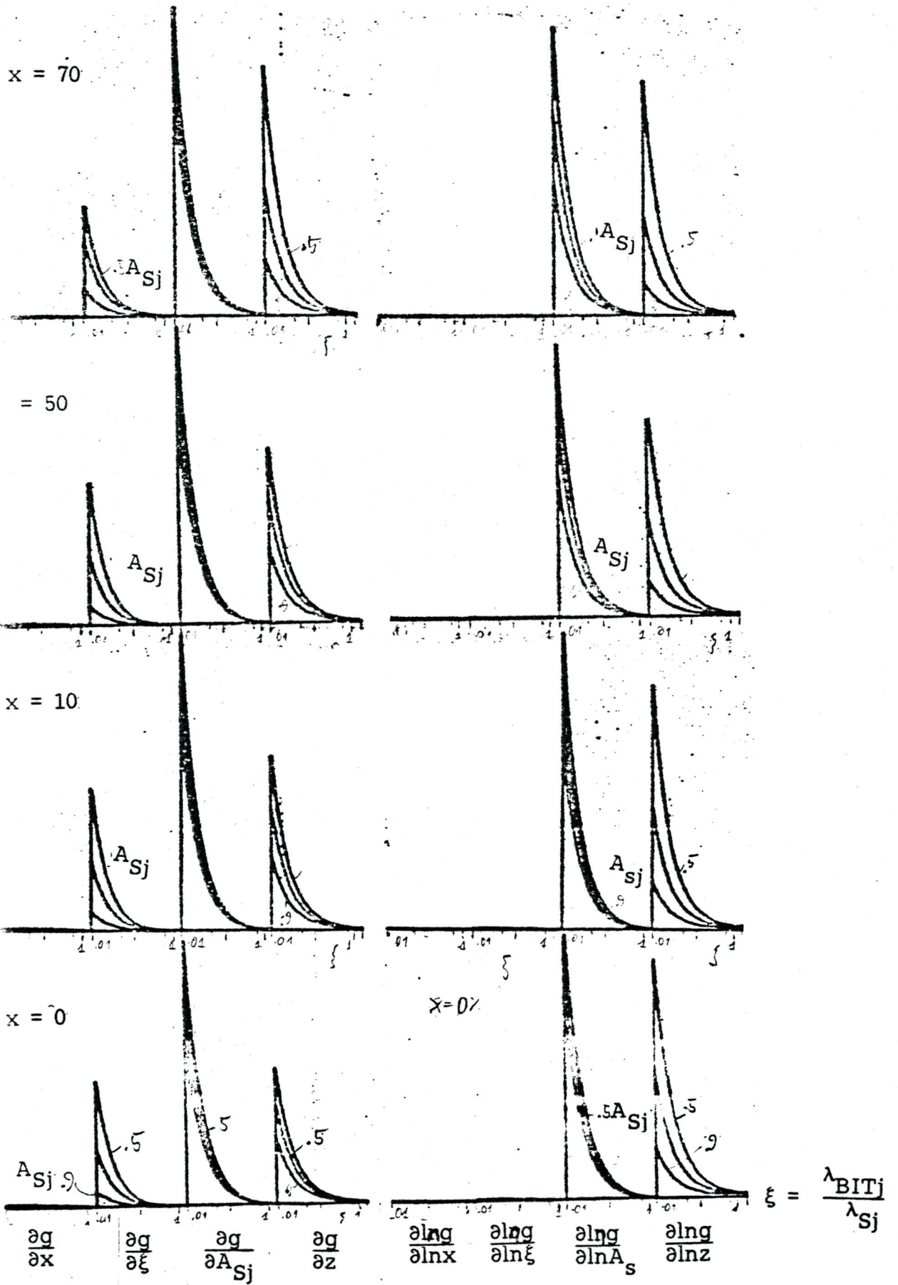
Fig. 8: Partial derivatives and sensitivity coefficients as on the figure 1, but now as functions of \xi = \lambda_{BITj} / \lambda_{Sj} .
