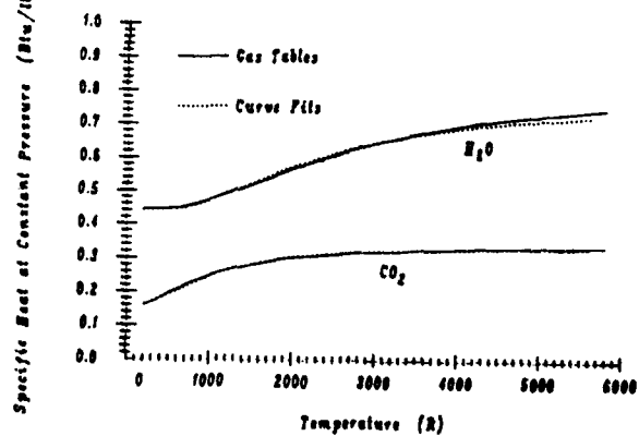
Figure 3. Agreement Between Tabulated Data and Curve Fits
