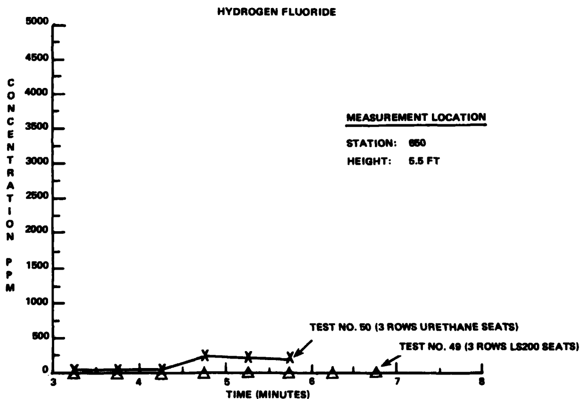
FIGURE B-8. EFFECT OF CUSHIONING PROTECTION AND MATERIALS ON HF AND HCl LEVELS IN IN-FLIGHT FIRES
