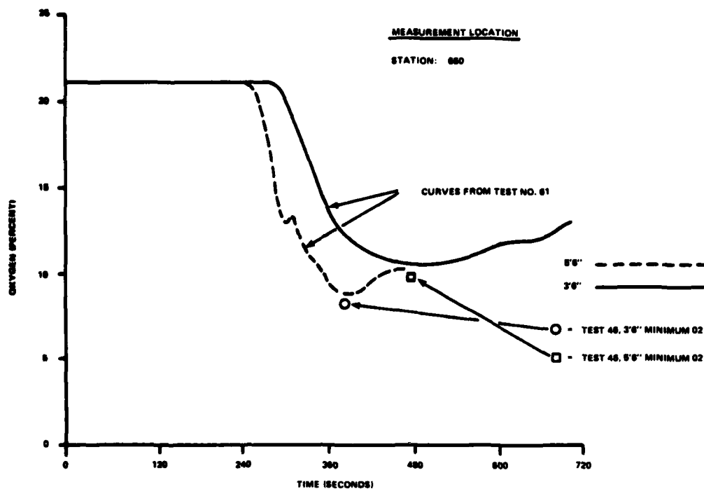
FIGURE 56. FULL-SCALE IN-FLIGHT OXYGEN COMPARISONS
