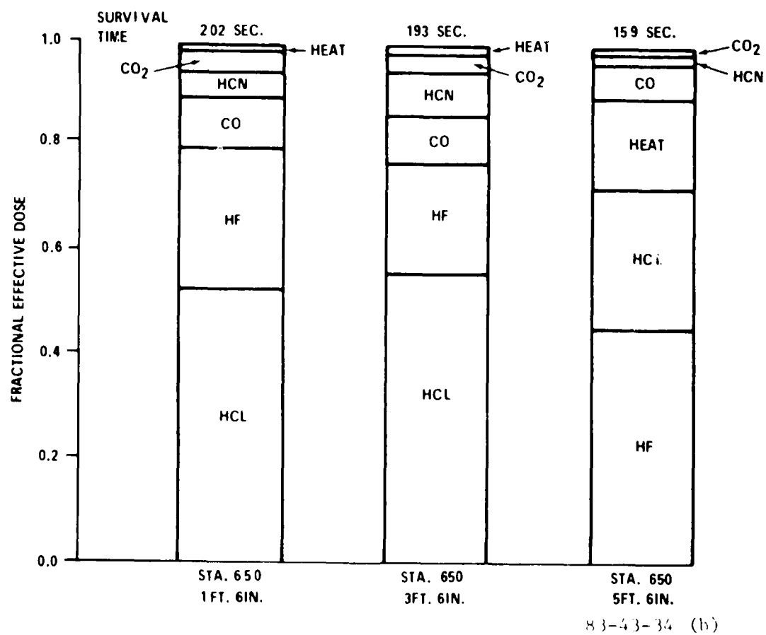
FIGURE 34. EFFECT OF ELEVATION ON SURVIVABILITY IN AFT CABIN
