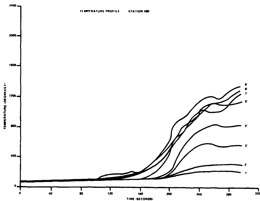
FIGURE C-2. TEMPERATURE PROFILE STATION 480 (1 of 2 Sheets)
