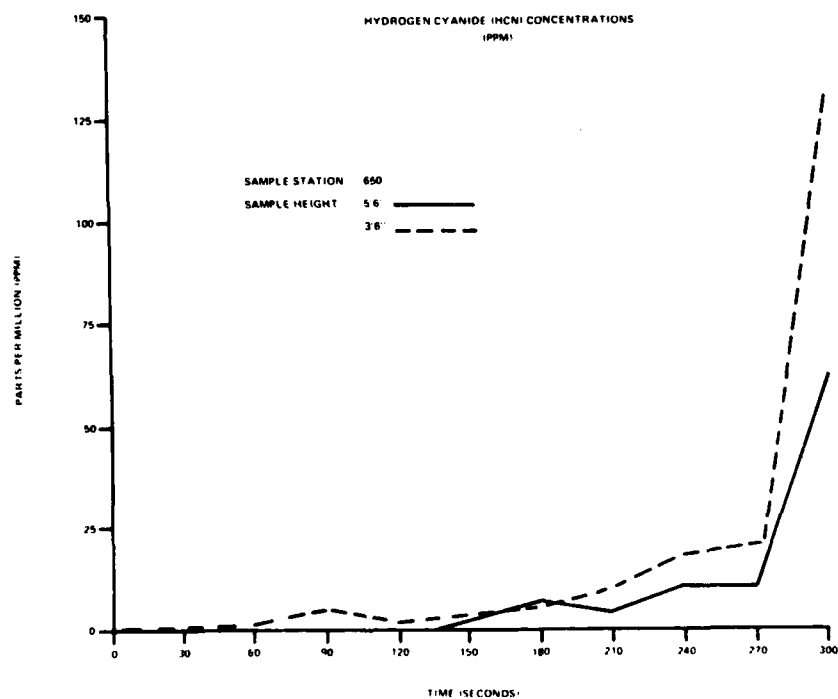
FIGURE C-11. HCN PROFILE STATION 650 (1 of 2 Sheets)
