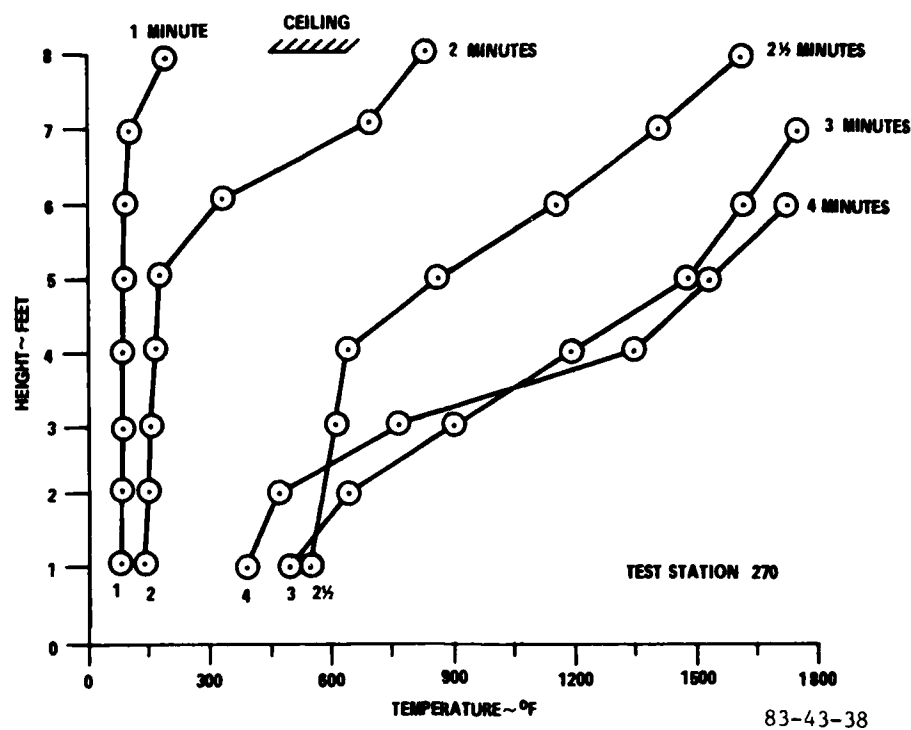
FIGURE 38. HEAT STRATIFICATION IN FORWARD CABIN
