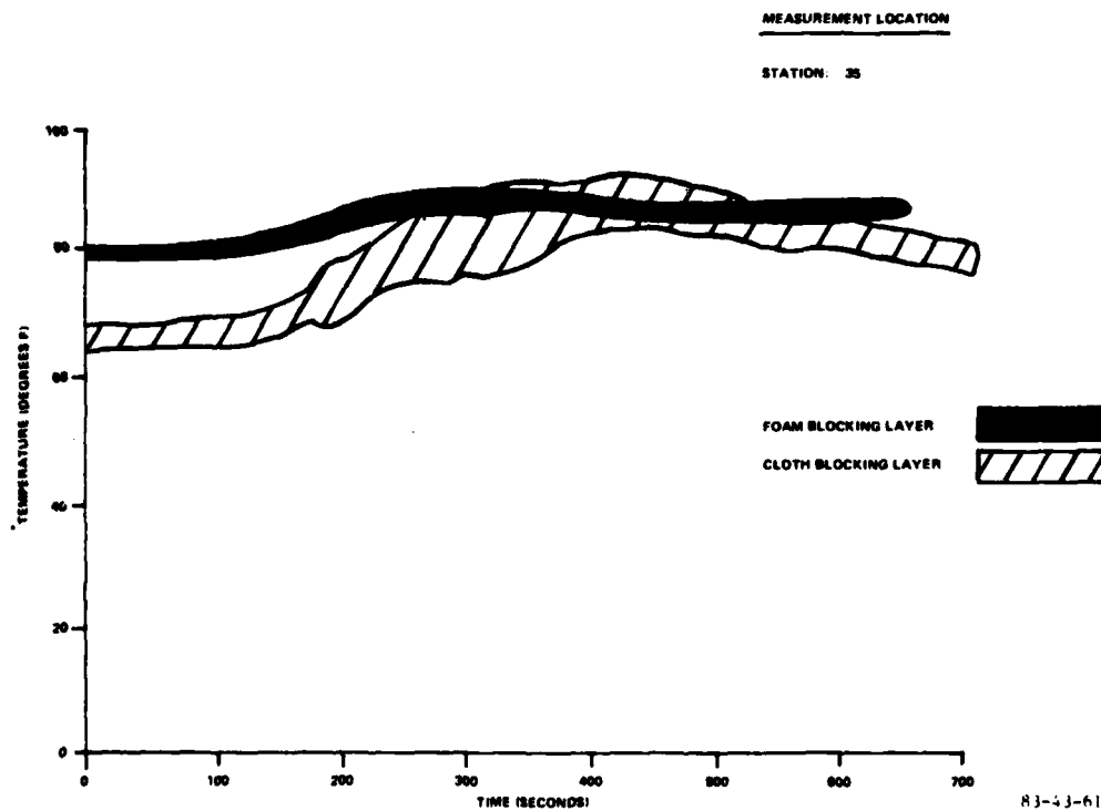
FIGURE 61. RANGE OF TEMPERATURE MEASUREMENTS FROM FLOOR TO CEILING
