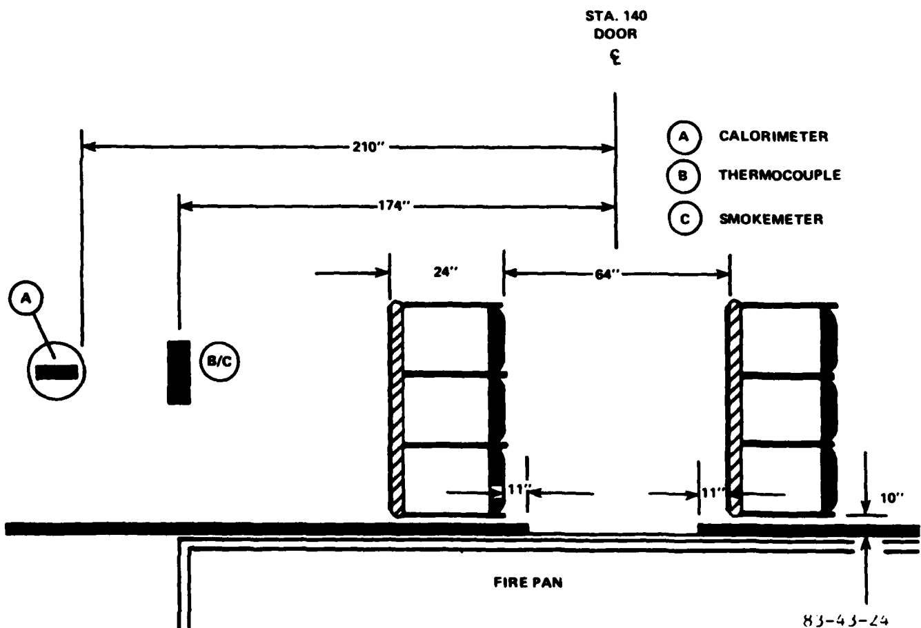
FIGURE 24. POST-CRASH SERIES FIVE CONFIGURATION
