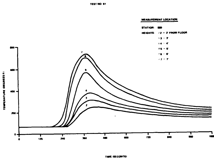
FIGURE 52. FULL-SCALE IN-FLIGHT TEMPERATURE PROFILE
