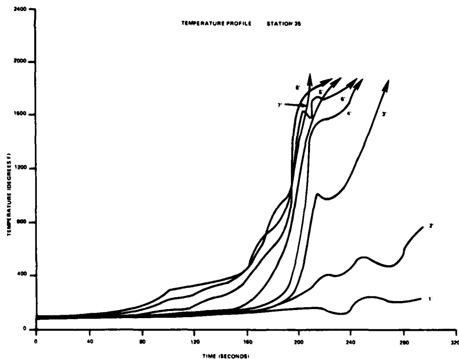
FIGURE C-1. TEMPERATURE PROFILE STATION 35 (1 of 2 Sheets)
