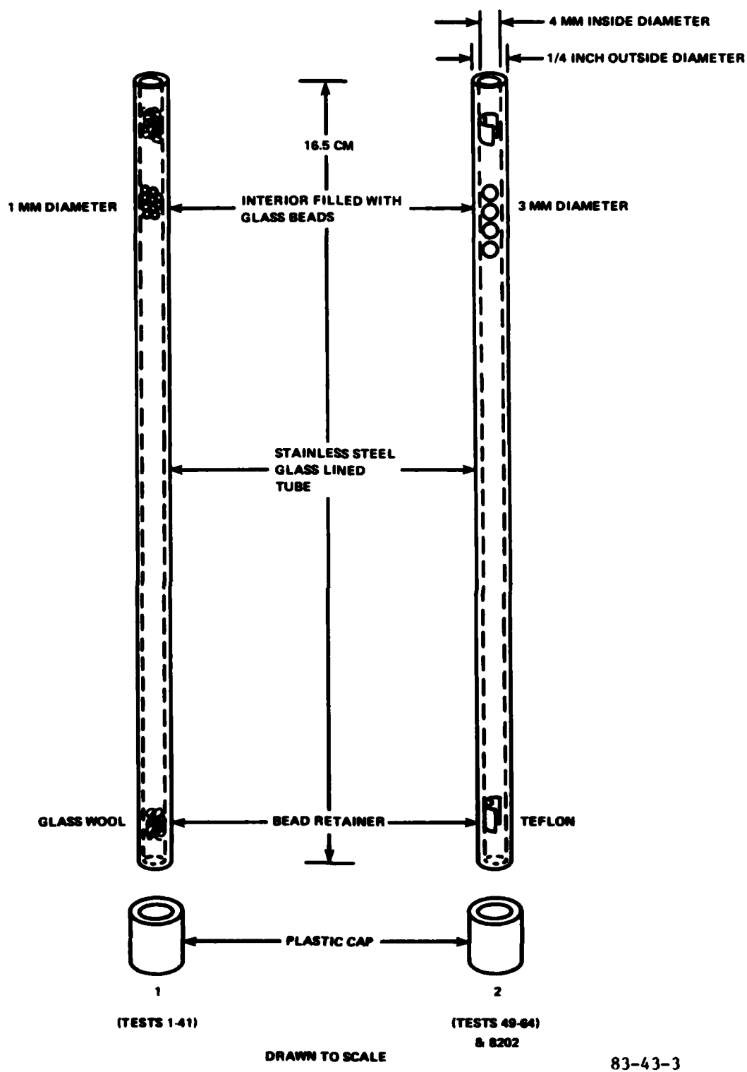
FIGURE B-3. ABSORPTION TUBES
