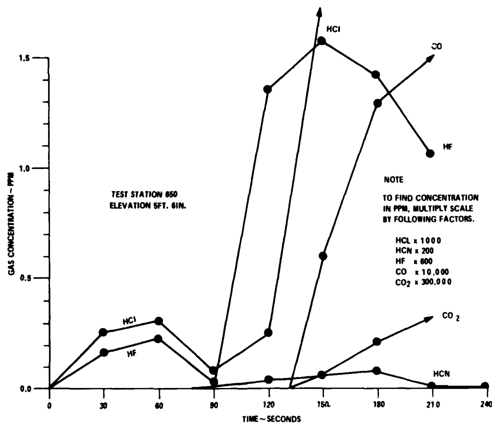
FIGURE 32. HAZARDS IN AFT CABIN PRODUCED BY BURNING INTERIOR MATERIALS
