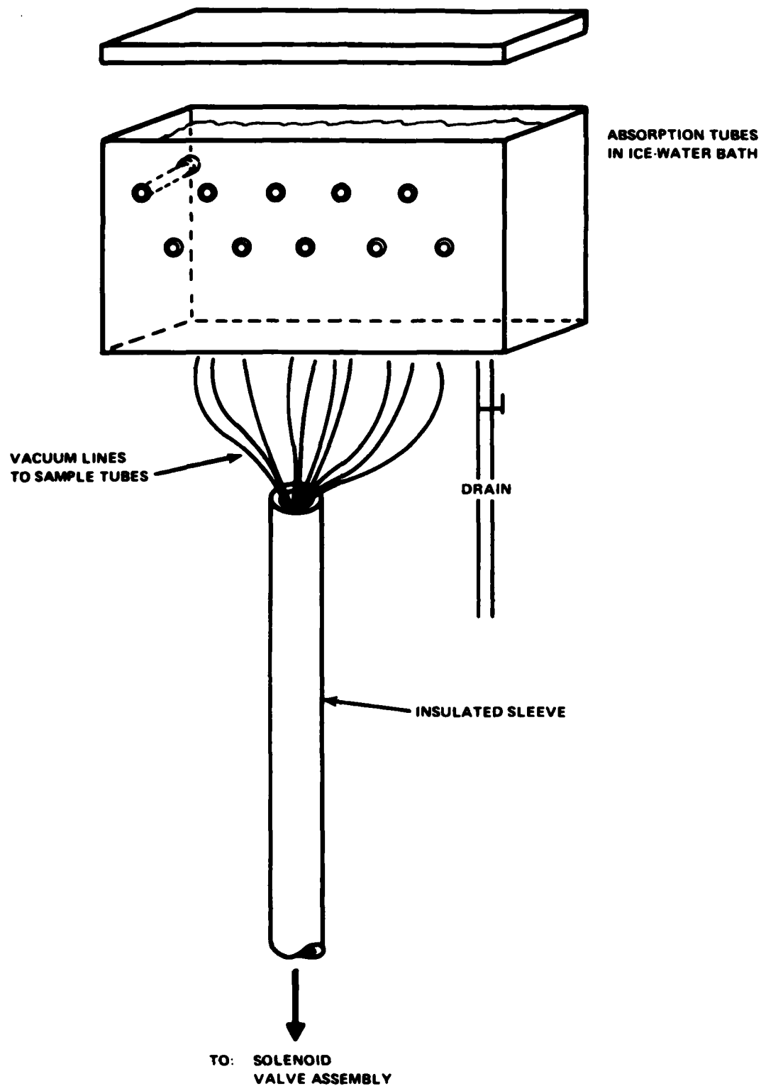
FIGURE B-1. C133 ACID GAS SAMPLING STATION
