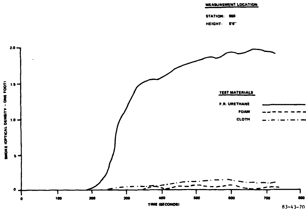
FIGURE 70. RAMP FIRE BLOCKING LAYER SMOKE COMPARISON
