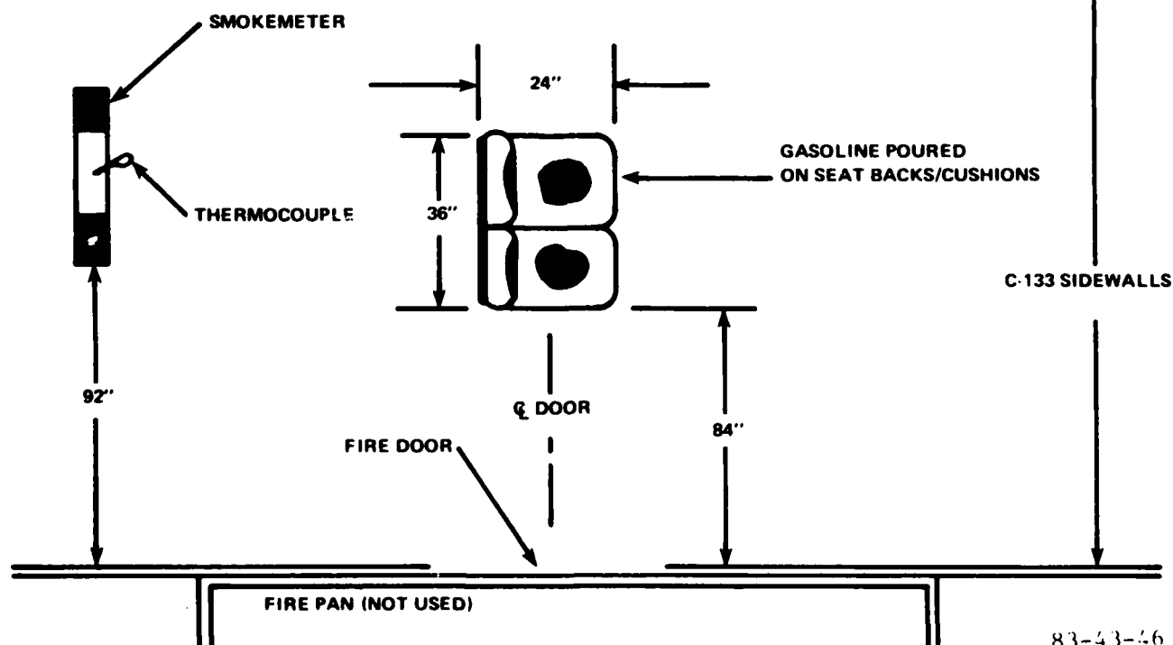
FIGURE 46. IN-FLIGHT GASOLINE TEST CONFIGURATIONS
