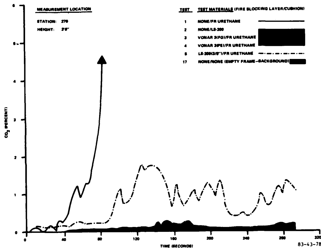
FIGURE 7. POST-CRASH SERIES ONE GAS COMPARISON
