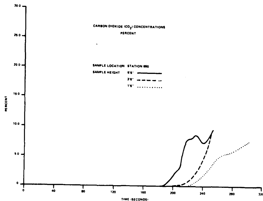
FIGURE C-5. \text{CO}_2 PROFILE STATION 650 (1 of 2 Sheets)
