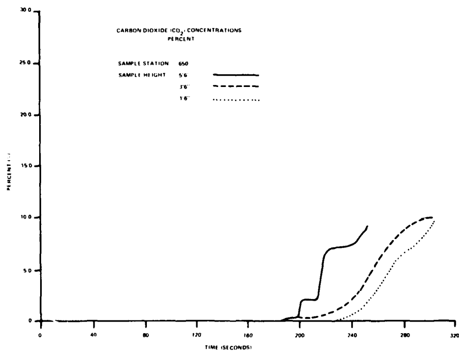
FIGURE C-5. \text{CO}_2 PROFILE STATION 650 (2 of 2 Sheets)
