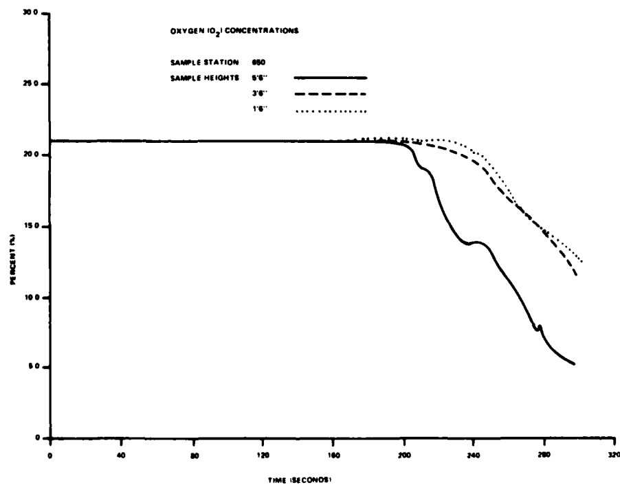
FIGURE C-9. O_2 PROFILE STATION 650 (2 of 2 Sheets)
