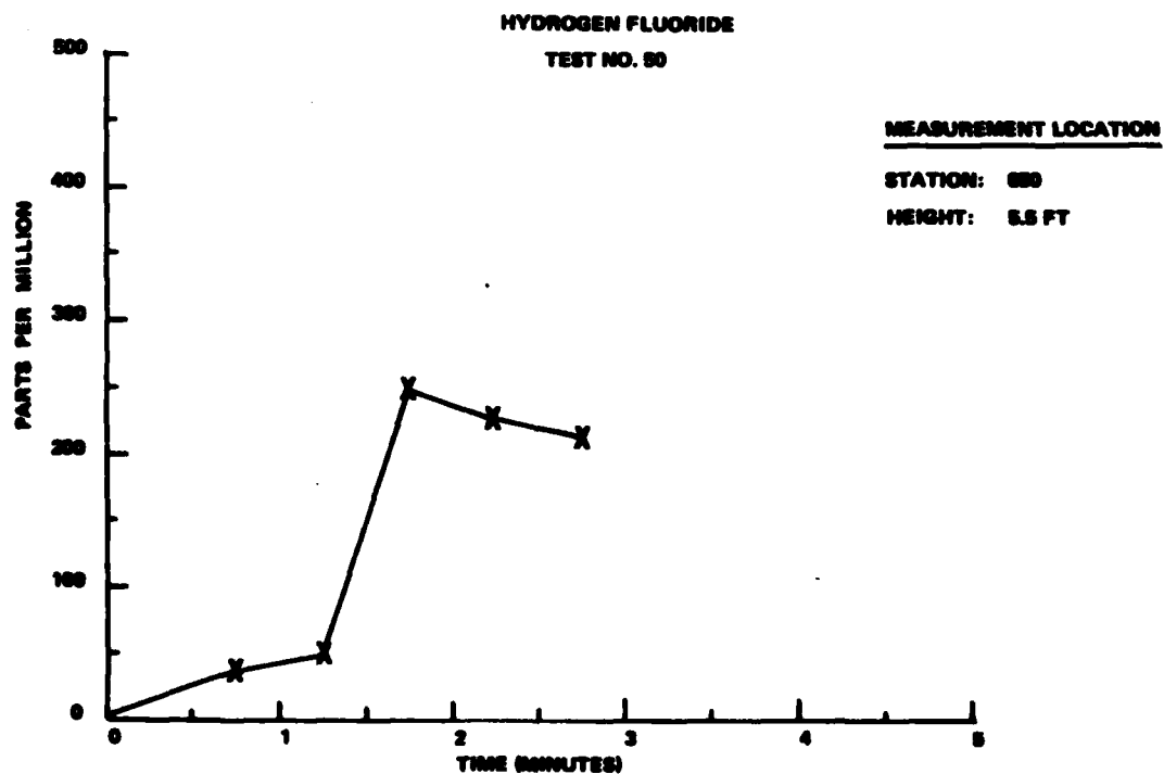
FIGURE 53. FULL-SCALE IN-FLIGHT ACID GAS MEASUREMENTS
