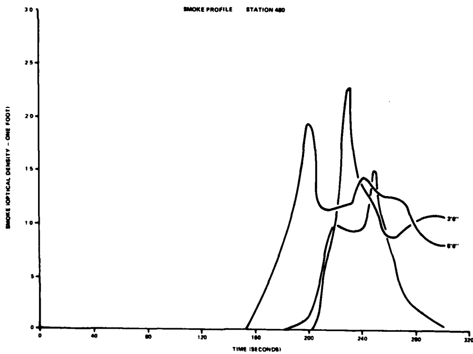
FIGURE C-4. SMOKE PROFILE STATION 480 (1 of 2 Sheets)
