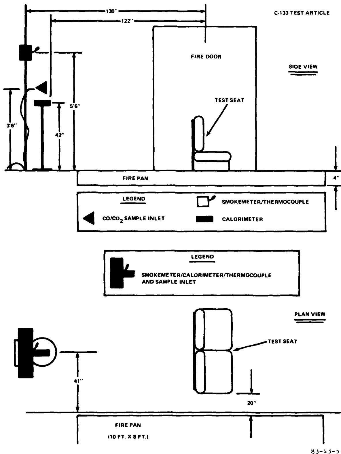
FIGURE 5. POST-CRASH SERIES ONE CONFIGURATION
