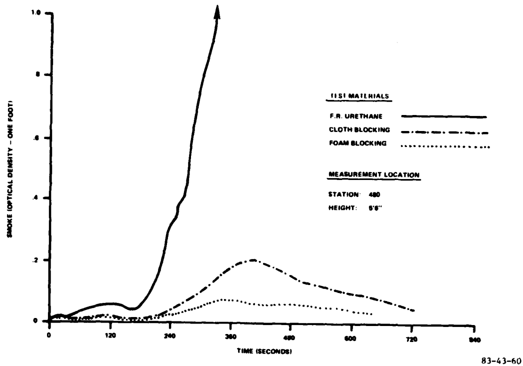
FIGURE 60. FULL-SCALE IN-FLIGHT BLOCKING LAYER COMPARISON (SMOKE)
