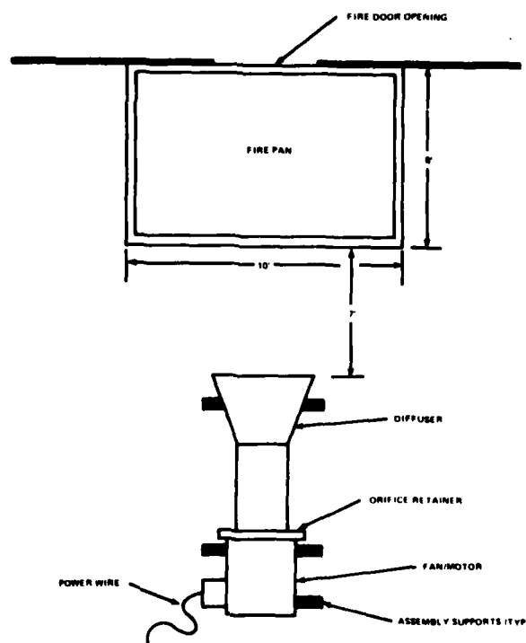
FIGURE 1. SCHEMATIC OF C133 WIDE-BODY CABIN FIRE TEST ARTICLE
