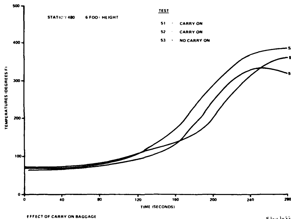
FIGURE 44. EFFECT OF CARRY-ON BAGGAGE
