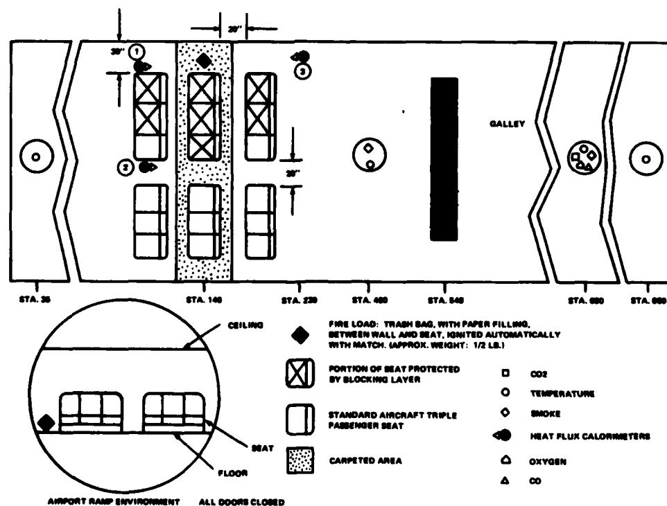
FIGURE 63. FULL-SCALE RAMP FIRE CONFIGURATION
