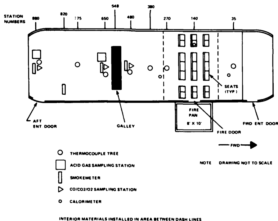
FIGURE 29. INSTALLATION OF WIDE-BODY MATERIALS INSIDE C-133 TEST ARTICLE
