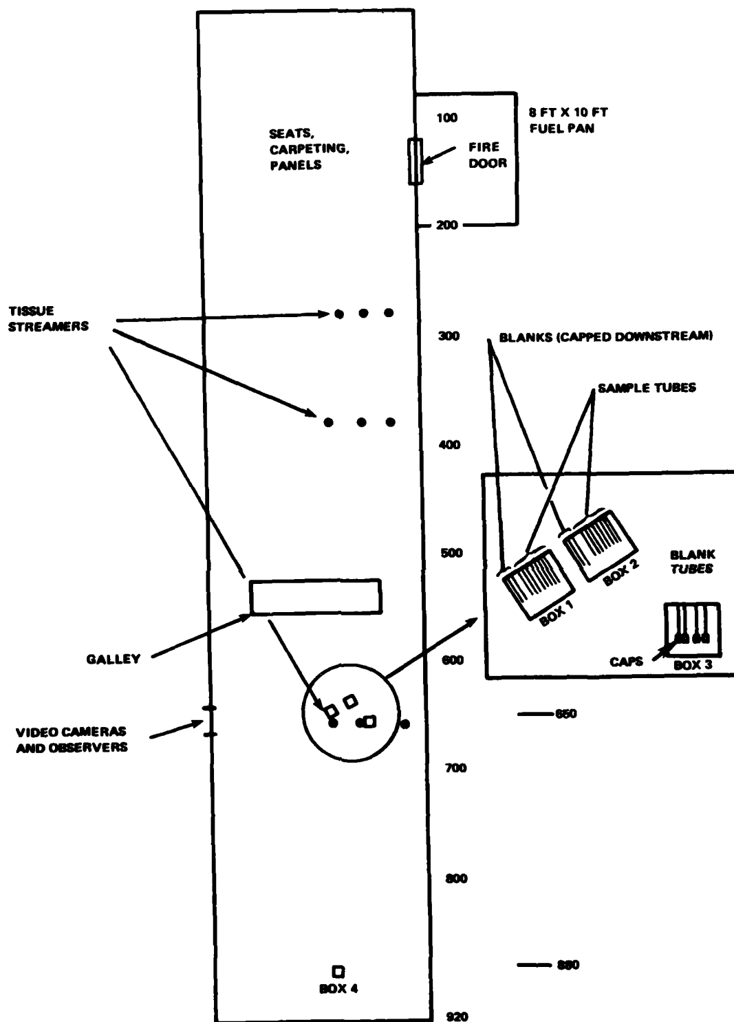
FIGURE B-9. POSITION DIAGRAM FOR ACID GAS SAMPLING STATIONS FOR C133 TEST 64
