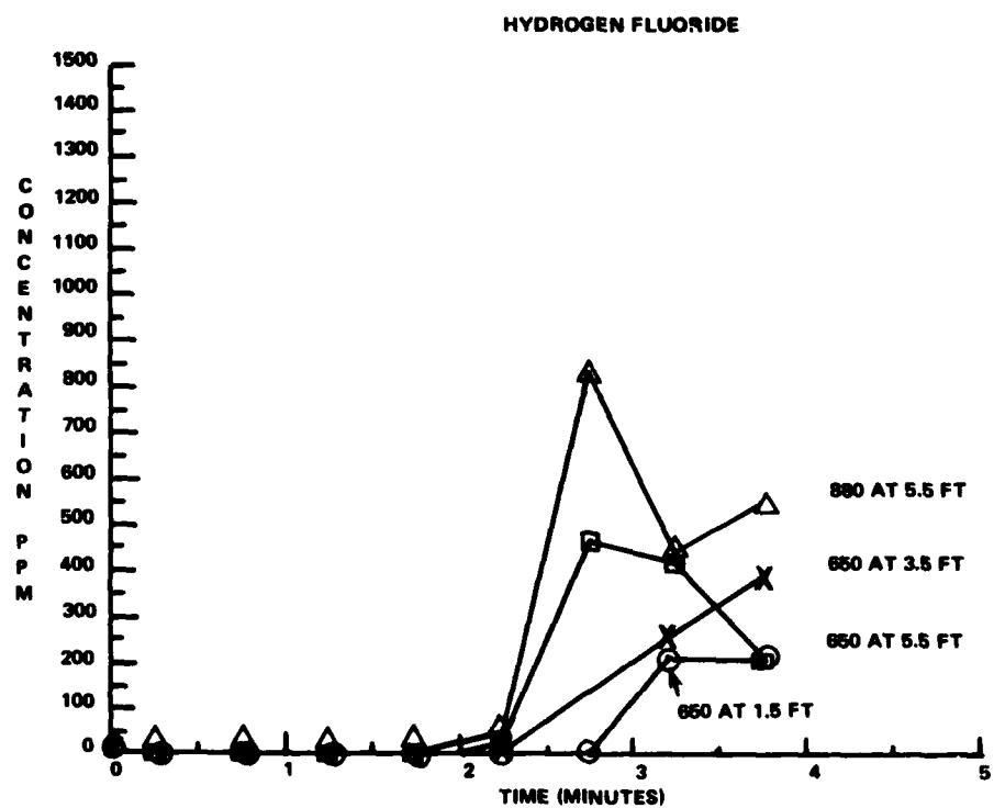
FIGURE B-5. EFFECT OF POSITION ON HF AND HCl LEVELS IN POST-CRASH FIRES: TEST 62
