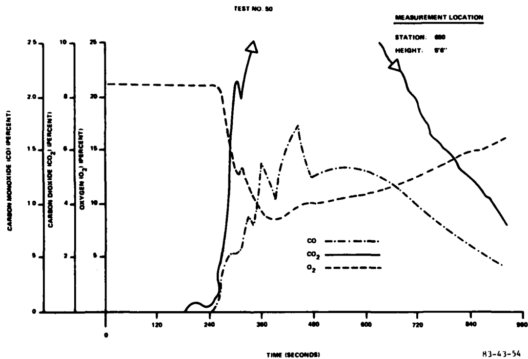
FIGURE 55. FULL-SCALE IN-FLIGHT SMOKE MEASUREMENTS
