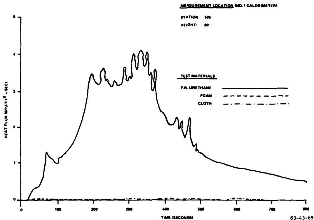
FIGURE 69. RAMP FIRE BLOCKING LAYER HEAT FLUX COMPARISON
