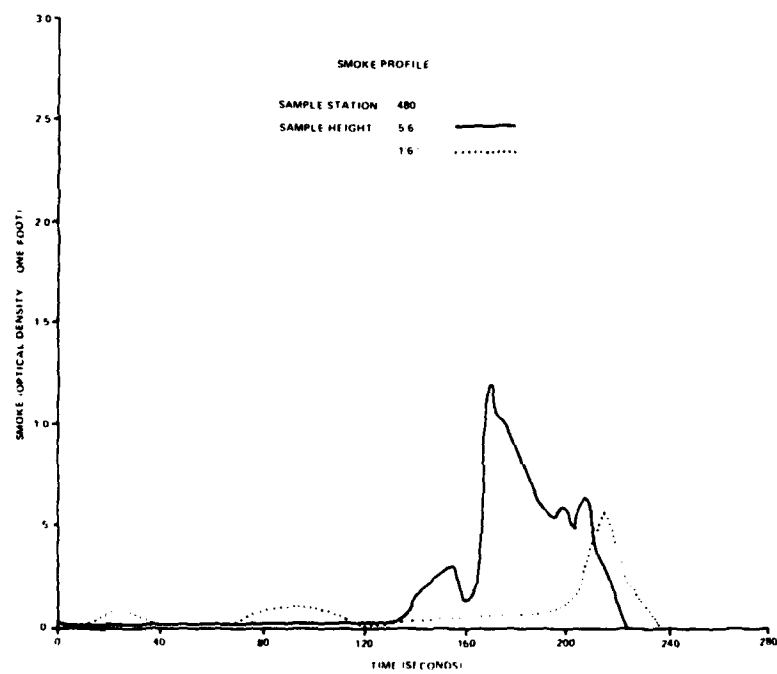
FIGURE C-4. SMOKE PROFILE STATION 480 (2 of 2 Sheets)
