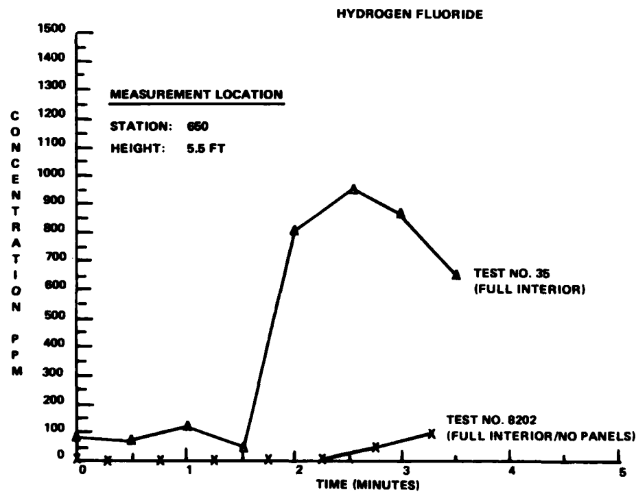
FIGURE B-7. EFFECT OF REMOVING PANELS ON HF AND HCl LEVELS IN POST-CRASH FIRES
