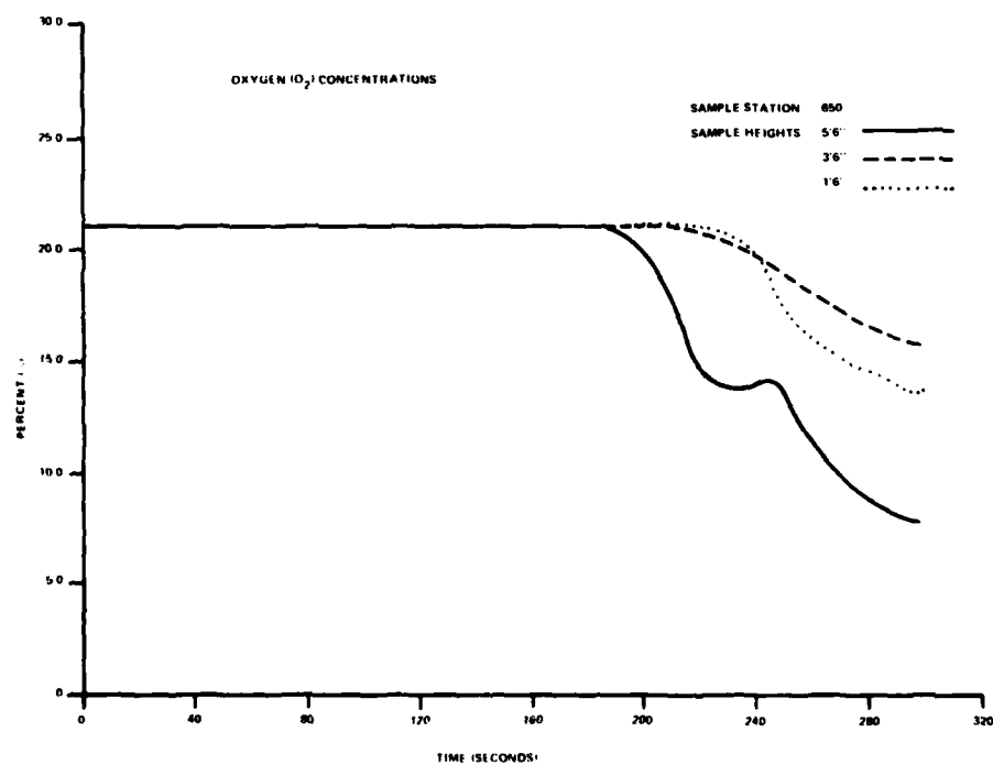
FIGURE C-9. O_2 PROFILE STATION 650 (1 of 2 Sheets)
