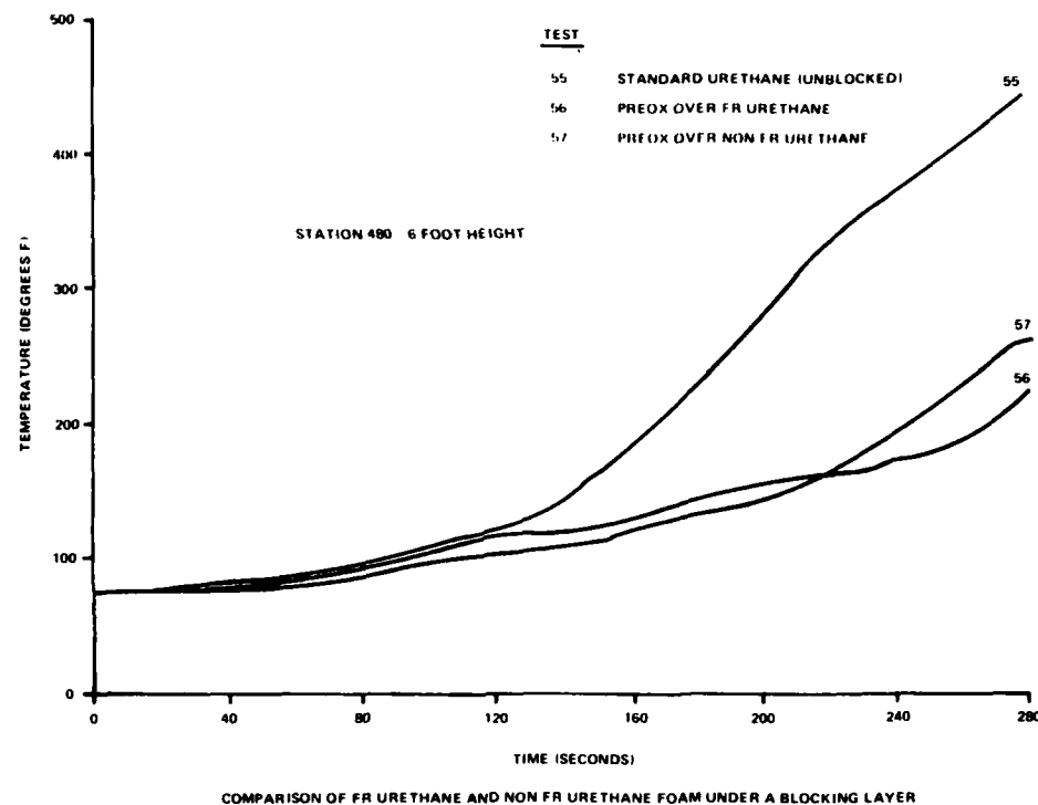
FIGURE 43. COMPARISON OF FR URETHANE AND NON-FR URETHANE FOAM UNDER A BLOCKING LAYER
