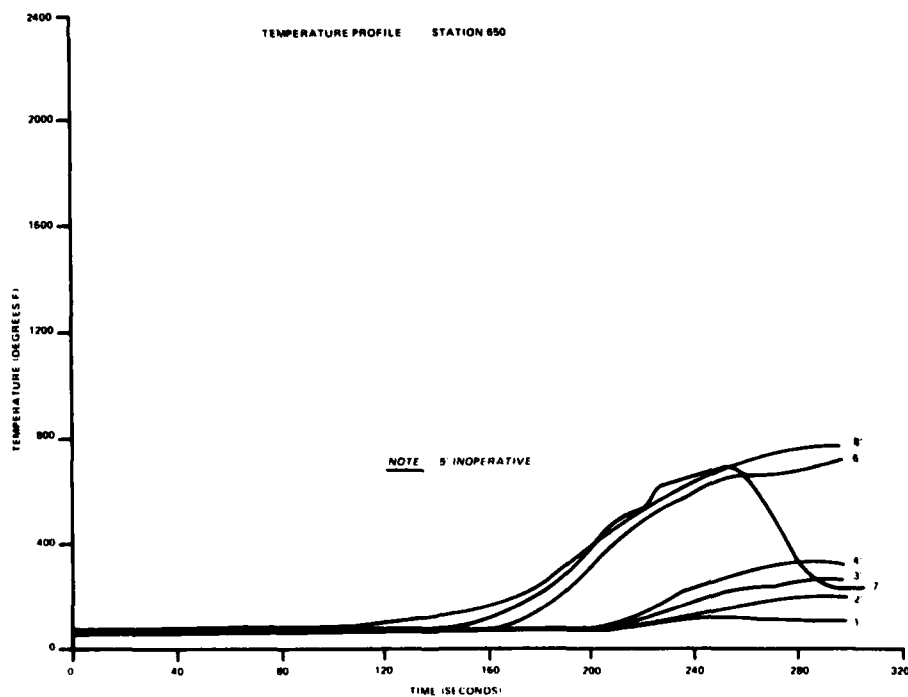
FIGURE C-3. TEMPERATURE PROFILE STATION 650 (1 of 2 Sheets)
