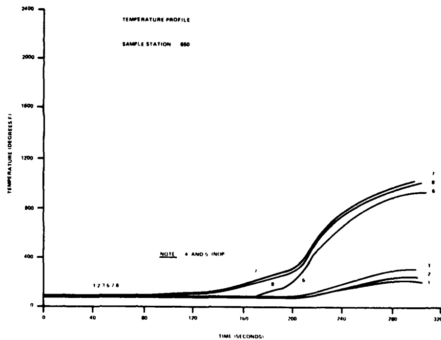
FIGURE C-3. TEMPERATURE PROFILE STATION 650 (2 of 2 Sheets)
