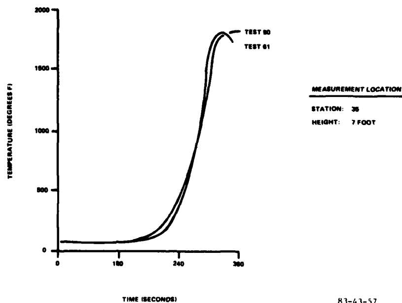
FIGURE 57. FULL-SCALE IN-FLIGHT TEMPERATURE COMPARISONS, STATION 35
