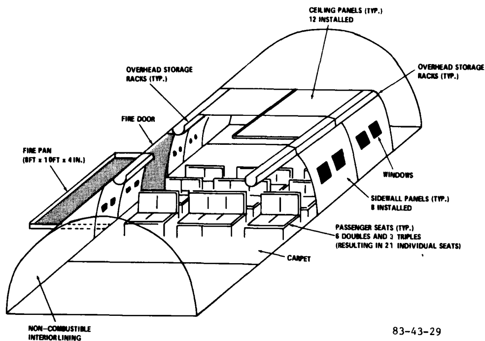
FIGURE 29. INSTALLATION OF WIDE-BODY MATERIALS INSIDE C-133 TEST ARTICLE
