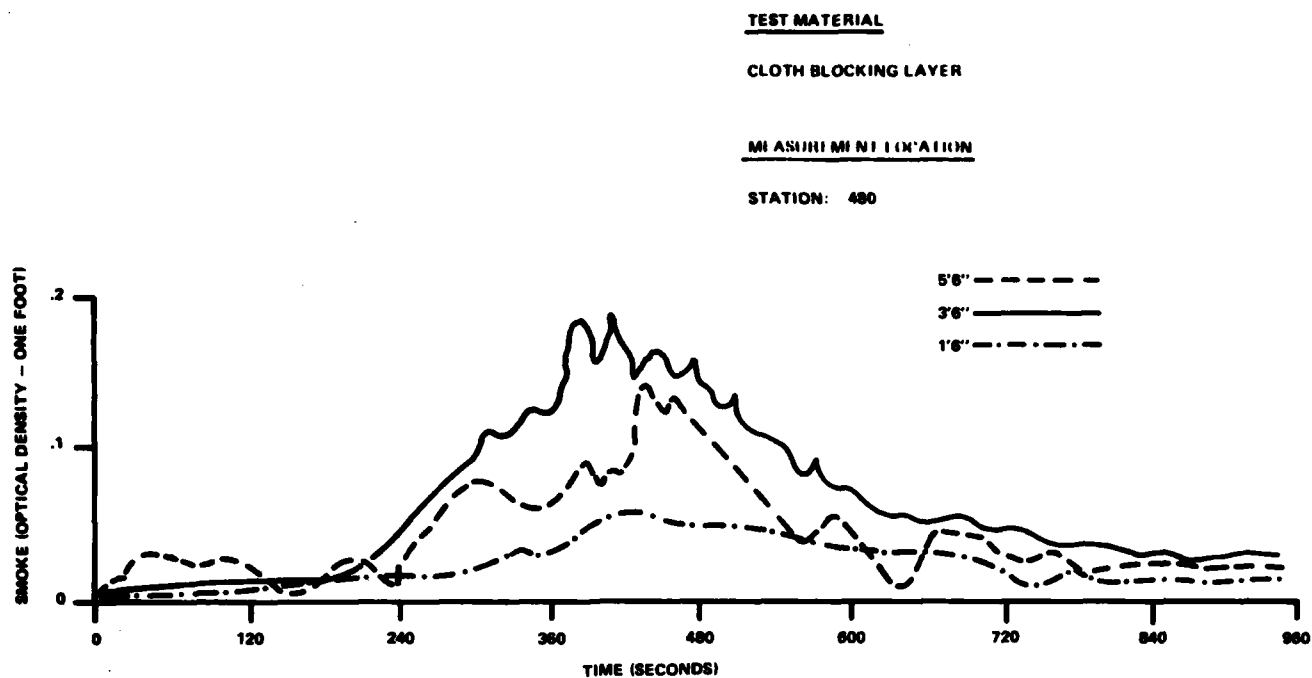
FIGURE 62. SMOKE STRATIFICATION PROFILE
