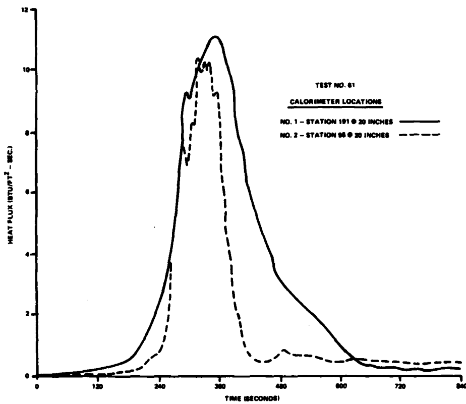
FIGURE 51. FULL-SCALE IN-FLIGHT HEAT FLUX
