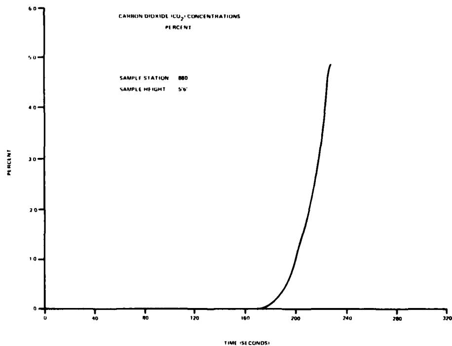
FIGURE C-6. CO 2 PROFILE STATION 880 (1 of 2 Sheets)
