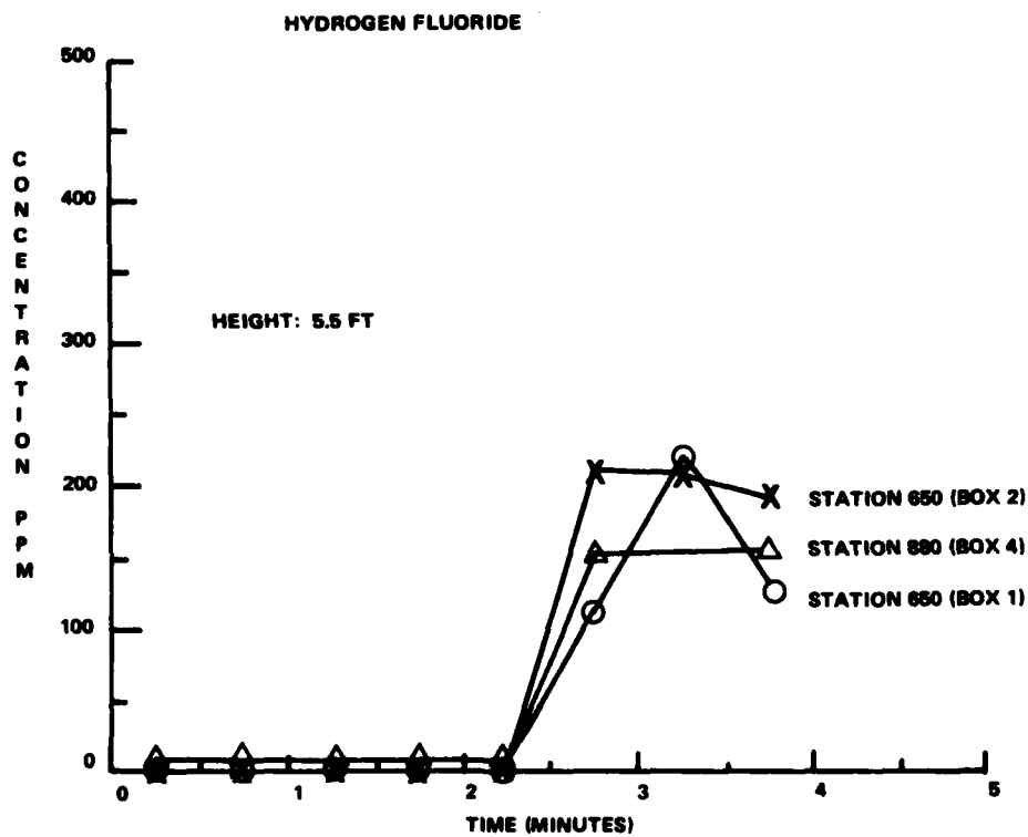
FIGURE B-10. CONCENTRATION — TIME PROFILES FOR C133 TEST 64
