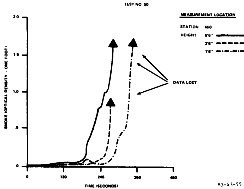
FIGURE 54. FULL-SCALE IN-FLIGHT GAS MEASUREMENTS
