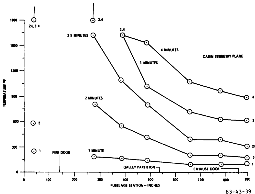
FIGURE 39. LONGITUDINAL TEMPERATURE PROFILE AT CEILING
