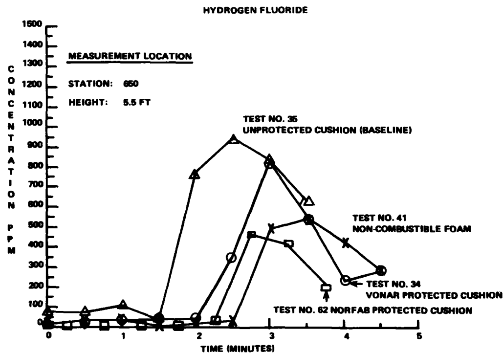
FIGURE B-6. EFFECT OF CUSHIONING PROTECTION AND MATERIALS ON HF AND HCl LEVELS IN POST-CRASH FIRES
