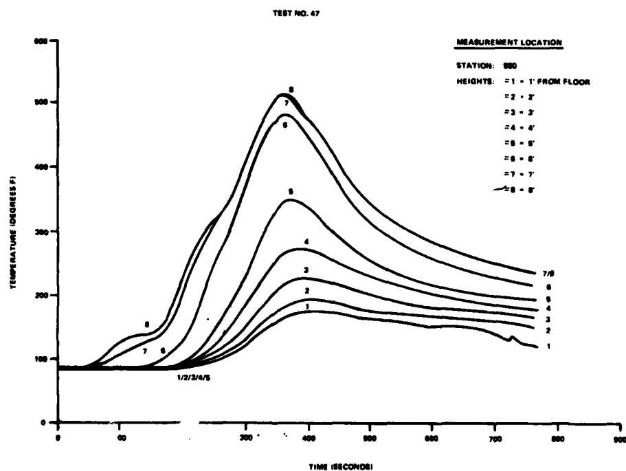
FIGURE 64. RAMP FIRE TEMPERATURE PROFILES (2 of 2 Sheets)
