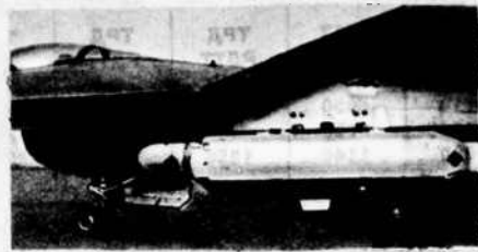
The AN/ALQ-131 Jamming Station in a suspended container on the F-16 Airplane.
