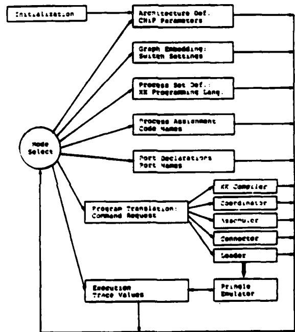
Figure 6. The logical structure of the Paker Environment.
