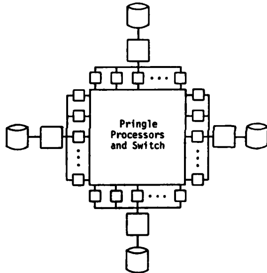
Figure 7. The logical structure of the external input/output system.
