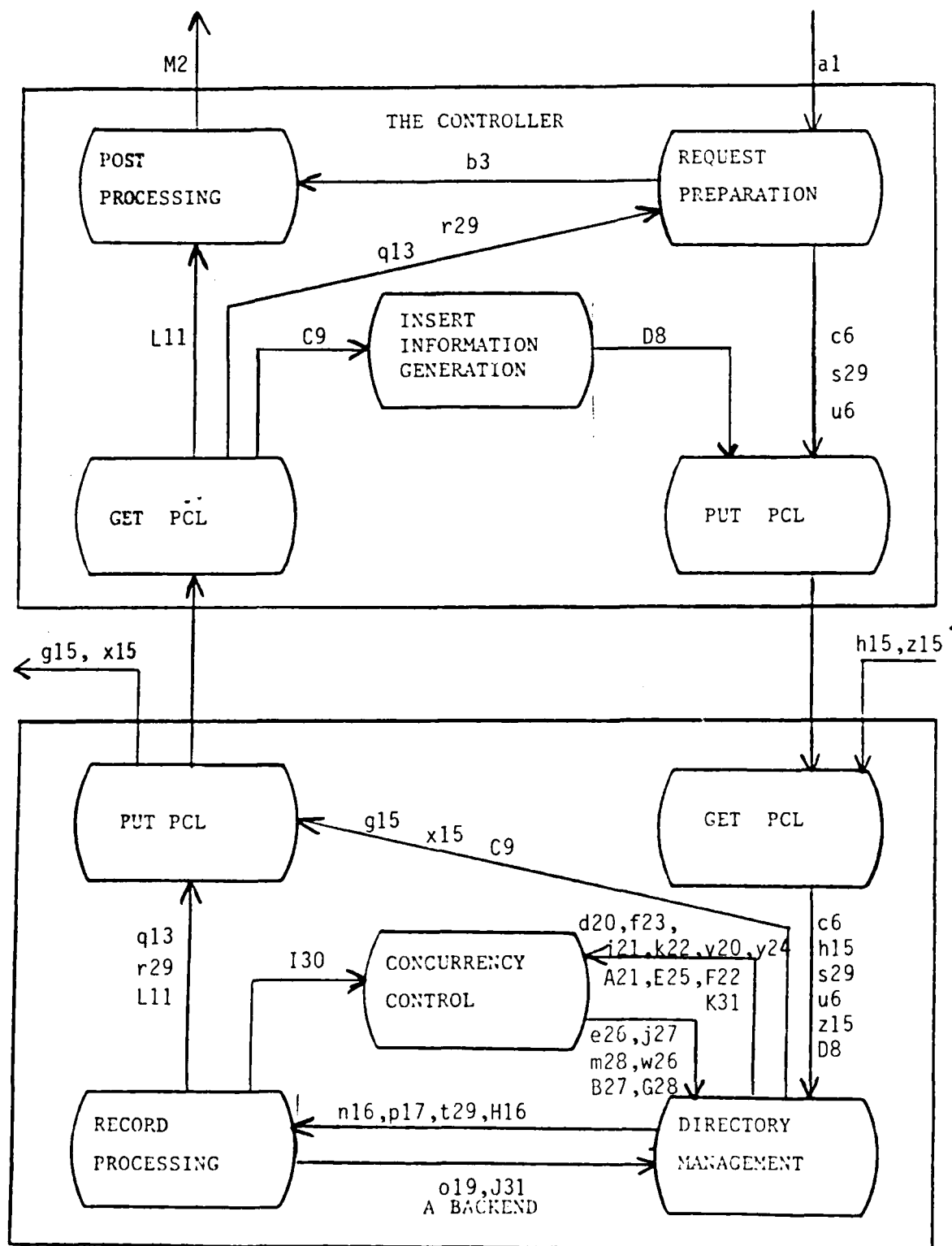
Figure 27. Sequence of Messages for an Update Request
