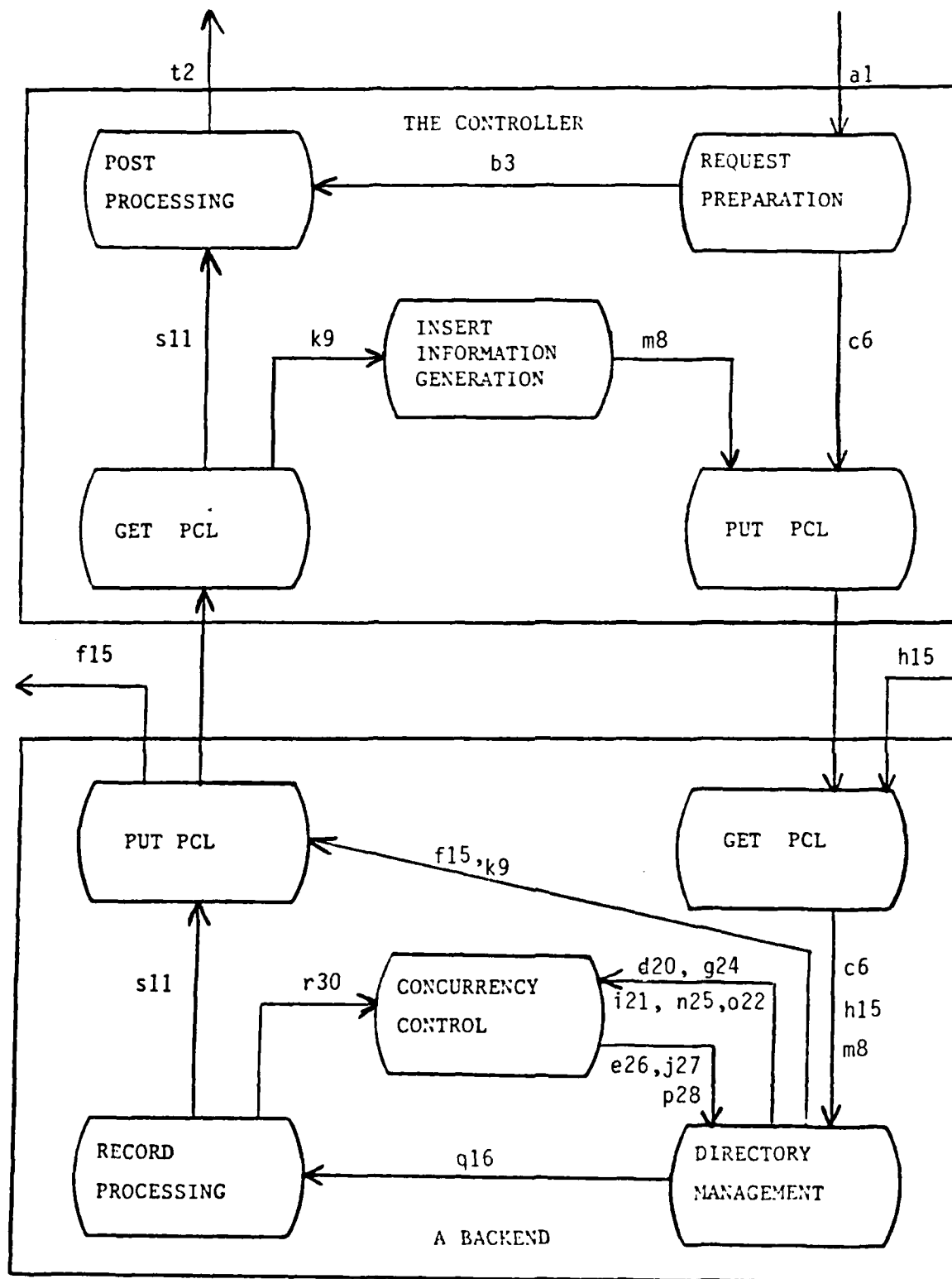
Figure 24. Sequence of Messages for an Insert Request
