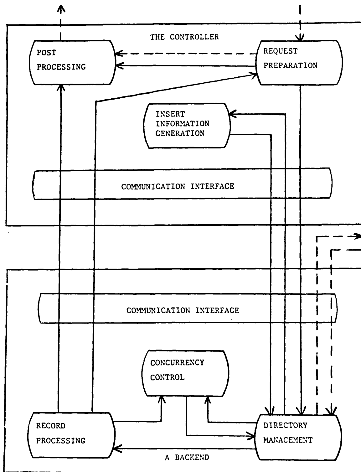
Figure 2. The MDBS Process Structure
