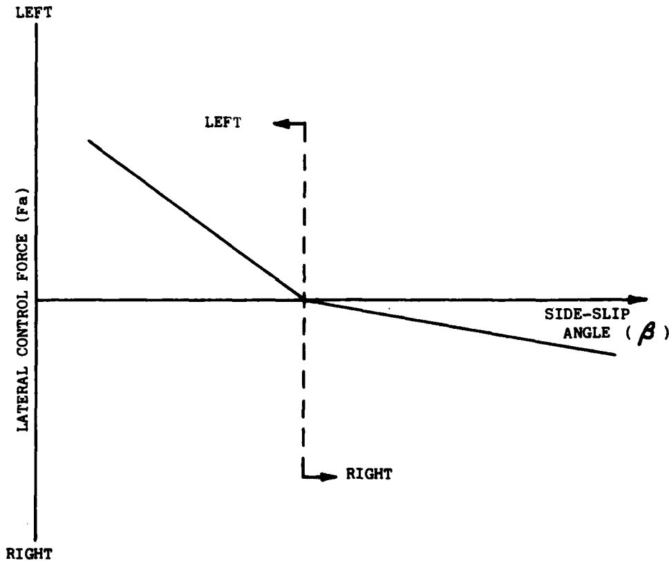
FIGURE 3 - LATERAL-DIRECTIONAL STATIC STABILITY - AILERON FORCE (LATERAL CONTROL FORCE) VARIATION WITH SIDE-SLIP ANGLE (APPARENT DIHEDRAL EFFECT ( C_{l\beta} ))
