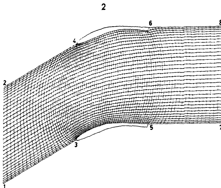
Fig. 1. Computational grid and boundary of the computational domain.
