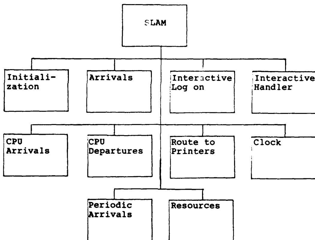
Figure 3.9 Discrete Structure.
