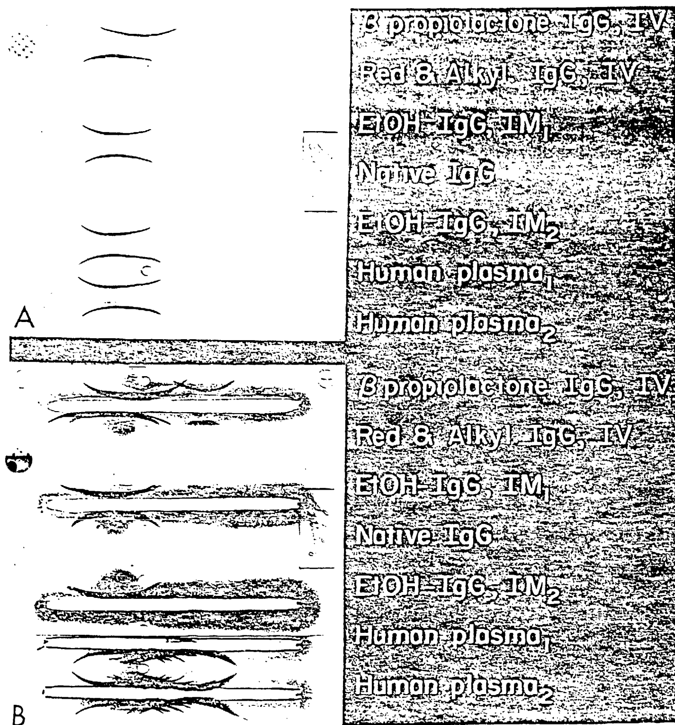
Figure 4. Immunoelectrophoresis of various immunoglobulin preparations. The electrodes and the preparations analyzed are indicated on the figure. Samples (40 mg protein/ml) were subjected to 150 V for 80 min and allowed to diffuse against antiserum for 24 h. Plates were washed for 48 h and stained with Amido Black. Plate A troughs contained anti-human IgG ( \gamma -chain specific); plate B, anti-whole human serum.
