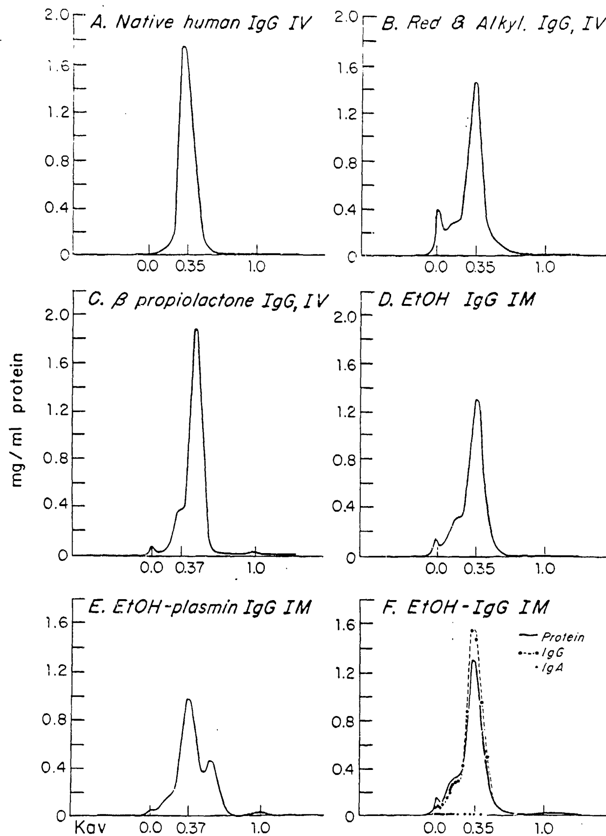
Figure 2. Measurement of aggregates and fragments of IgG by exclusion chromatography. Elution pattern shows the chromatographic behavior of various immunoglobulin preparations on a column of Biogel A-1.5m. Abscissa shows K_{av} .
