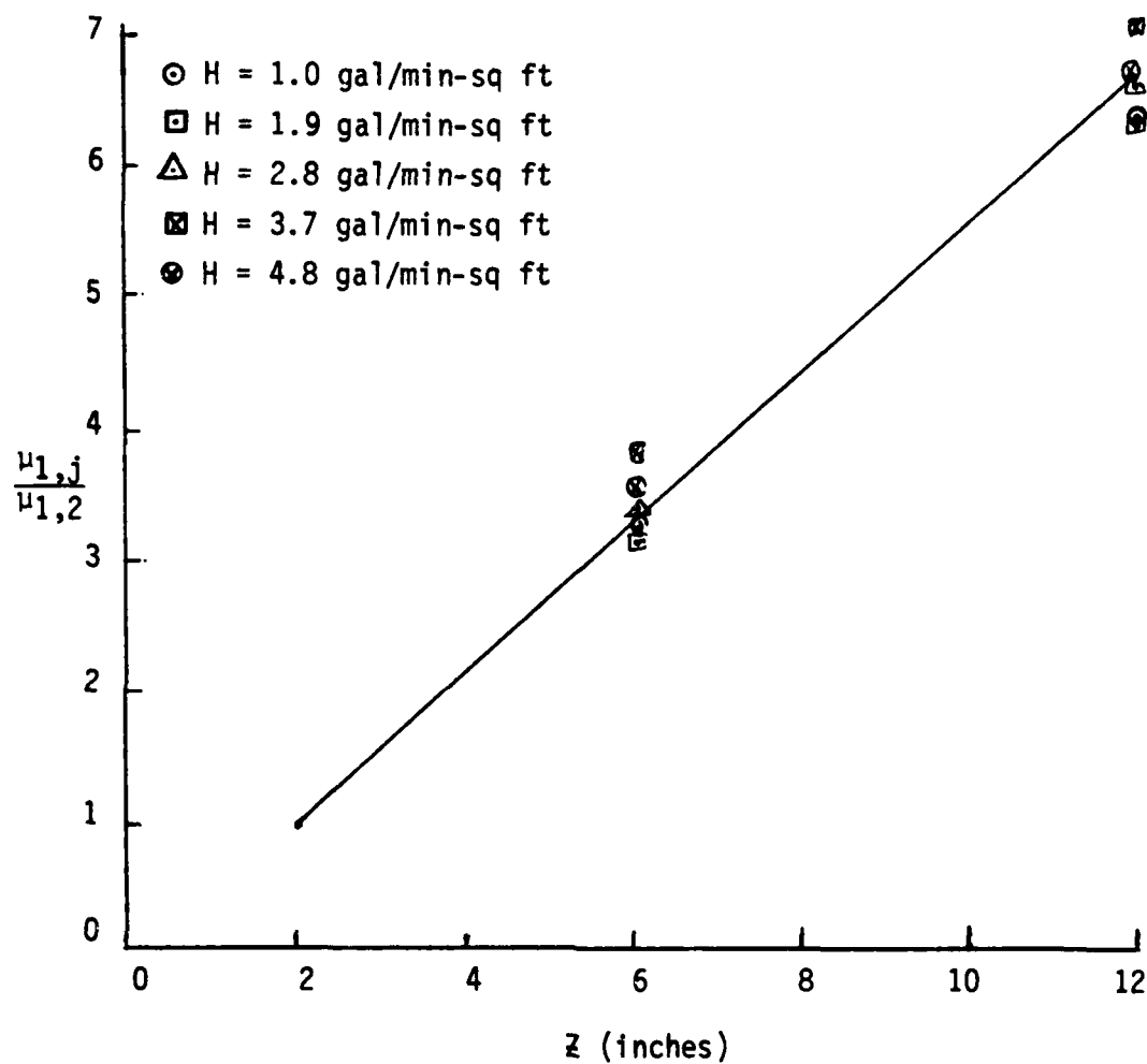
Figure 13. Effect of column length and hydraulic loading on the dimensionless ratio \mu_{1,j}/\mu_{1,2} for 300 ppm MIK at 271.2 nm.
