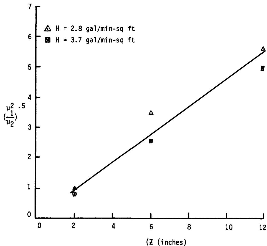
Figure 23. Effect of column length and hydraulic loading on the dimensionless ratio (\mu_{1,j}^2 / \mu_{2,2})^{.5} for 300 ppm chloroform at 211 nm.
