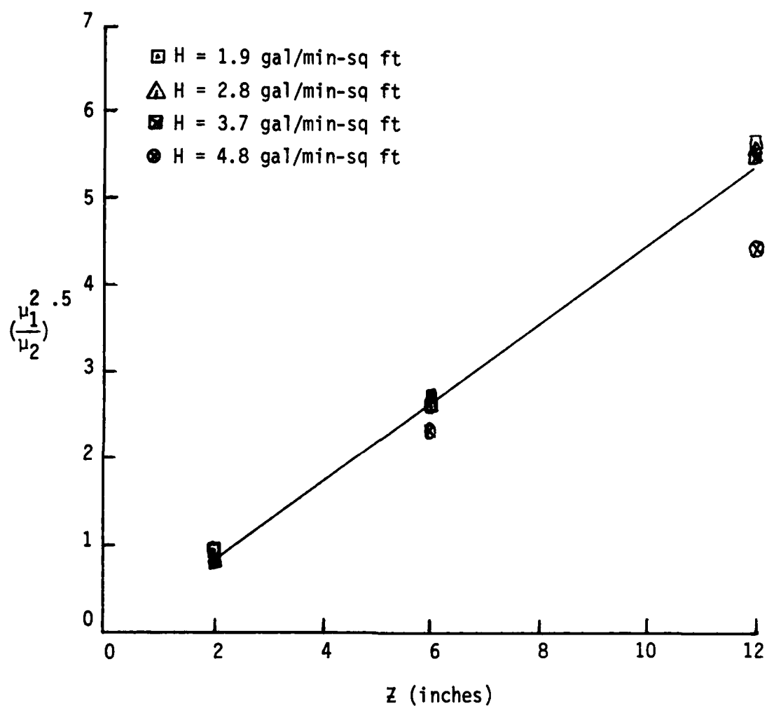
Figure 22. Effect of column length and hydraulic loading on the dimensionless ratio (\mu_{1,j}^2/\mu_{2,2})^{0.5} for binary solution of 300 ppm MIK and 300 ppm chloroform at 271.2 nm.
