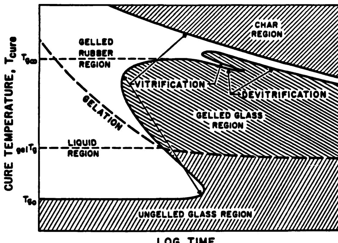
FIGURE 1 Isothermal time-temperature-transformation (TTT) diagram of a thermosetting polymer showing three critical temperatures ( T_{g\infty} , gelT_g , and T_{g0} ) and four distinct states of matter (liquid, gelled rubber, gelled glass, and ungelled glass) that pertain to cure. T_{g\infty} is the maximum glass transition temperature of the cured material; gelT_g is the temperature at which the times to gelation and to vitrification are equal; T_{g0} is the glass transition temperature of the reactants. At high temperatures thermal degradation can lead to vitrification and devitrification, depending on whether the glass transition temperature increases from the rubbery to the glassy state or decreases from the glassy to the rubbery state.
