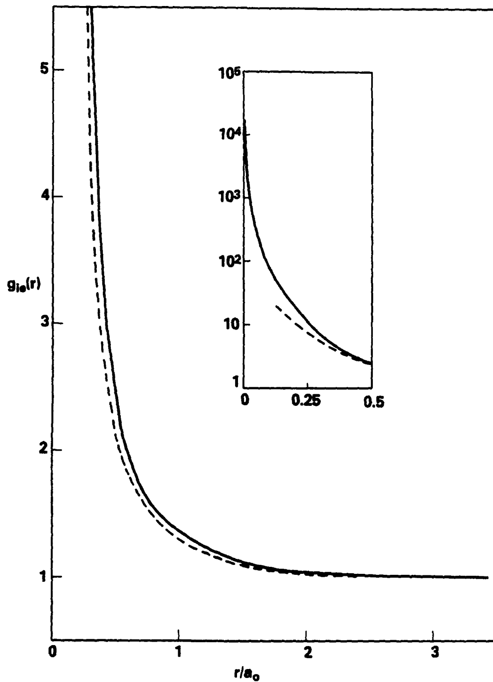
Fig. 2. Electron distribution around an ion for \Gamma = 2.2 . Solid line is the DF model; dashed is the HNC approximation. The smallest radius used in the Fourier transform within the HNC scheme was r/a_0 = 0.125 .
