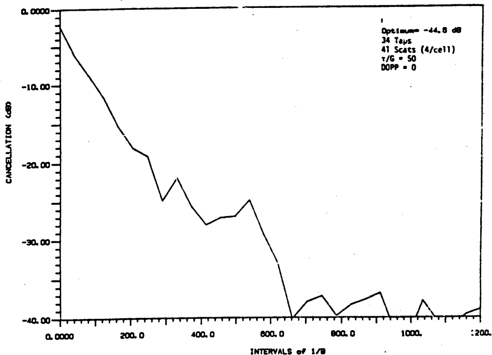
Fig. 10 -- Scatter Canceller - 34 Taps, 10 Cells Contain Scatterers
