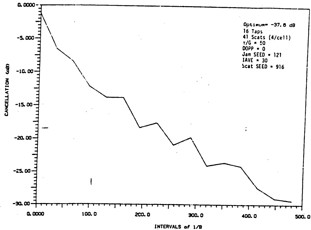
Fig. 5 -- Scatterer Celler - Effect of Random Scatterer Coefficients (Compare Fig. 4)
