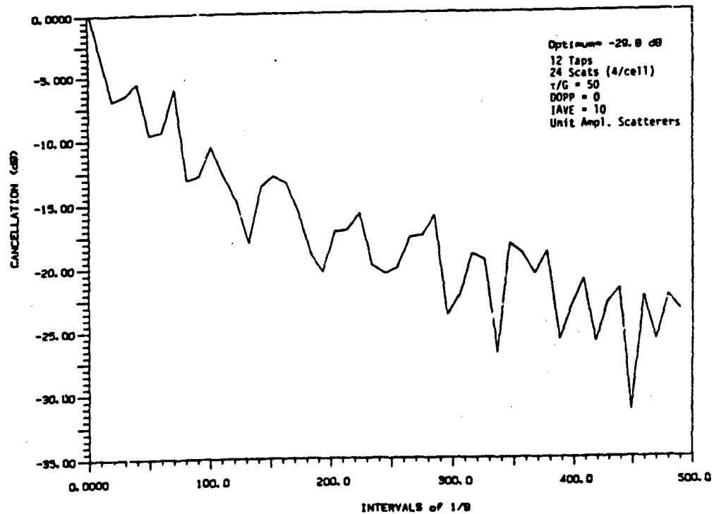
Fig. 16 -- Simulation of Scatter Canceller with Unit Amplitude Scatterers (4/cell)
