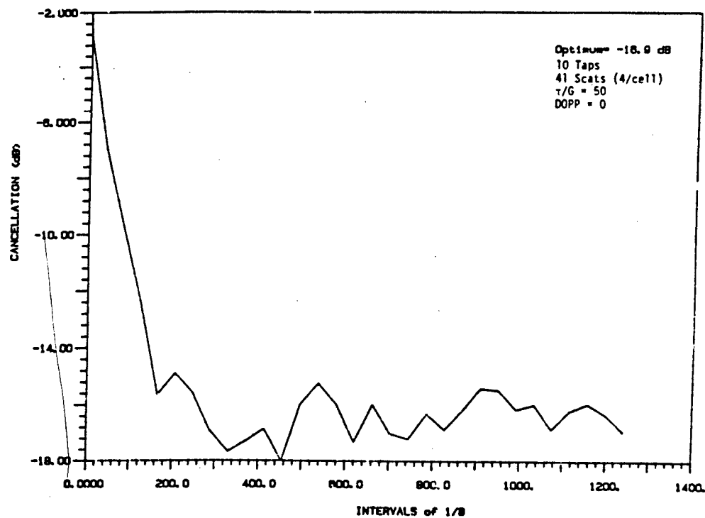
Fig. 6 -- Scatterer Celler - 10 Taps, 10 Cells Contain Scatterers
