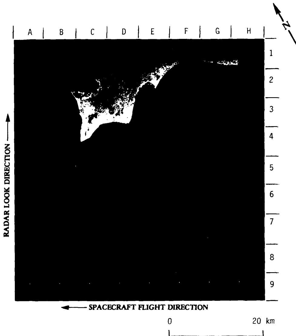
Figure 15. SIR-A SAR Imagery of Mayaguana, Bahamas (Data Take 24 BB, 13 November 1981, Optically Processed Imagery Courtesy of NASA)
