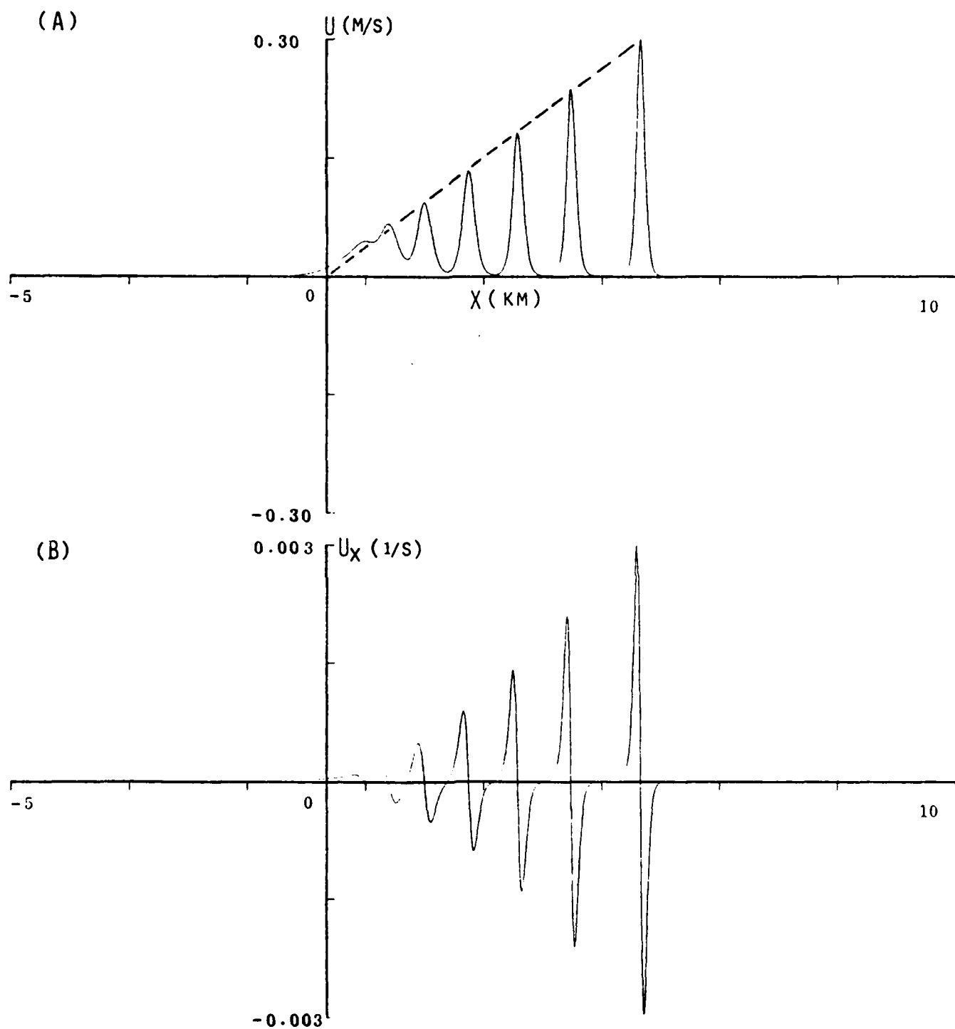
Figure 7. (a) Surface Current, and (b) Strain Rate Induced by an Internal Wave Packet.
