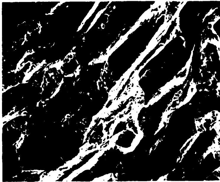
Figure 24. Zone of cleavage fracture suggesting hydrogen damage. ( 540X)
