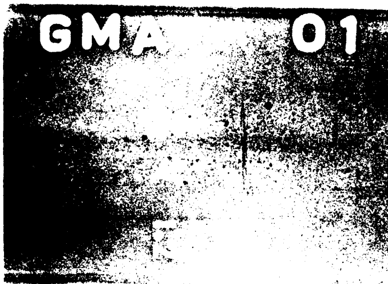
Figure 21. Portion of a xeroradiograph showing hydrogen induced cracking and porosity in a Gas Metal Arc weld (GMA-01)
