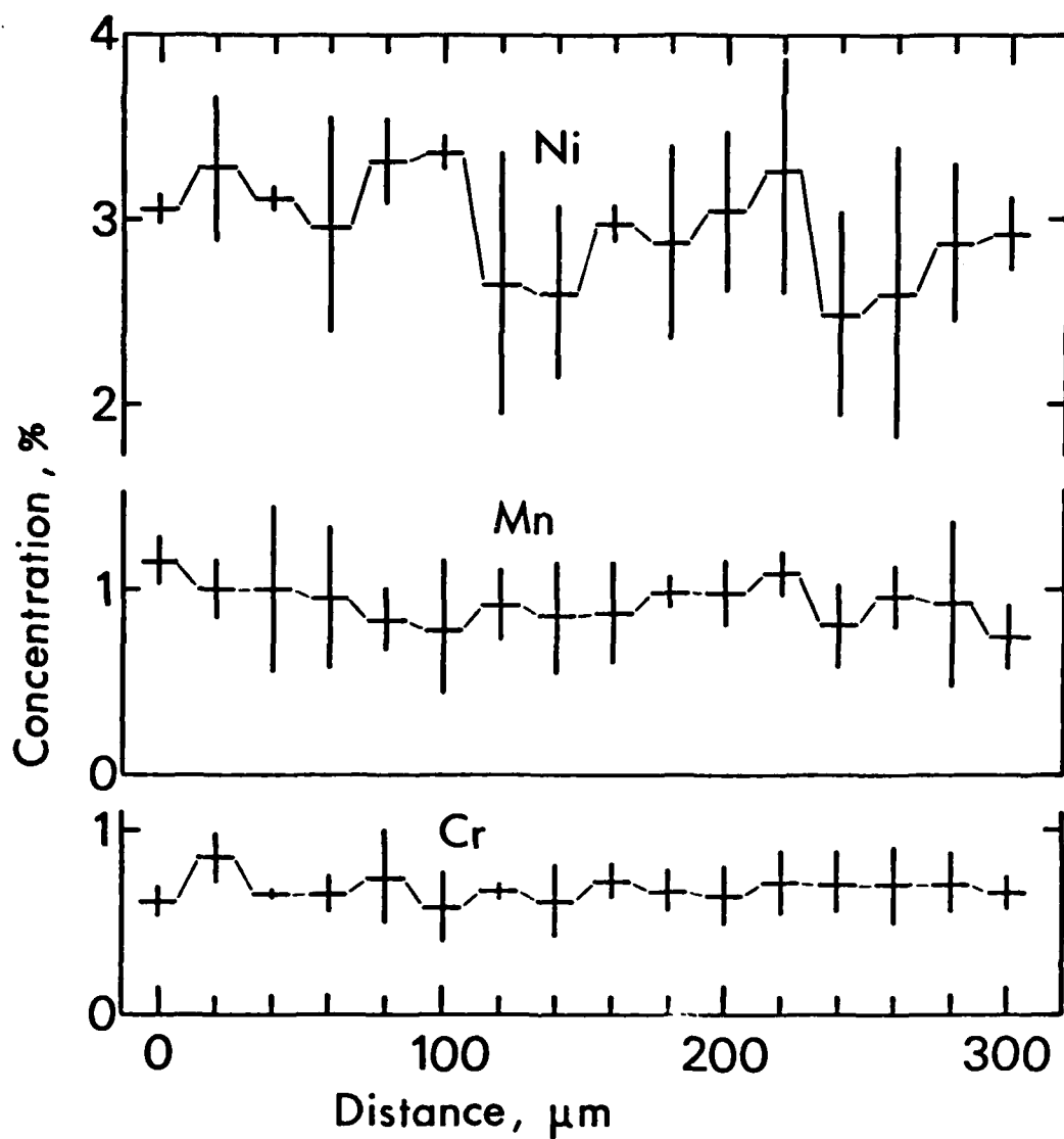
Figure 49. Microprobe traverse across light etching band in figure 50. Weld produced with ribbon type electrode. Bars are two sigma limits.
