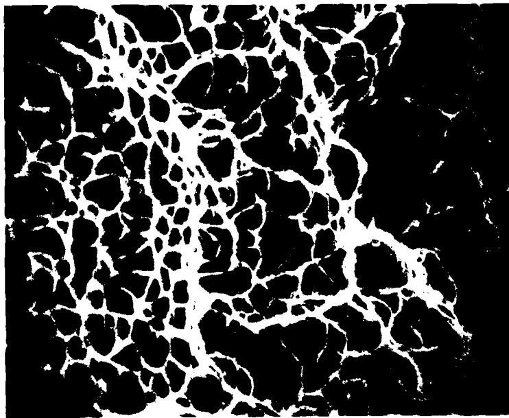
Figure 25. Ductile fracture zone. ( 2200X)
