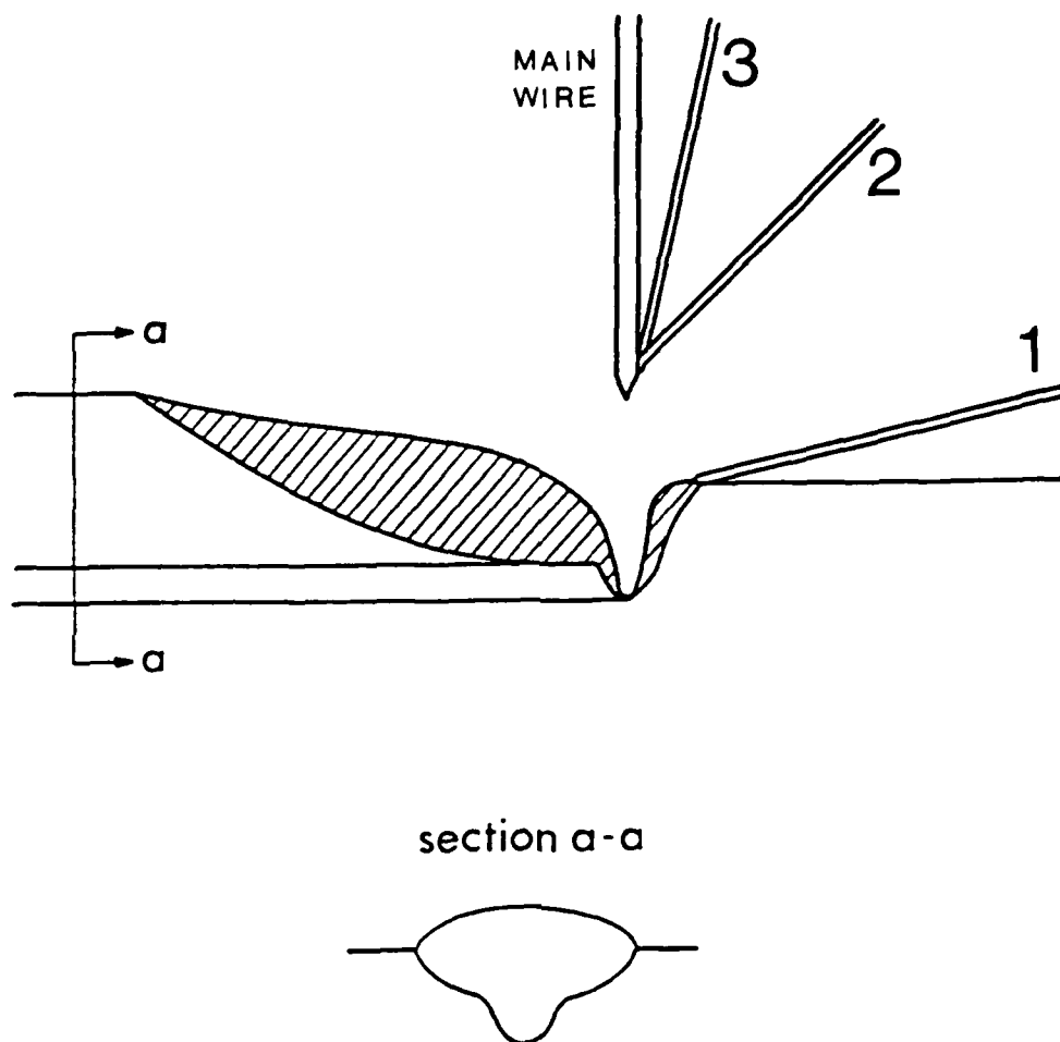
Figure 9. Schematic illustration of Gas Metal Arc secondary wire addition methods.
