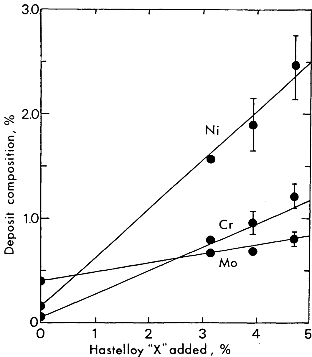
Figure 34. Results of weld metal chemical analysis from Gas Metal Arc, method 1, pad deposit. E80S-D2 primary wire with various additions of Hastelloy 'X'. Spectrographic analysis, compared with calculations. Bars indicate 2-sigma limits of 7 analyses at different points in the deposit. Scatter is evidently due to 2-cell mixing pattern.
