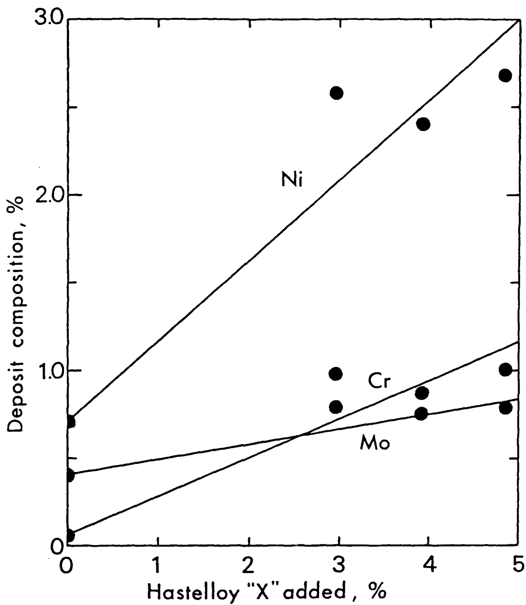
Figure 33. Results of weld metal chemical analysis from Gas Metal Arc, method 1, pad deposit. Linde 44 with various additions of Hastelloy 'X'. Spectrographic analysis compared with calculations.
