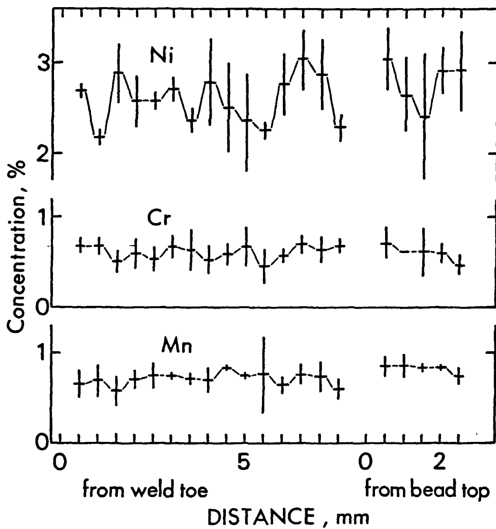
Figure 48. Results of microprobe surveys on ribbon type electrode deposit. Bars are 2-sigma limits.
