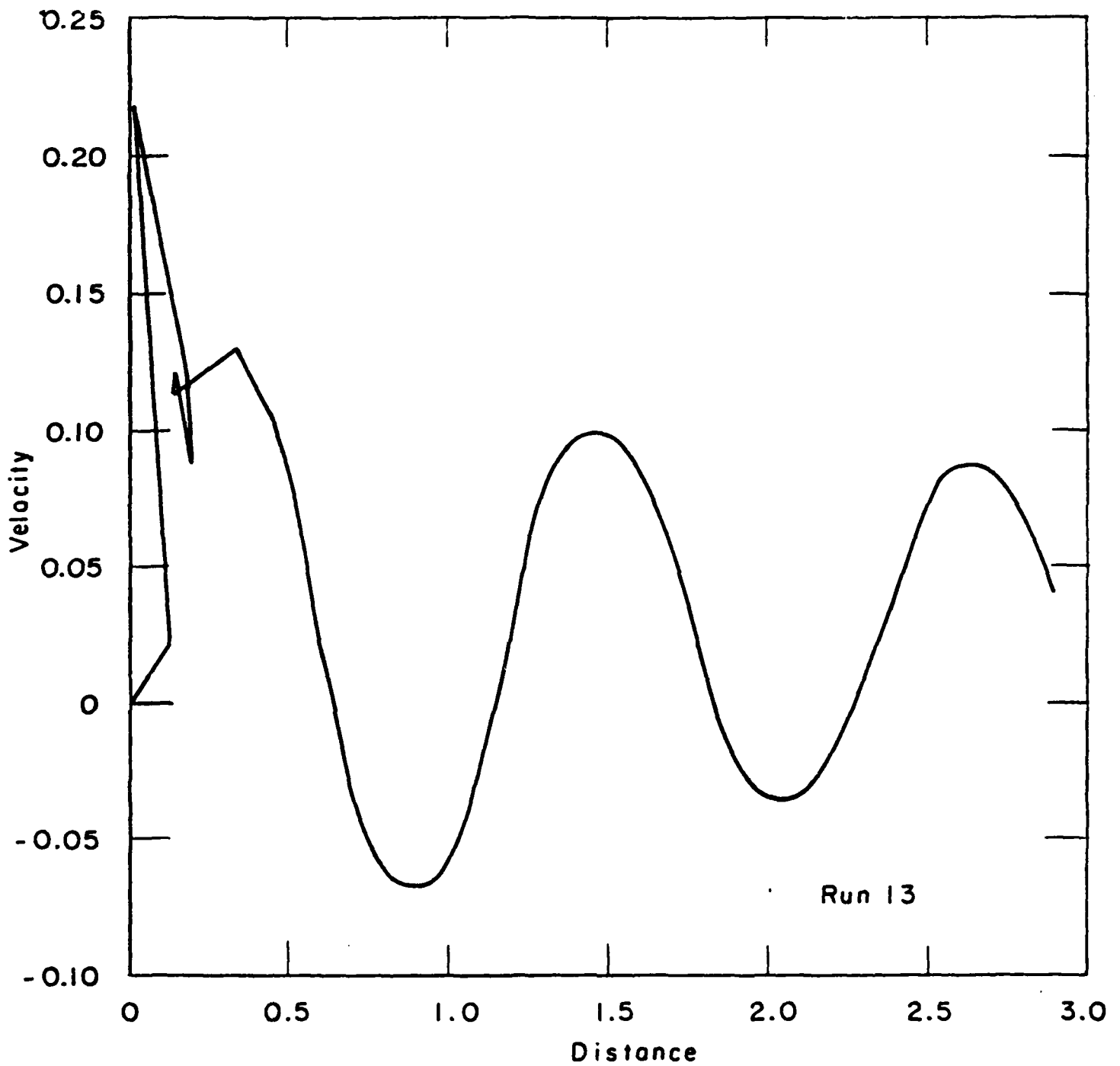
FIG. 15 LIAPUNOV STABILITY C_L = 2.33 , \delta = 0^\circ , YAW \approx 2^\circ
