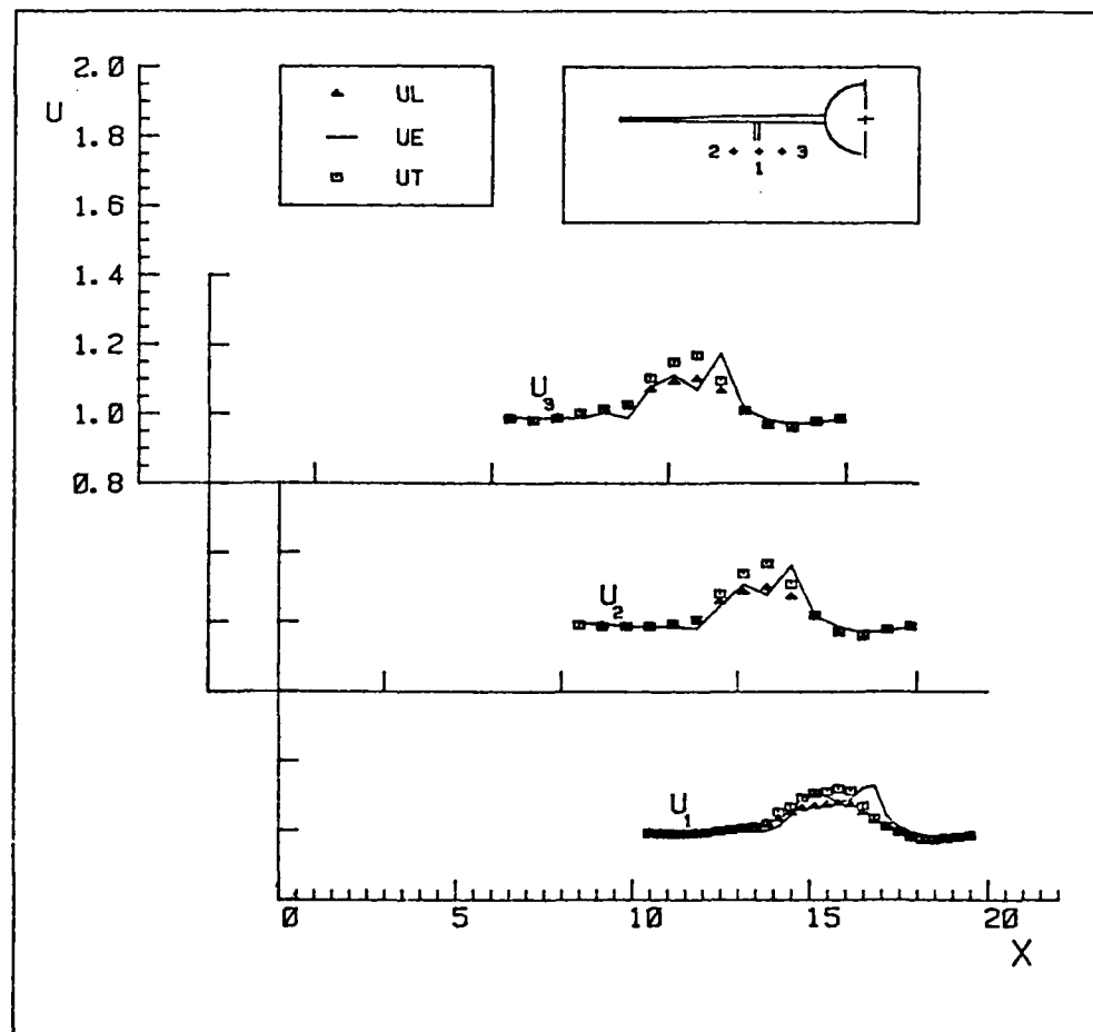
Figure 12. U VELOCITIES FOR M = 0.925 ; \alpha = 0^\circ
