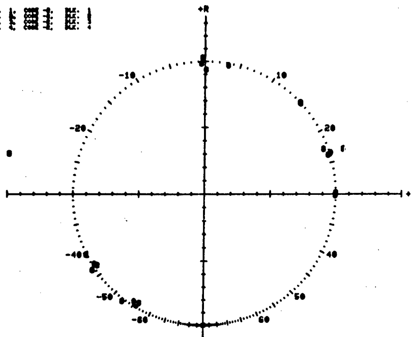
(a) Z-plane roots
