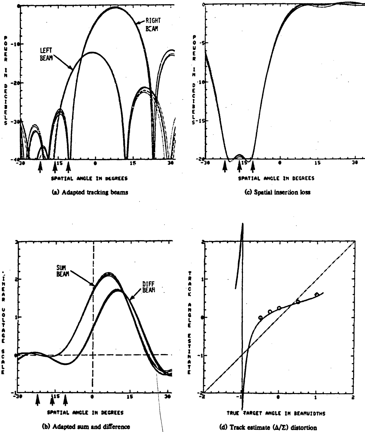
Fig. 16 — Adaptive processing spatial filter functions related to tracking angle estimation for Case C8L3J3C-I
