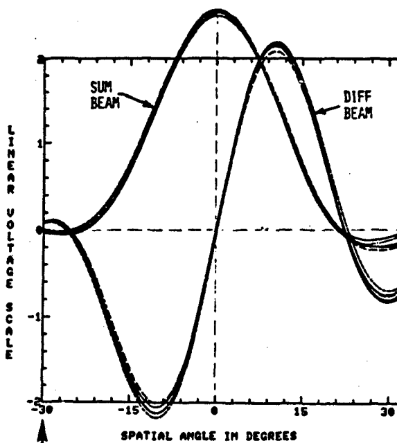
(b) Adapted sum and difference
