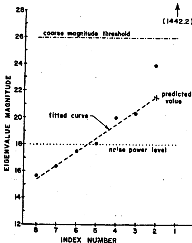
Fig. 22 — Plot of eigenvalues vs eigenvalue index for Case C8L1J1TφG
