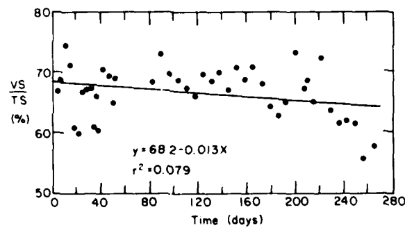
Figure 18. Ratio of volatile to total solids over time for the Palmer lagoon.
