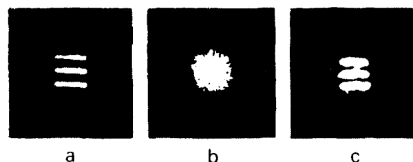
Figure 3-1. Demonstration of image transmission through a fiber. (a) Image of Air Force resolution chart at input end of fiber. (b) Output after a single pass through the fiber. (c) Reconstruction of resolution chart after output has been phase conjugated and retraverses fiber.
