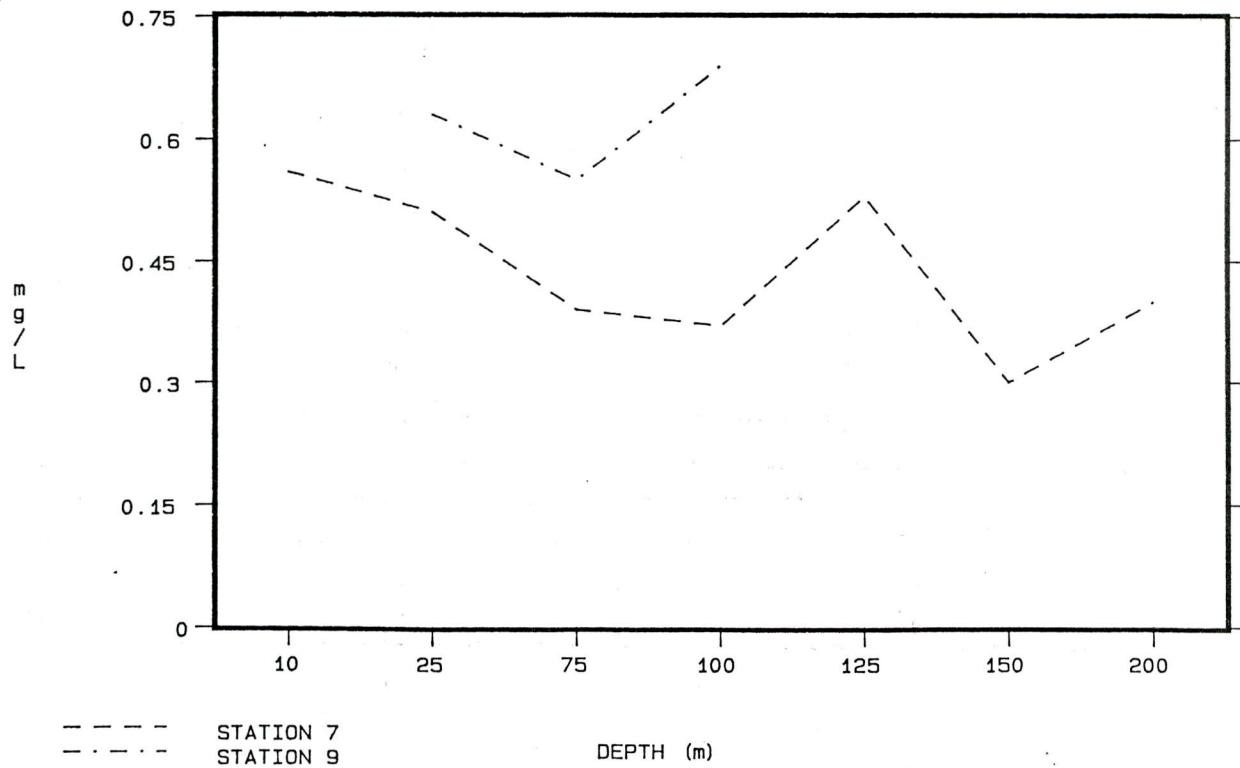
Figure 17. Dissolved organic carbon concentrations as a function of depth in Exuma Sound (top) and in the Straits of Florida (bottom).
