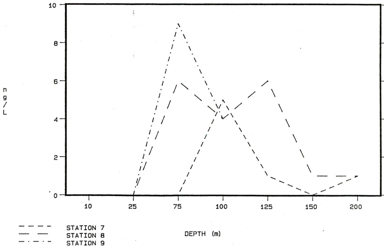
Figure 14. Phaeophytin concentrations as a function of depth in Exuma Sound (top) and in the Straits of Florida (bottom).
