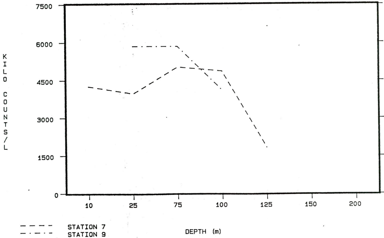
Figure 23. Small (1-10 \mu\text{m} diameter) particle counts from Exuma Sound (top) and the Straits of Florida (bottom).
