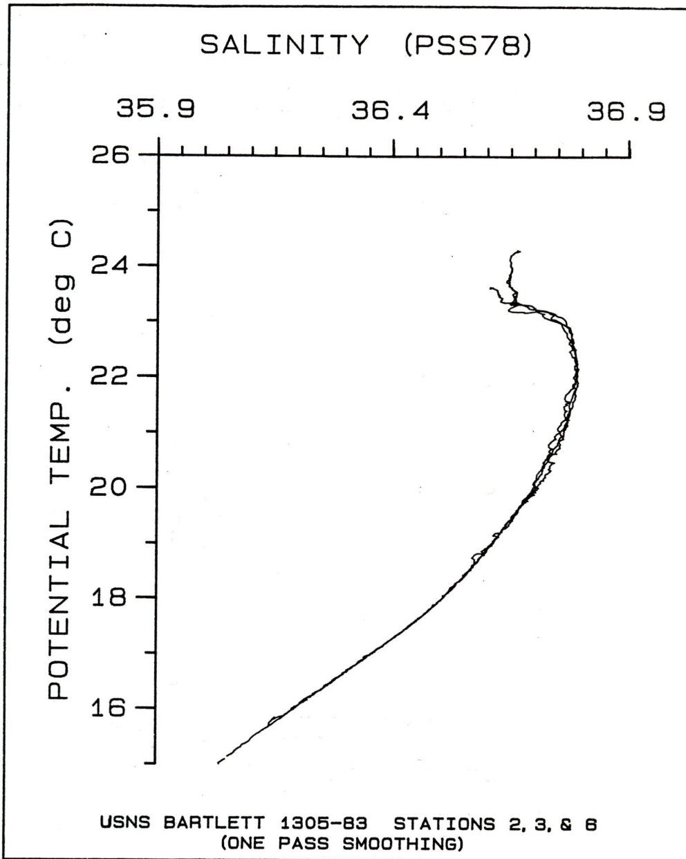
Figure 3. Plot of salinity vs. temperature at Stations 2, 3, and 6 in Exuma Sound.
