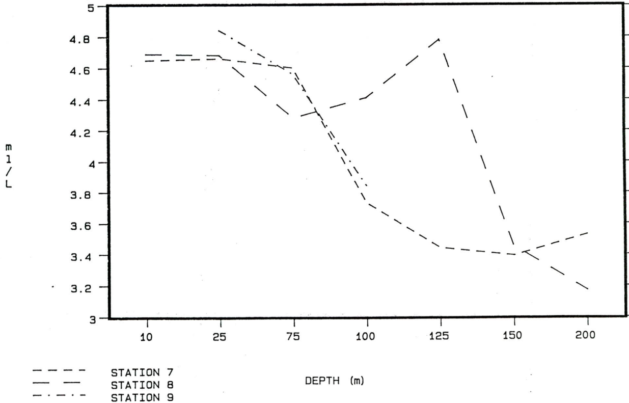
Figure 9. Oxygen concentration as a function of depth in Exuma Sound (top) and in the Straits of Florida (bottom).
