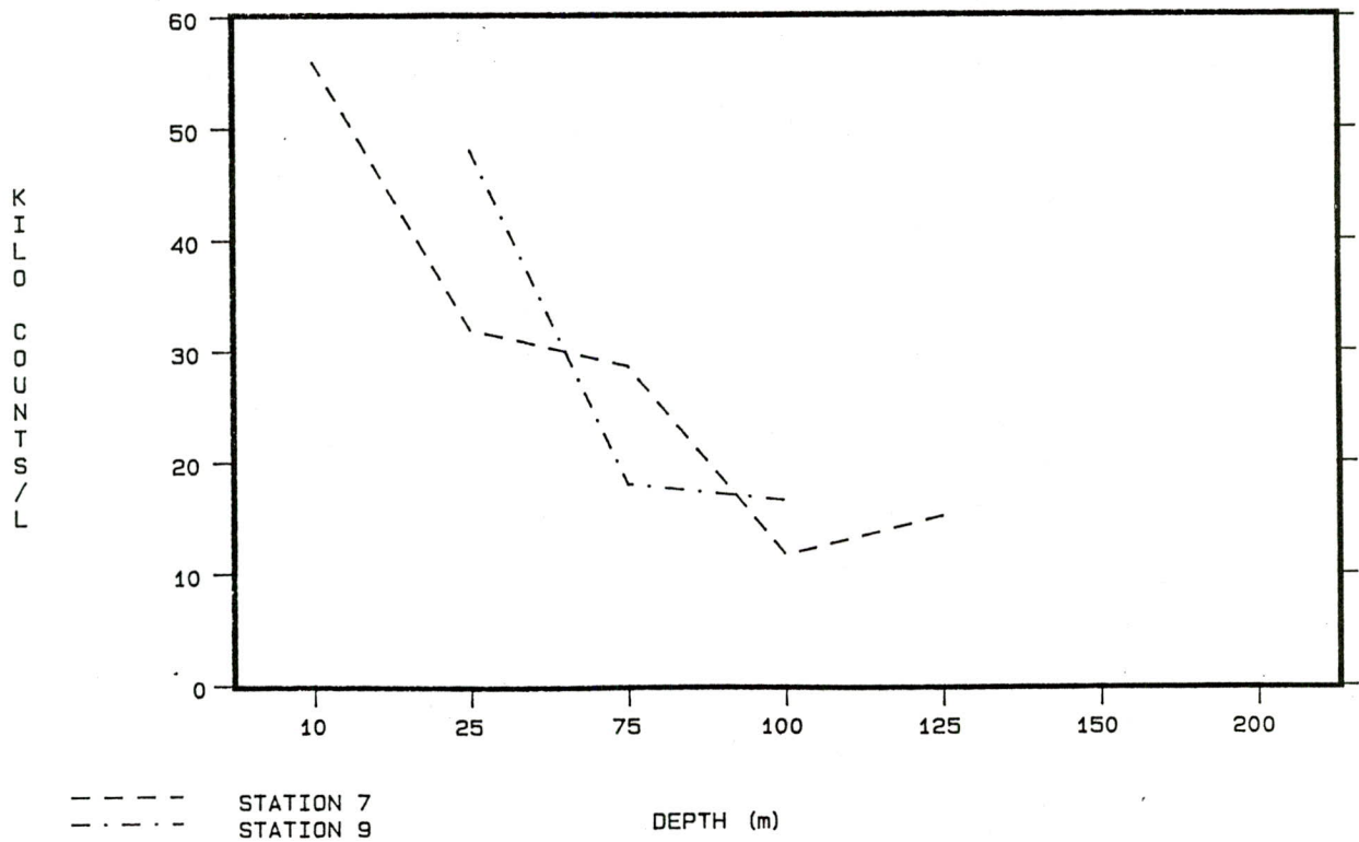
Figure 24. Large (10-100 \mu\text{m} diameter) particle counts from Exuma Sound (top) and the Straits of Florida (bottom).
