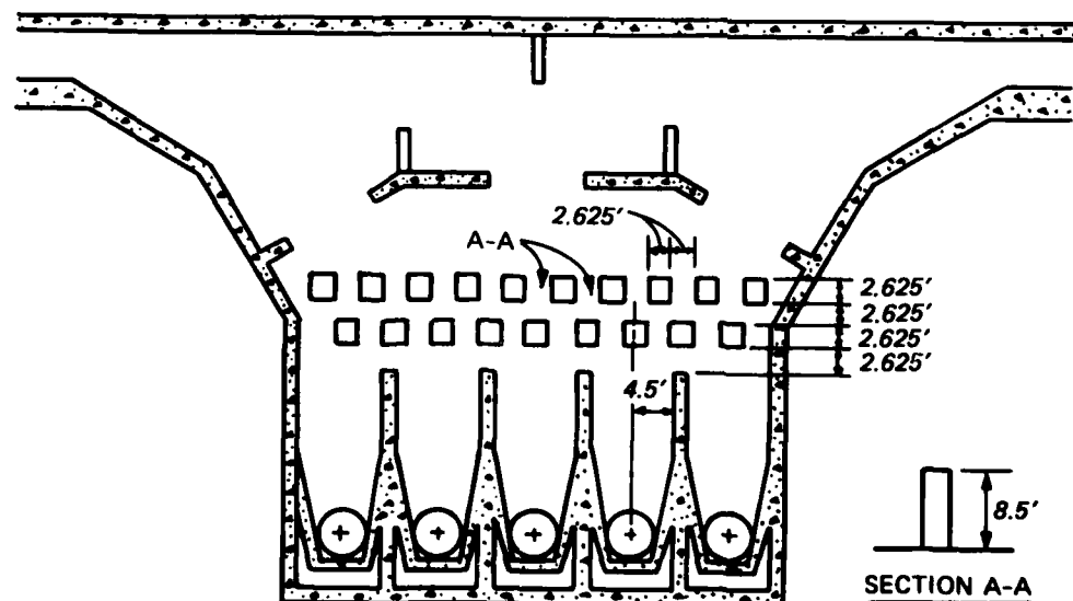
Figure 6. Type 2 design baffles
