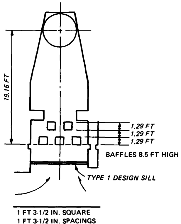
Figure 19. Type 5 design baffles
