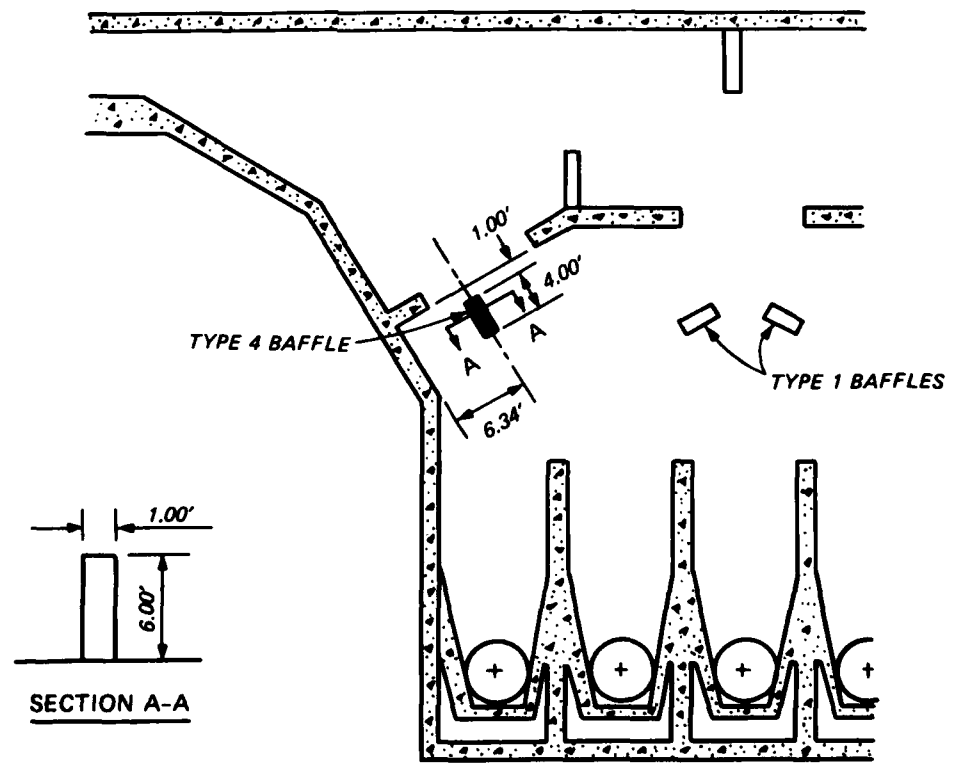
Figure 16. Type 4 design baffle
