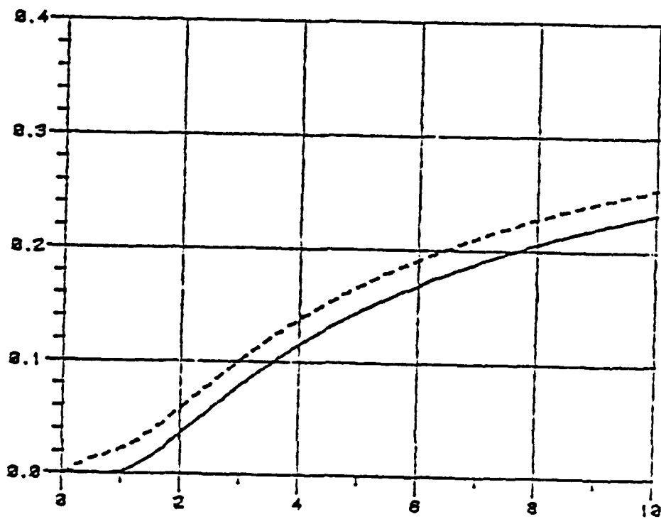
Figure 5.4b. y_{\epsilon}^0 and y_{\epsilon}^h for \kappa=0.1 , \epsilon=0.001 .
