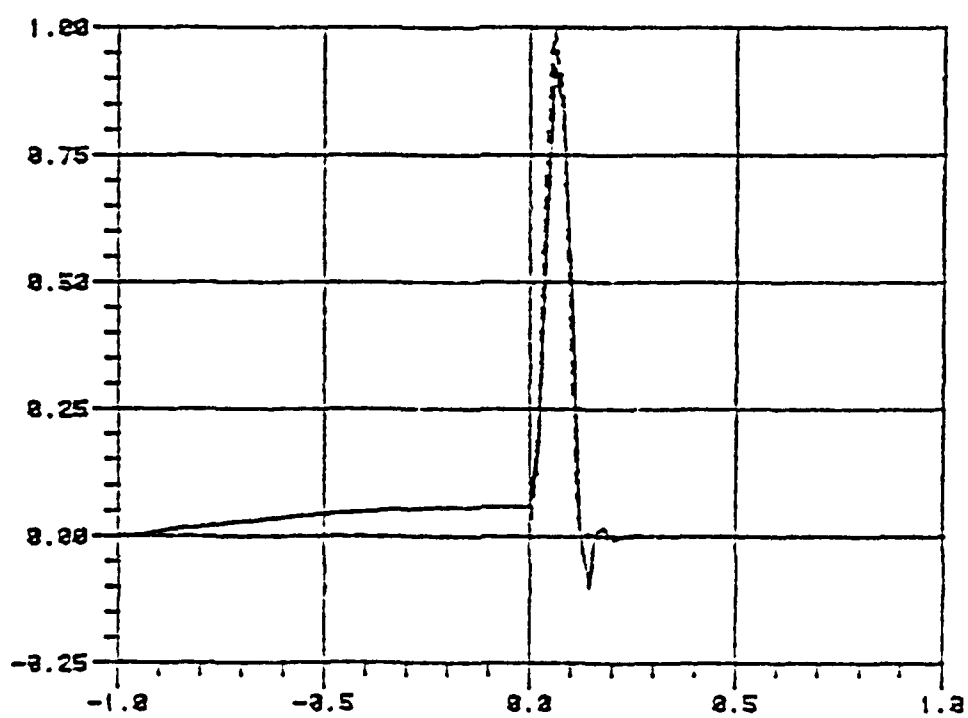
Figure 5.7b. y_{\epsilon}^0 and y_{\epsilon}^h for t=4 , \epsilon=0.001 .
