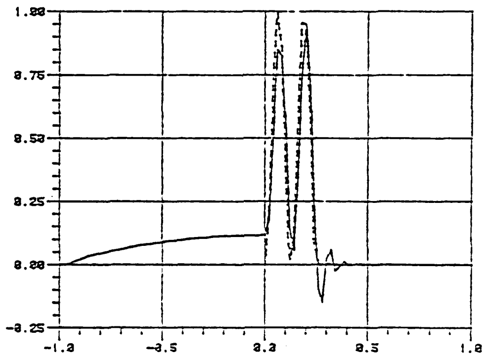
Figure 5.8b. y_{\epsilon}^0 and y_{\epsilon}^h for t=3 , \epsilon=0.001 .
