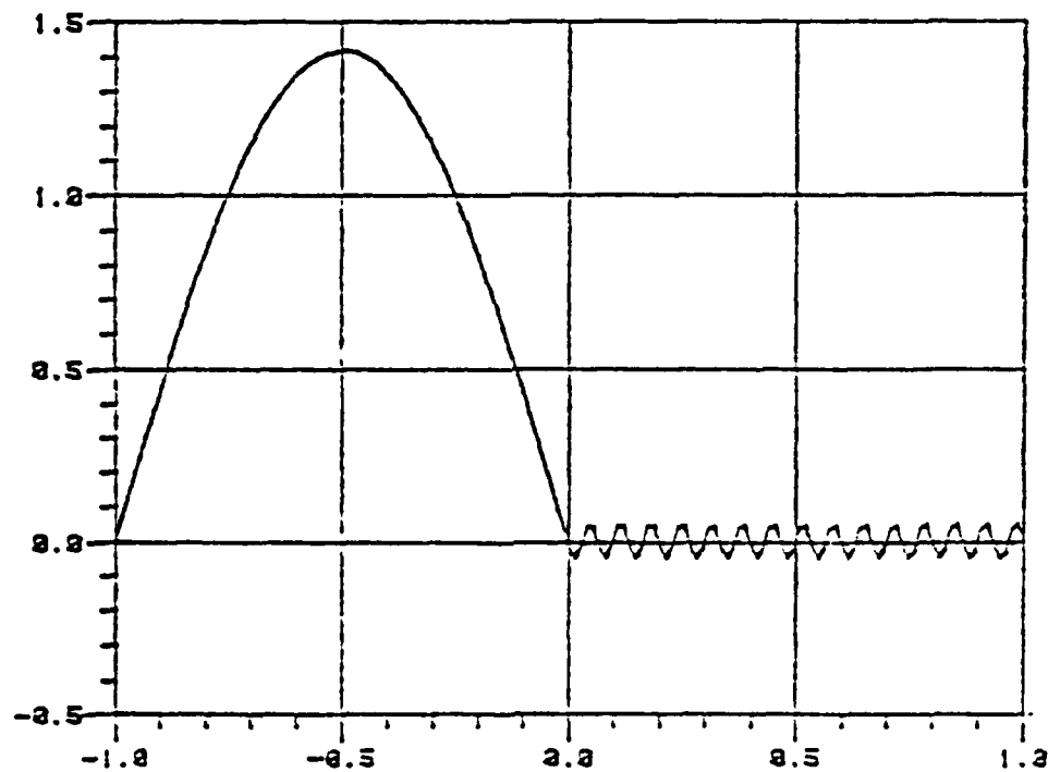
Figure 2.7d. \psi_\epsilon^1 for \epsilon = 0.0001 , N = 150 .
