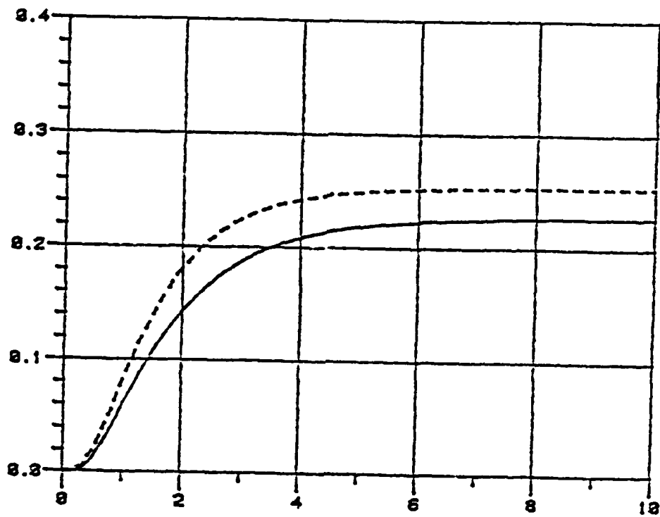
Figure 5.4a. y_{\epsilon}^0 and y_{\epsilon}^h for \kappa=0.5 , \epsilon=0.1 .
