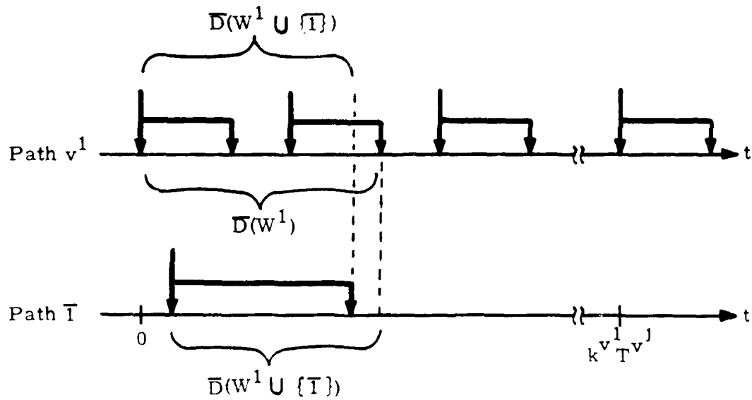
Fig. 4.7 Reduction of the effective delay by readjustment of departure times.
