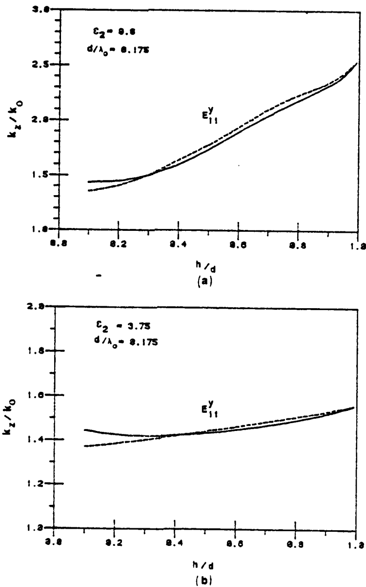
Figure 9. Normalized propagation constants of a single suspended H-waveguide vs. h/d . \epsilon_1 = \epsilon_3 = 2.3 , l = d , a = b (\infty) . Mode-matching: solid line; effective parameter: dashed line. (a) 2w/\lambda_0 = 0.165 . (b) 2w/\lambda_0 = 0.2255 .
