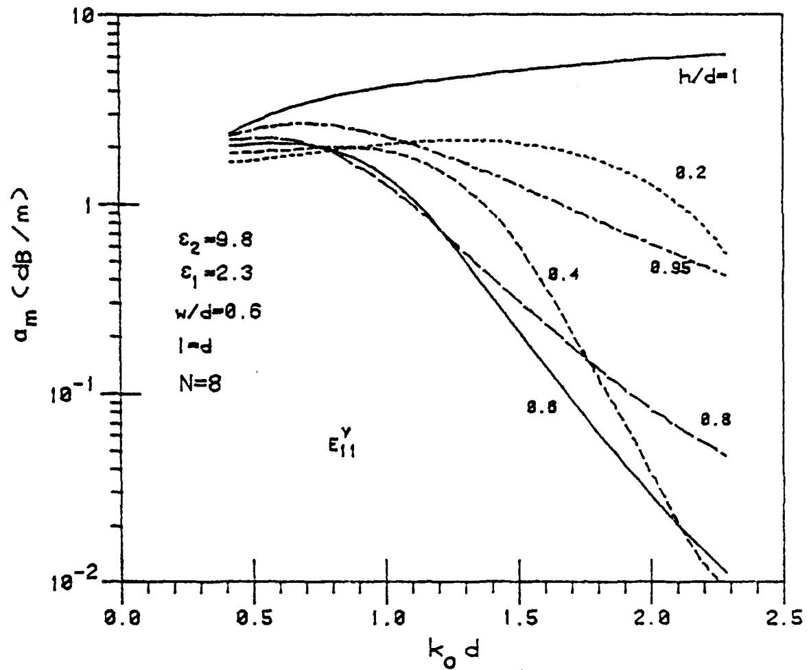
Figure 48. Attenuation of the E_{11}^y mode in decibels per meter due to the metal loss in a single suspended H-waveguide.
