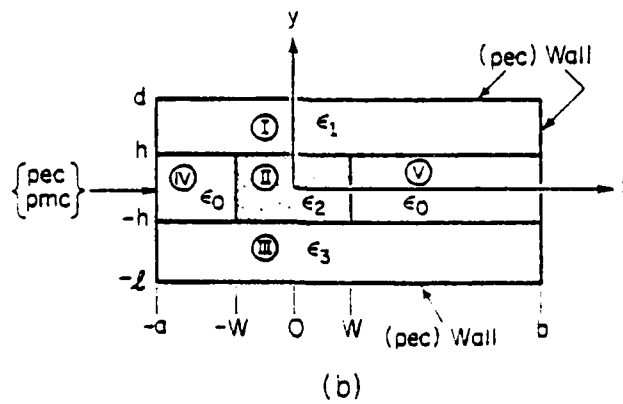
Figure 2. (a) Cross section of the coupled suspended H-waveguide.
