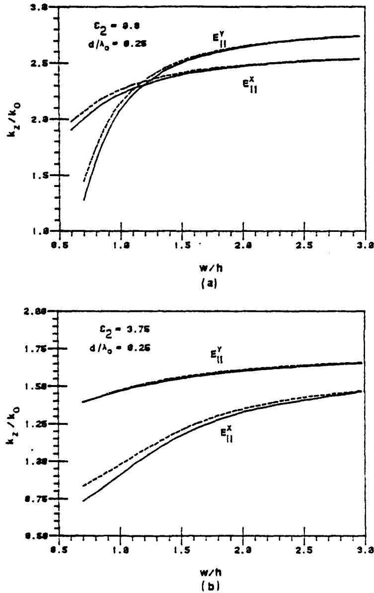
Figure 10. Normalized propagation constants of a single suspended H-waveguide vs. w/h . \epsilon_1 = \epsilon_3 = 2.3 , l = d , a = b (\rightarrow \infty) . Mode matching: solid line; effective parameter: dashed-line. (a) \epsilon_2 = 9.8 ; (b) \epsilon_2 = 3.75 .
