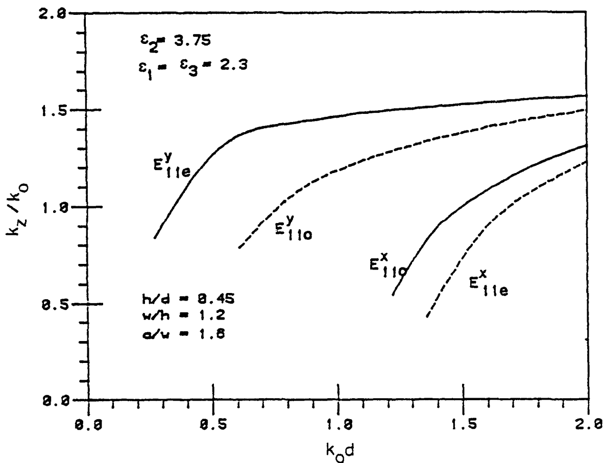
Figure 19. Normalized propagation constants of even and odd E_{11}^y and E_{11}^x modes of a coupled suspended H-waveguide vs. the normalized free-space wavenumber. l = d , b/w = \infty .
