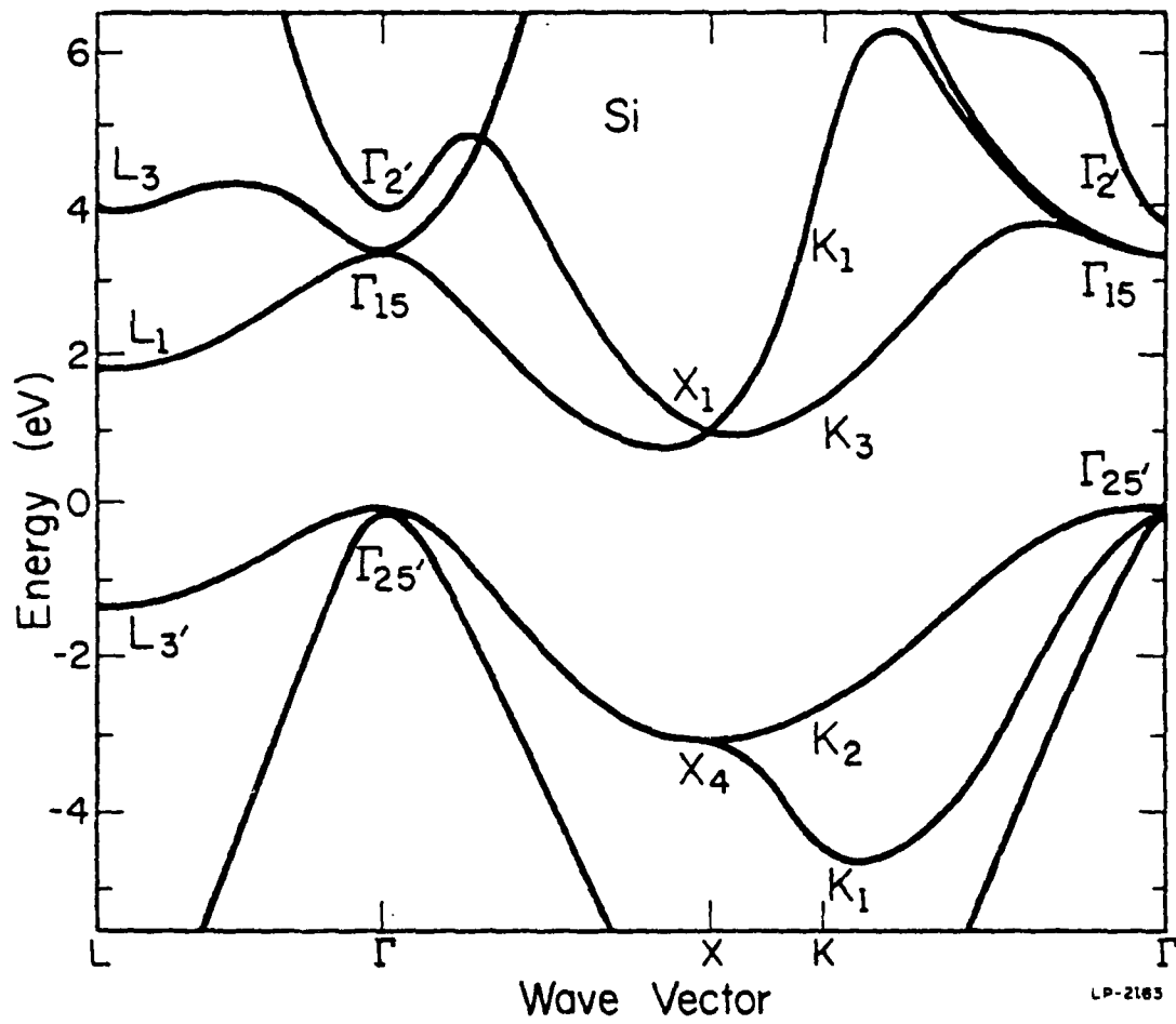
Figure 4.1: The band structure of silicon calculated by the empirical pseudopotential method [37].
