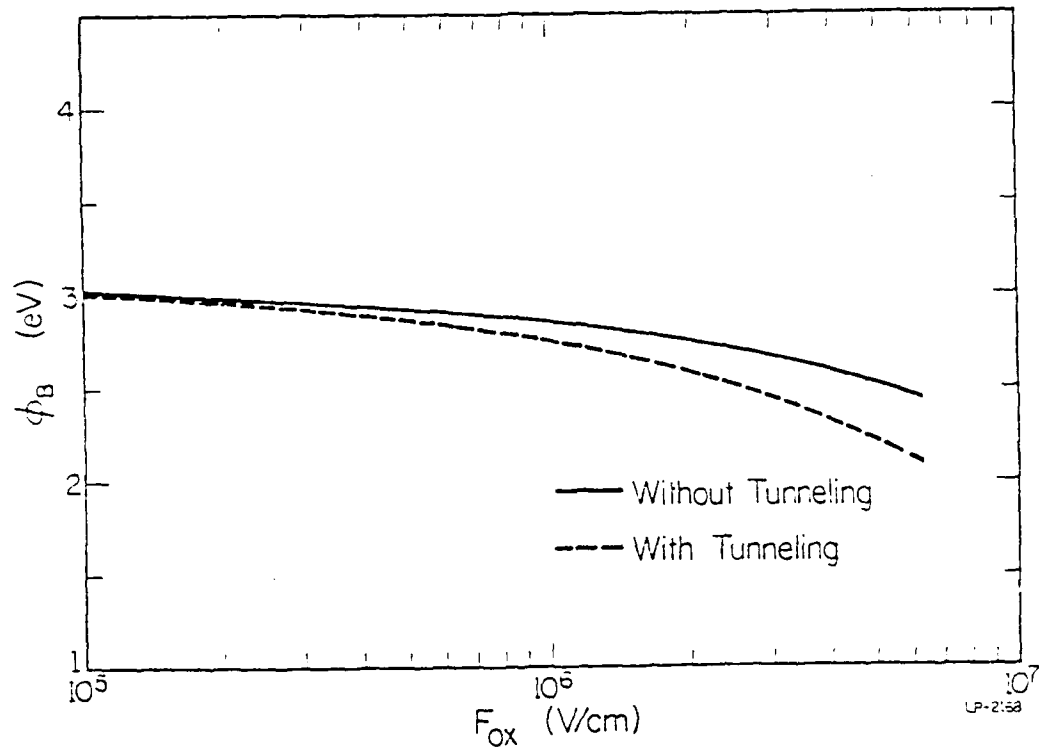
Figure 5.4: Effective barrier height plotted against the oxide field strength. The solid line is without tunneling and the dashed line is with tunneling.
