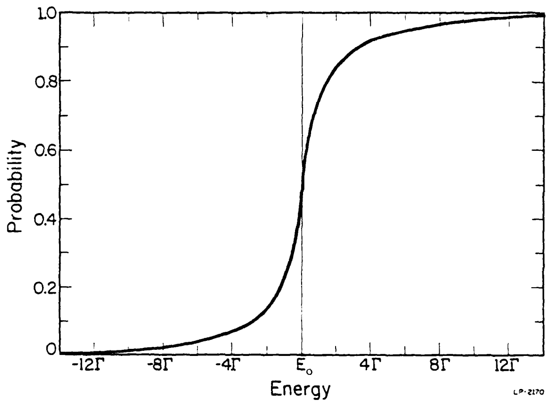
Figure 6.8: The escape probability as described in the text.
