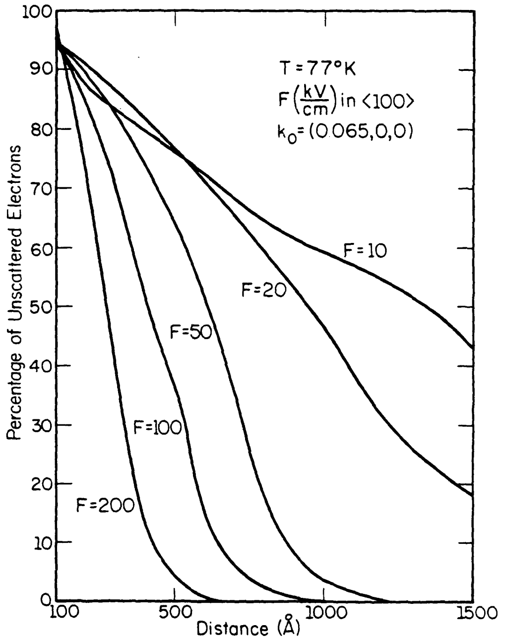
Figure 3.3(b): The percentage of unscattered electrons as a function of device length with the electric field as a parameter at T = 77 K. These curves correspond to those of Figure 3.2b.
