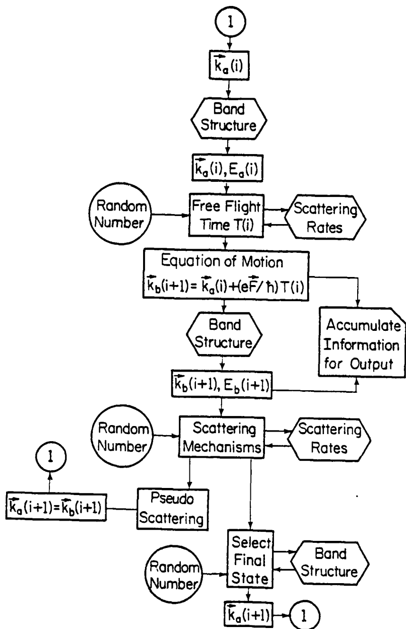
Figure 2.1: Flow chart of a Monte Carlo simulation.
