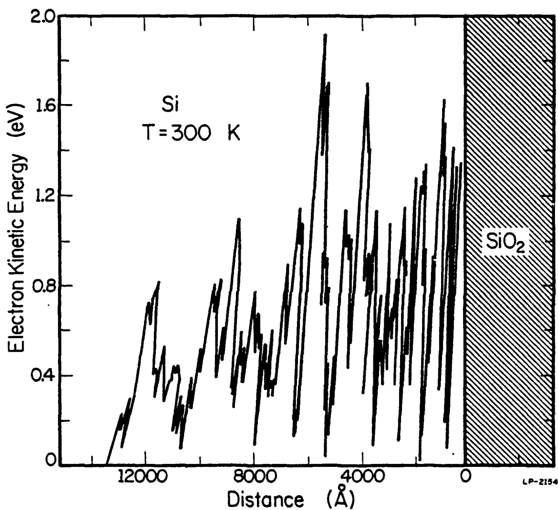
Figure 5.7: The histogram of the kinetic energy of the same electron as in Figure 5.6.
