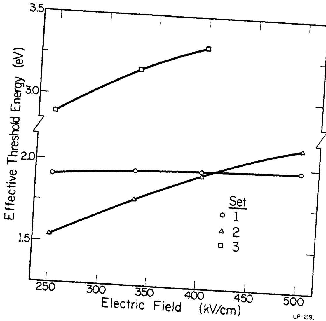
Figure 4.12: The effective threshold energy of impact ionization plotted against the electric field for the three sets of transport parameters.
