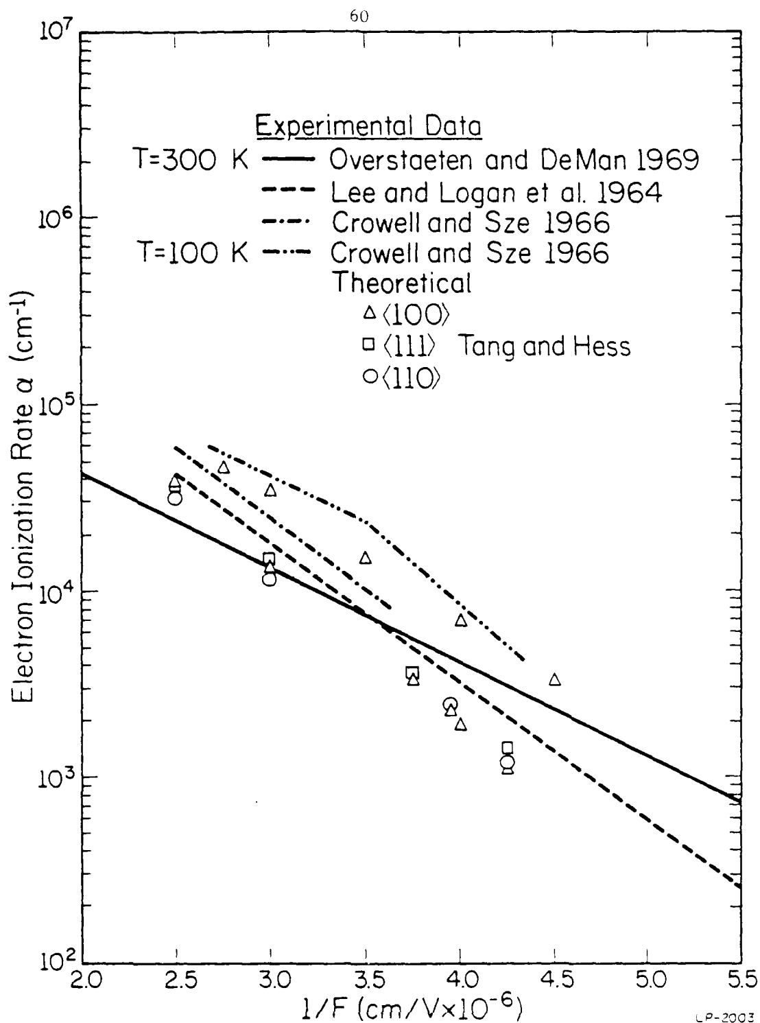
Figure 4.7: Calculated electron ionization coefficient \alpha plotted as a function of inverse field strength.
