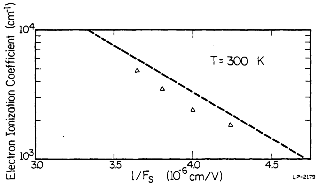
Figure 5.11: The electron ionization coefficient plotted against the surface field.
