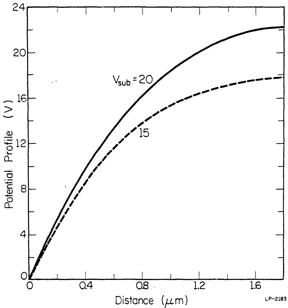
Figure 5.2(a): Potential profiles in the depletion region for device 15-2-9.
