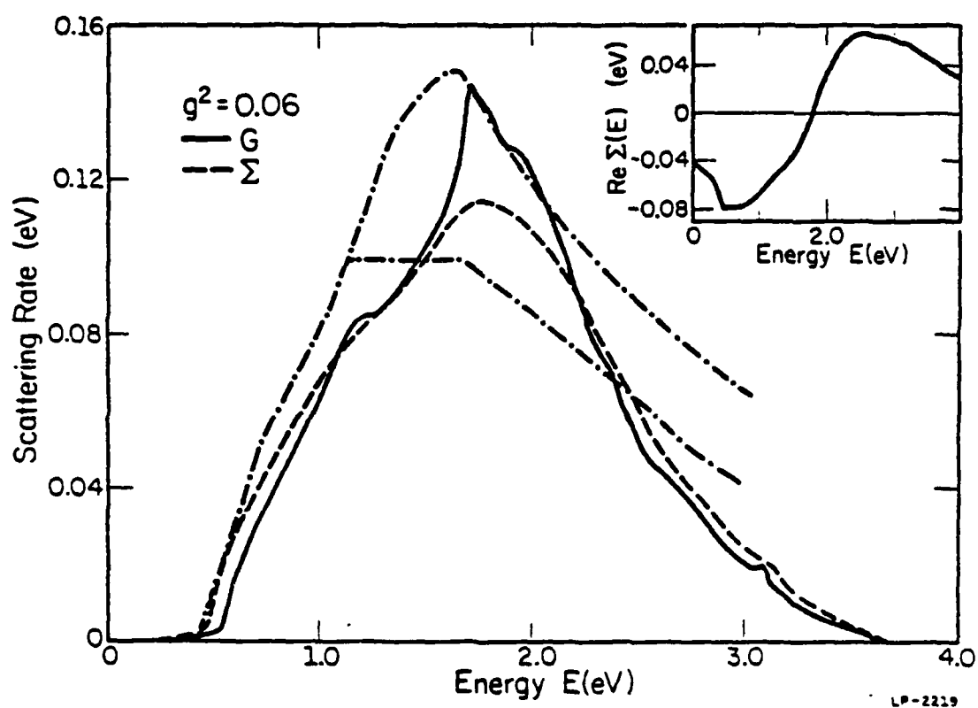
Figure 6.2: The scattering rates (the imaginary part of the self-energy) plotted as a function of the electron energy. The solid curve corresponds to the first order self-energy and the dashed curve corresponds to the full order self-energy. The dash-dotted curves are that used in the calculations. The inset shows the real part of the self-energy.
