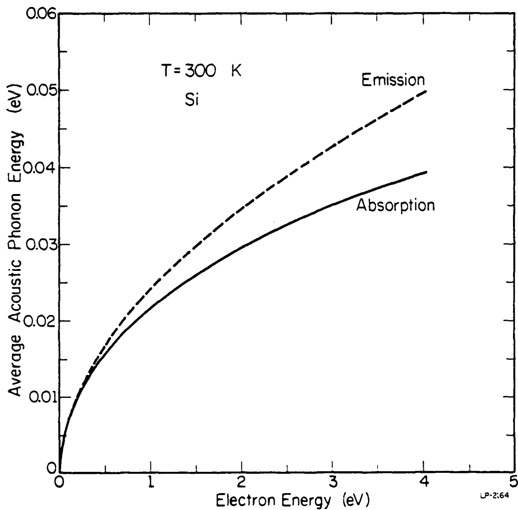
Figure A2.2: The average acoustic phonon energy as a function of the electron energy for both emission and absorption.
