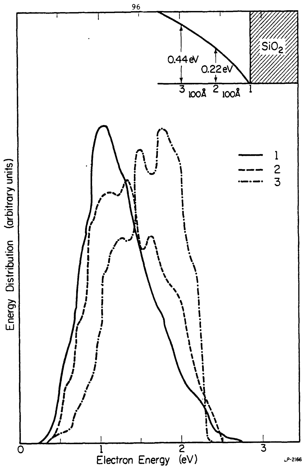
Figure 5.10: The energy distribution of electrons at three positions for the second simulation.
