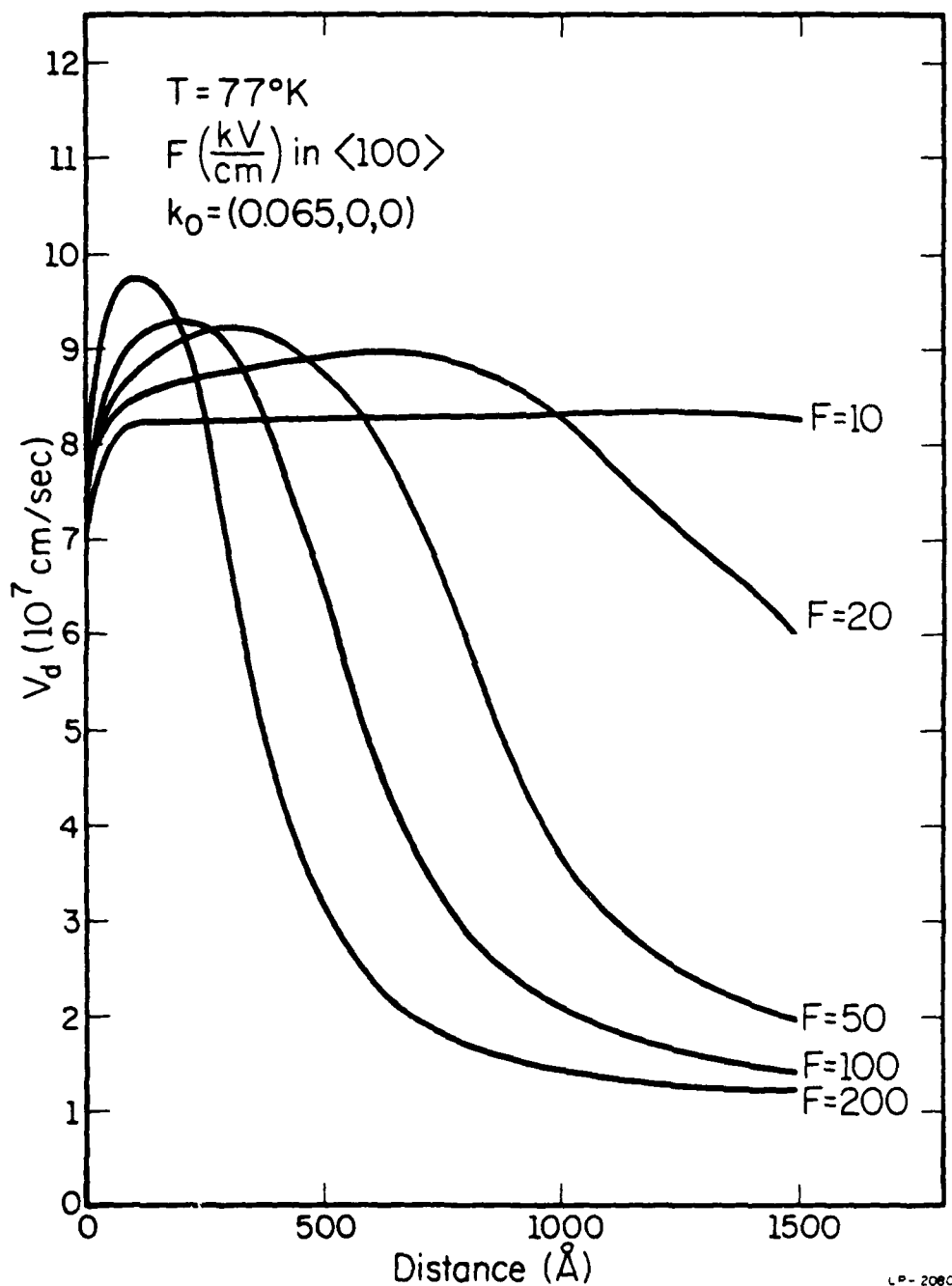
Figure 3.2(b): Average drift velocity versus the device length with the electric field as a parameter at T = 77 \text{ K} . The initial k_0 given in units of 2\pi/a , where "a" is the lattice constant. The injection energy corresponding to k_0 is E_0 = 0.24 \text{ eV} .
