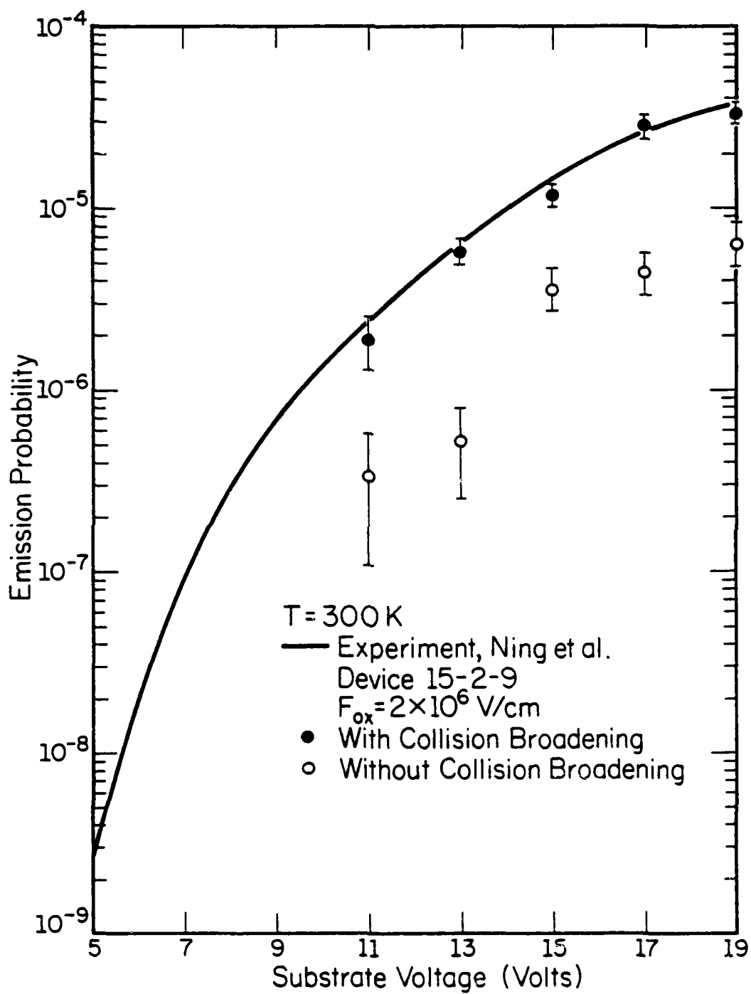
Figure 5.8: The calculated emission probability as a function of the substrate voltage.
