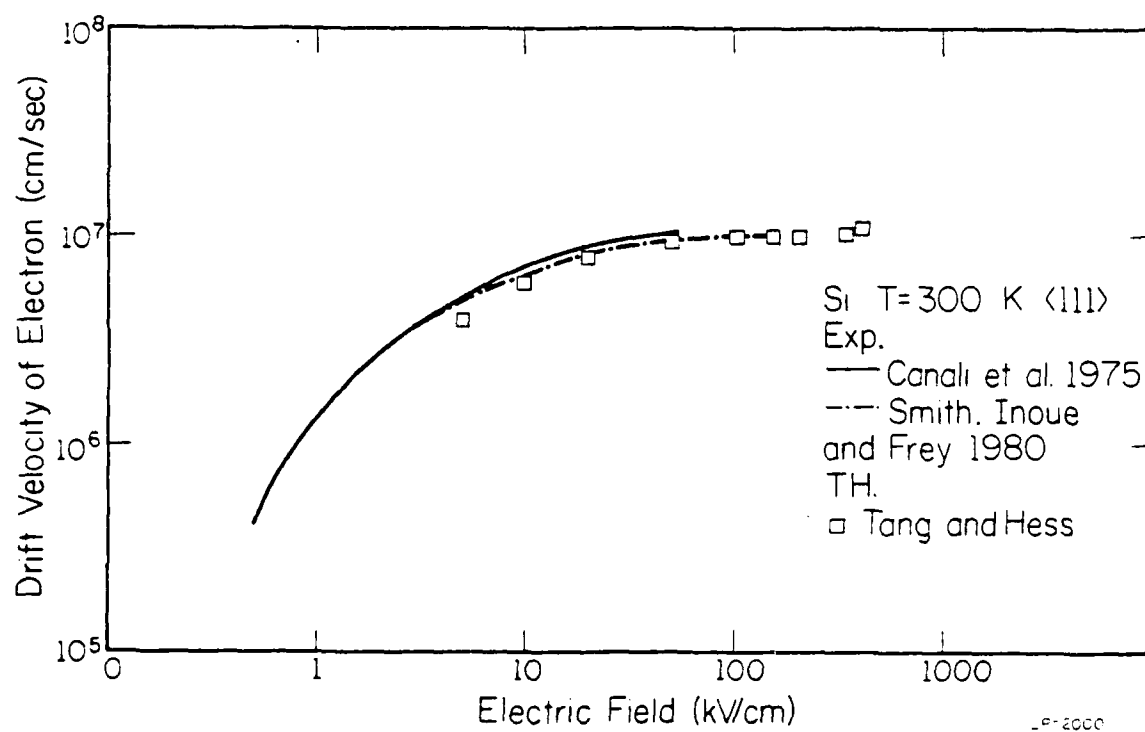
Figure 4.6: Calculated drift velocities for silicon along the <111> direction. The dashed line and the solid line are the experimental results.
