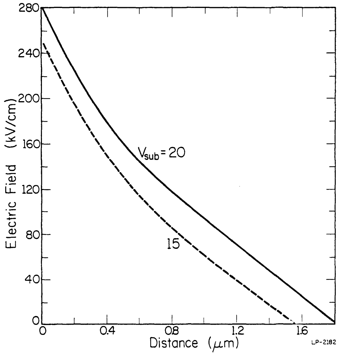
Figure 5.2(b): Electric field profiles in the depletion region for device 15-2-9.
