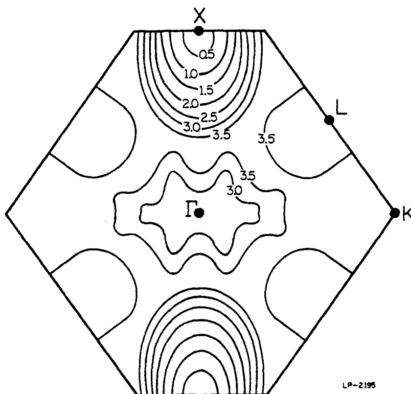
Figure 4.5(b): Equal energy surfaces for the second conduction band of silicon corresponding to the cross section of Figure 4.4.
