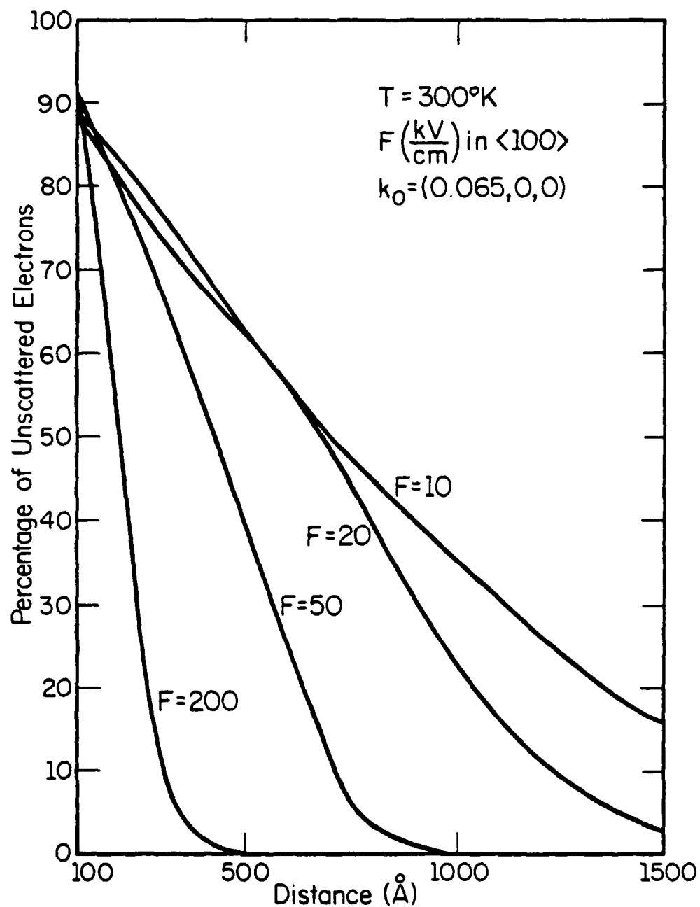
Figure 3.3(a): The percentage of unscattered electrons as a function of device length with the electric field as a parameter at T = 300 \text{ K} . These curves correspond to those of Figure 3.2a.
