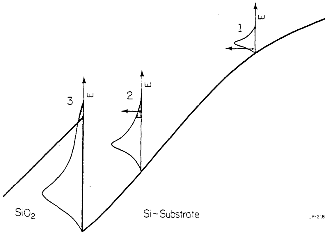
Figure 5.5: Schematic diagram for the Monte Carlo simulation.
