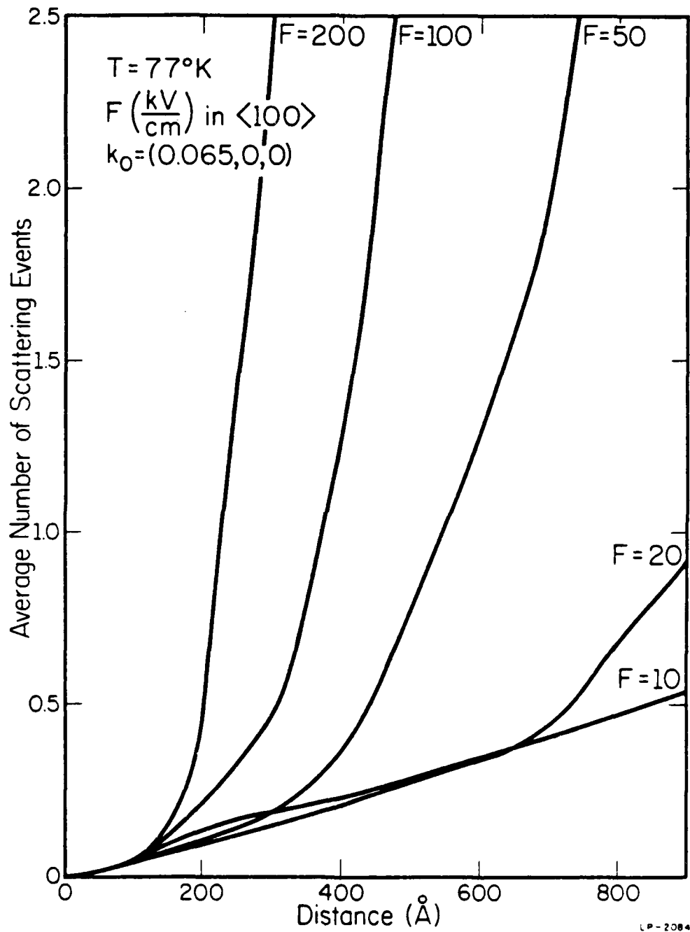
Figure 3.4(b): The average number of scattering events as a function of device length with the electric field as a parameter at T = 77 K. The curves here correspond to those of Figure 3.2b.
