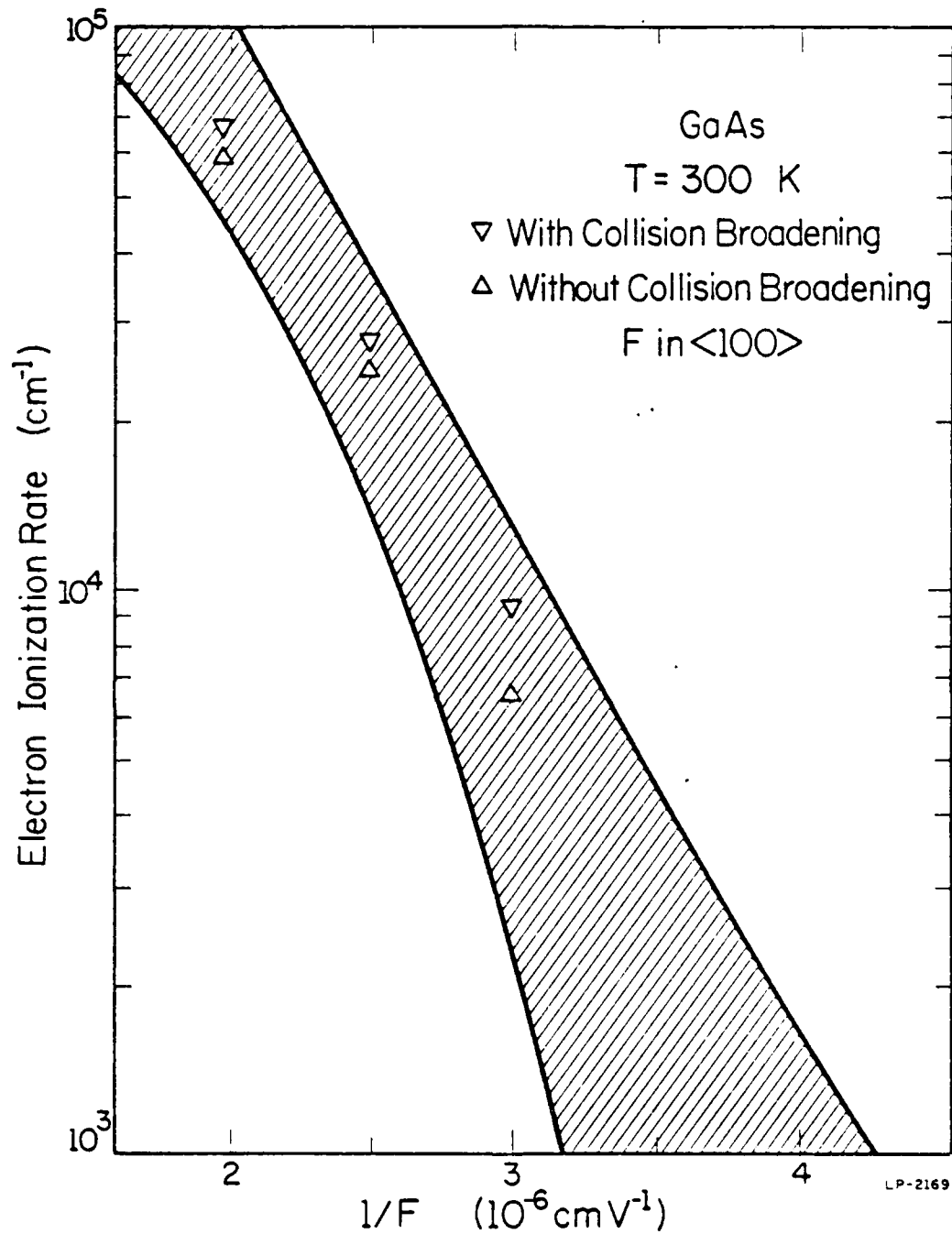
Figure 6.6: Calculated ionization coefficients as a function of the inverse field strength. The shaded region represents the available experimental results.
