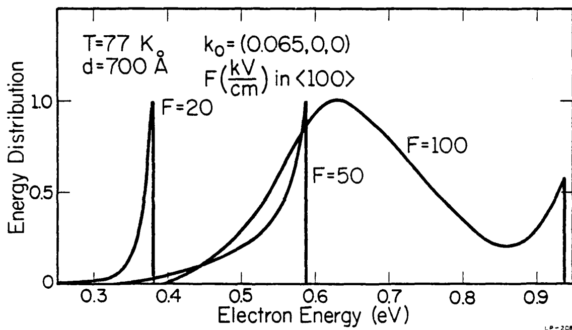
Figure 3.6: Energy distribution at d = 700 \text{ Å} for T = 77 \text{ K} . The electric fields are all in the \langle 100 \rangle direction and the injection energy is the same as in the previous graphs.
