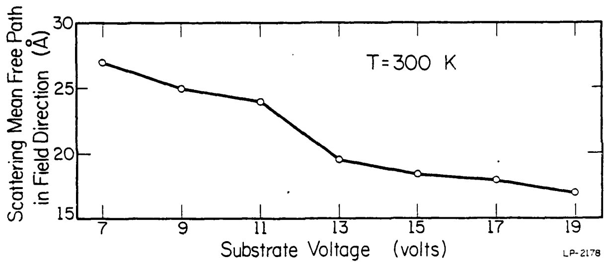
Figure 5.12: The scattering mean free path in the field direction plotted as a function of substrate voltage for device 15-2-9.
