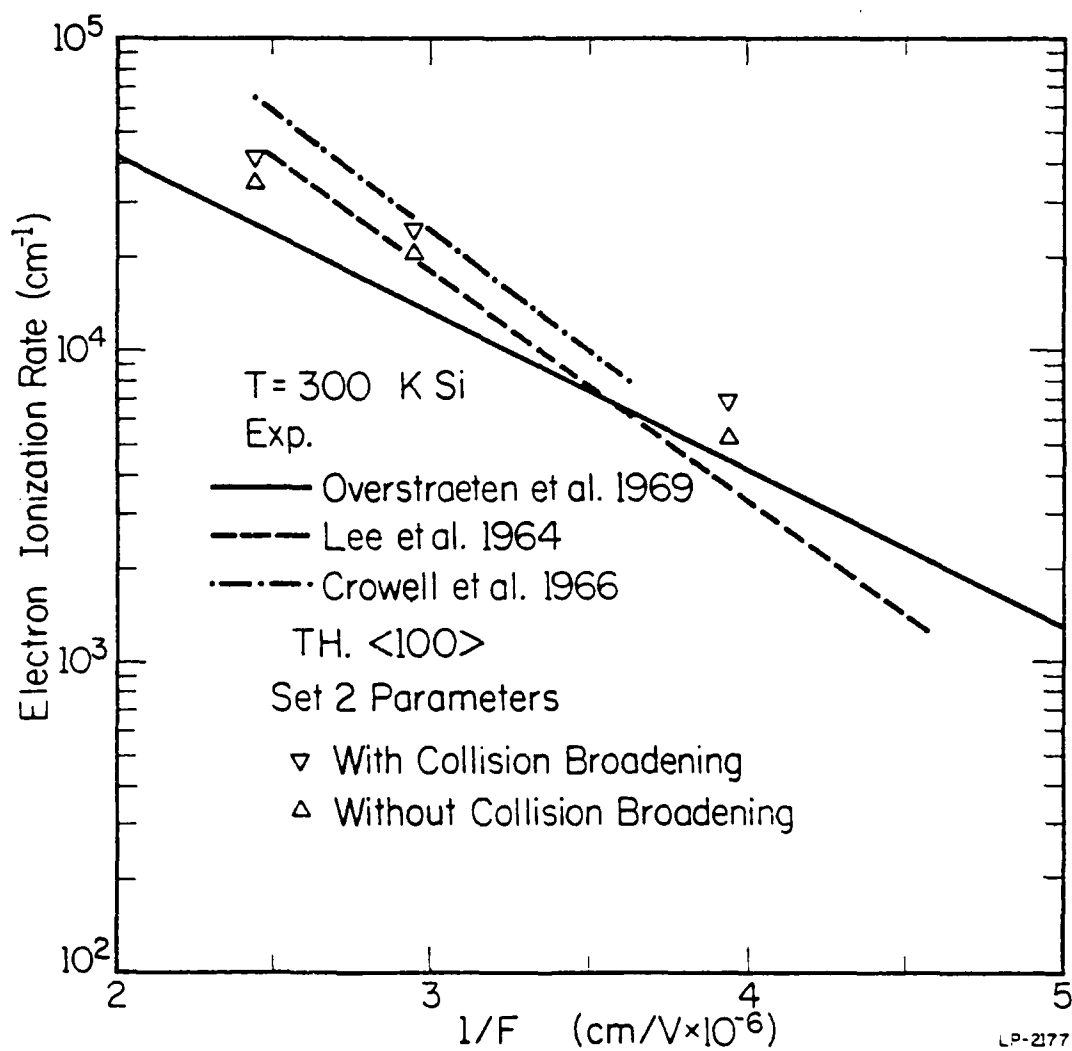
Figure 6.7: Calculated ionization coefficients as a function of the inverse field strength.
