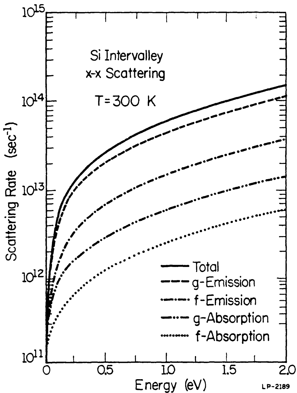
Figure A2.3: Intervalley scattering rates in silicon.
