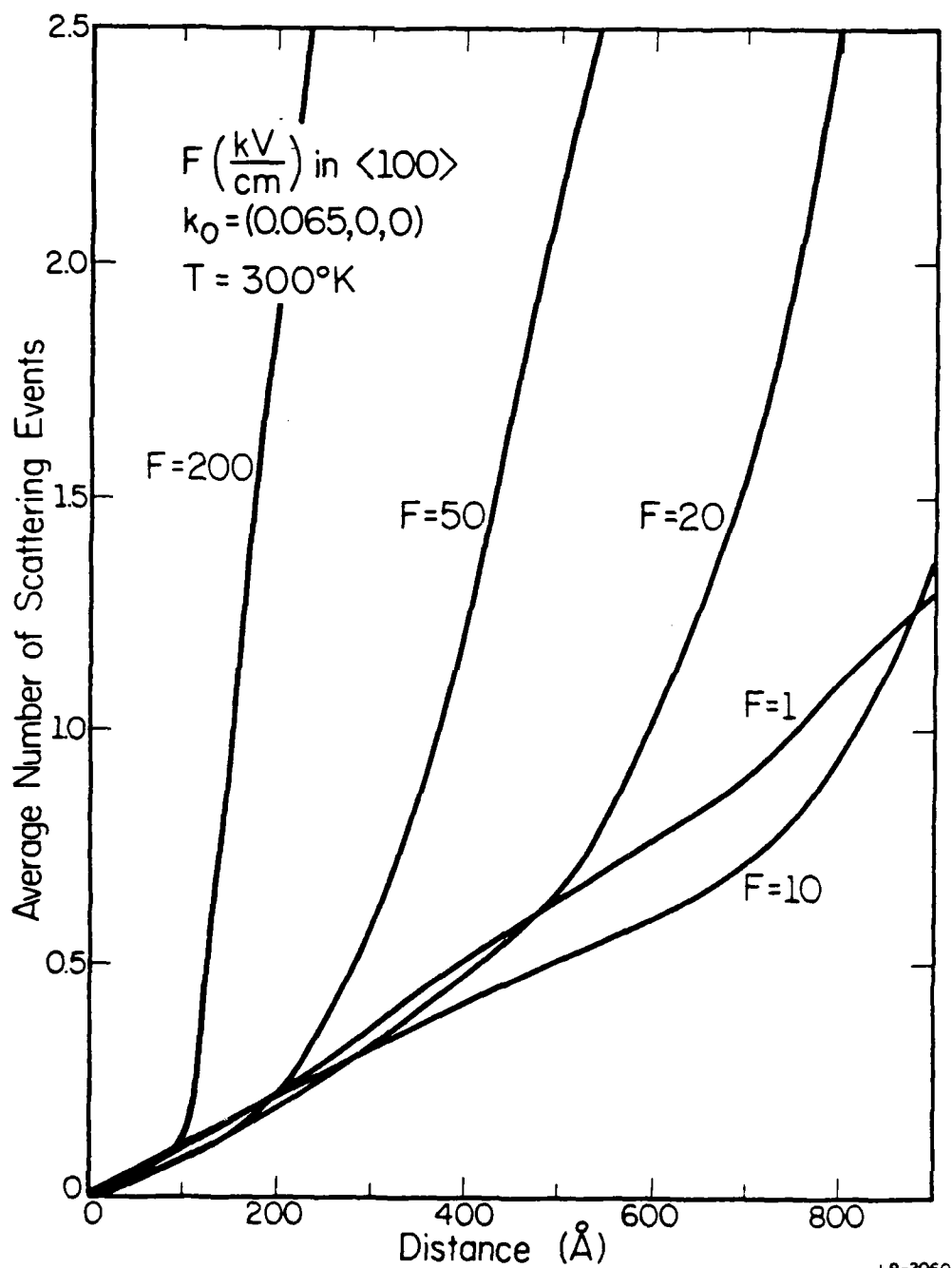
Figure 3.4(a): The average number of scattering events as a function of device length with the electric field as a parameter at T = 300 K. The curves here correspond to those of Figure 3.2a.
