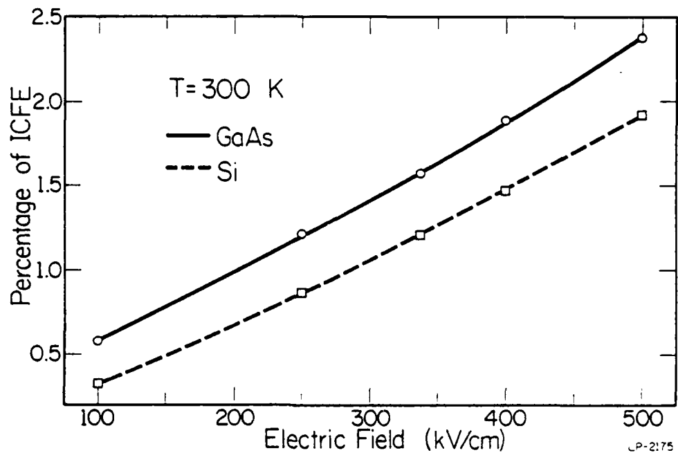
Figure 6.9: The intra-collisional field effect (ICFE) as a function of electric field for GaAs and Si.
