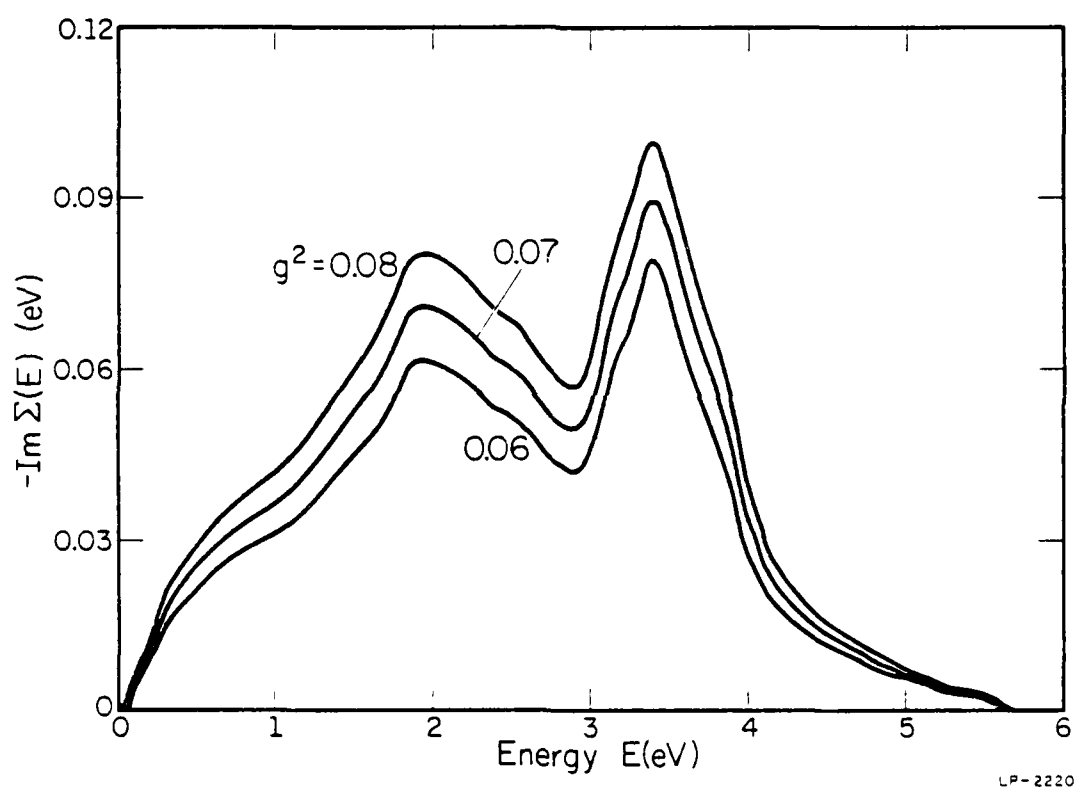
Figure 6.5: The imaginary part of the self-energy for different coupling constants.
