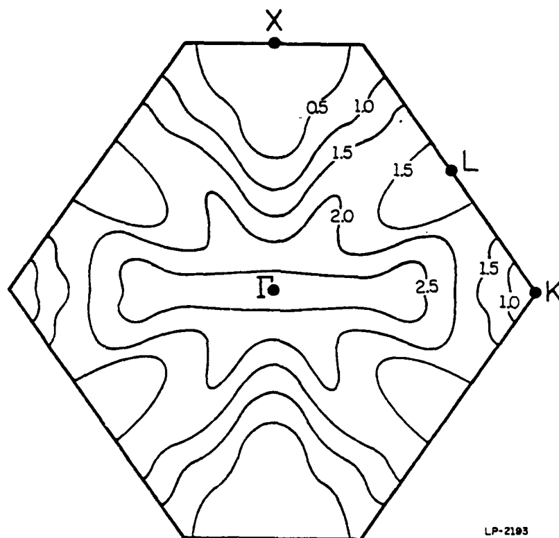
Figure 4.5(a): Equal energy surfaces for the first conduction band of silicon corresponding to the cross section of Figure 4.4.
