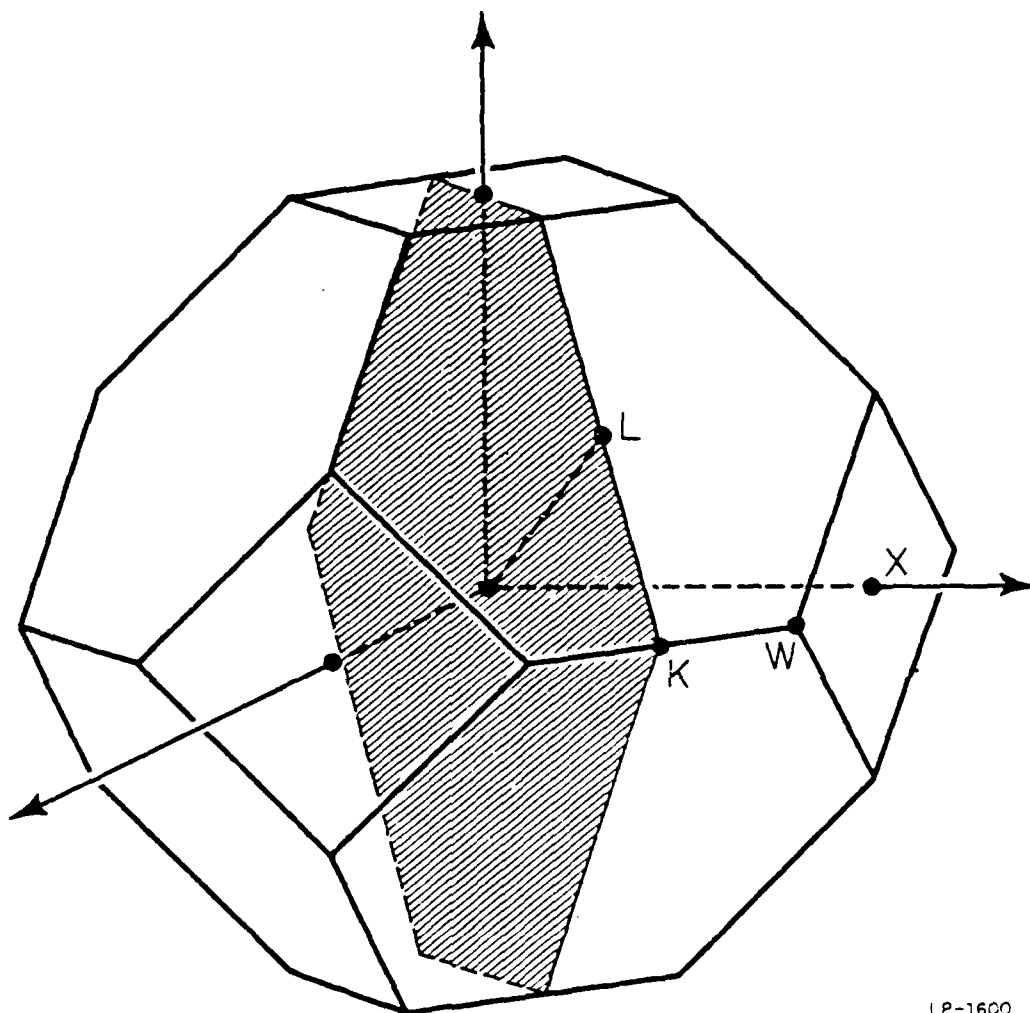
Figure 4.4: A cross section of the Brillouin zone.
