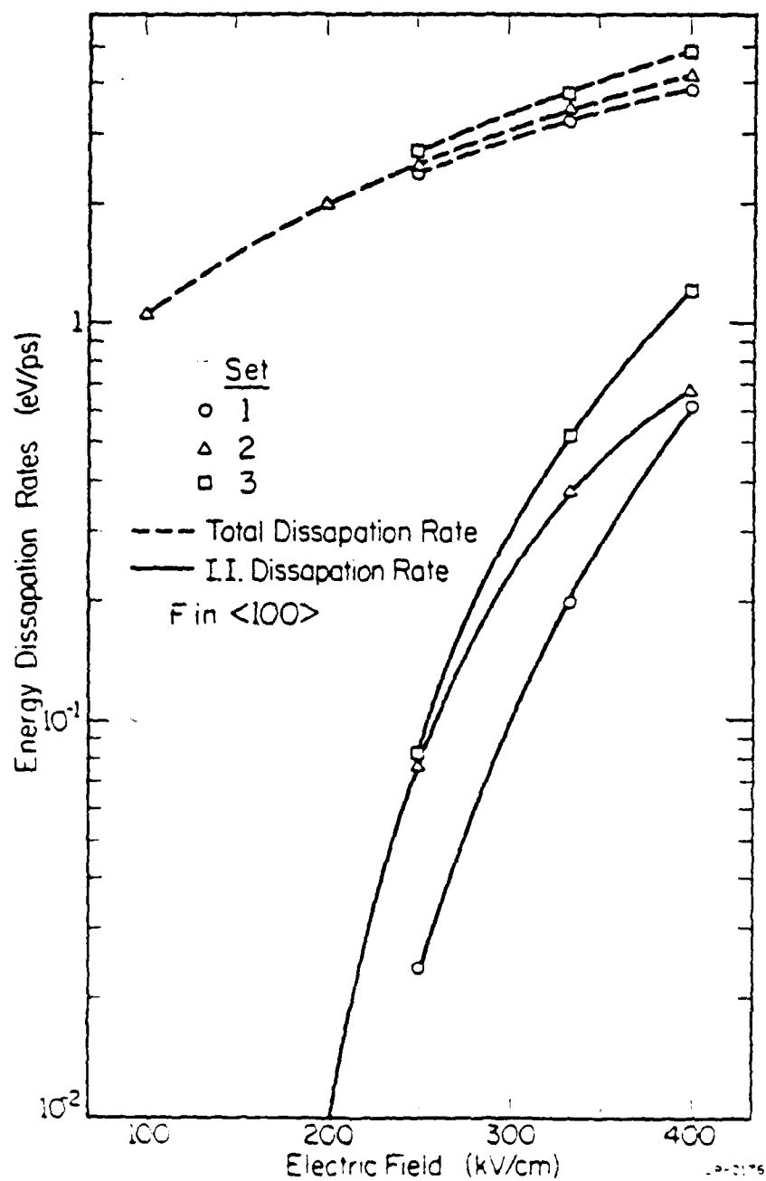
Figure 4.15: The total energy dissipation rate and the impact ionization dissipation rate plotted against the electric field for the three sets of transport parameters.
