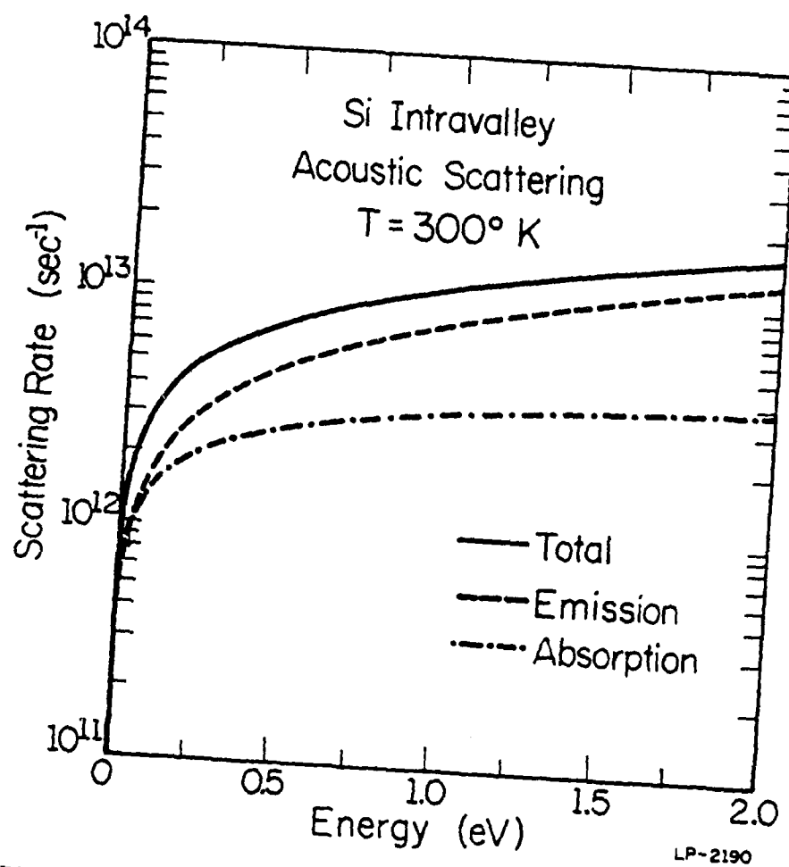
Figure A2.1: Acoustic phonon scattering rate as a function of the electron energy.
