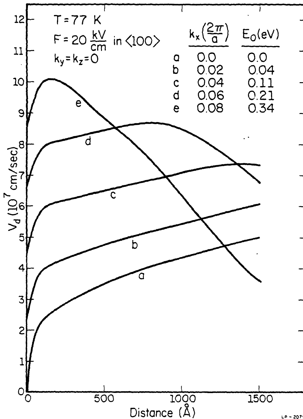
Figure 3.1(b): Average drift velocity versus the device length with injection energy as a parameter at T = 77 \text{ K} . The electric field is applied in the \langle 100 \rangle direction.
