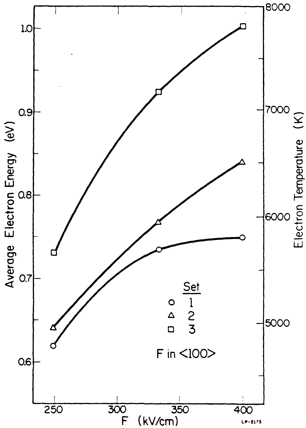
Figure 4.14: The average electron energy as a function of the electric field. The right scale is the corresponding electron temperature ..
