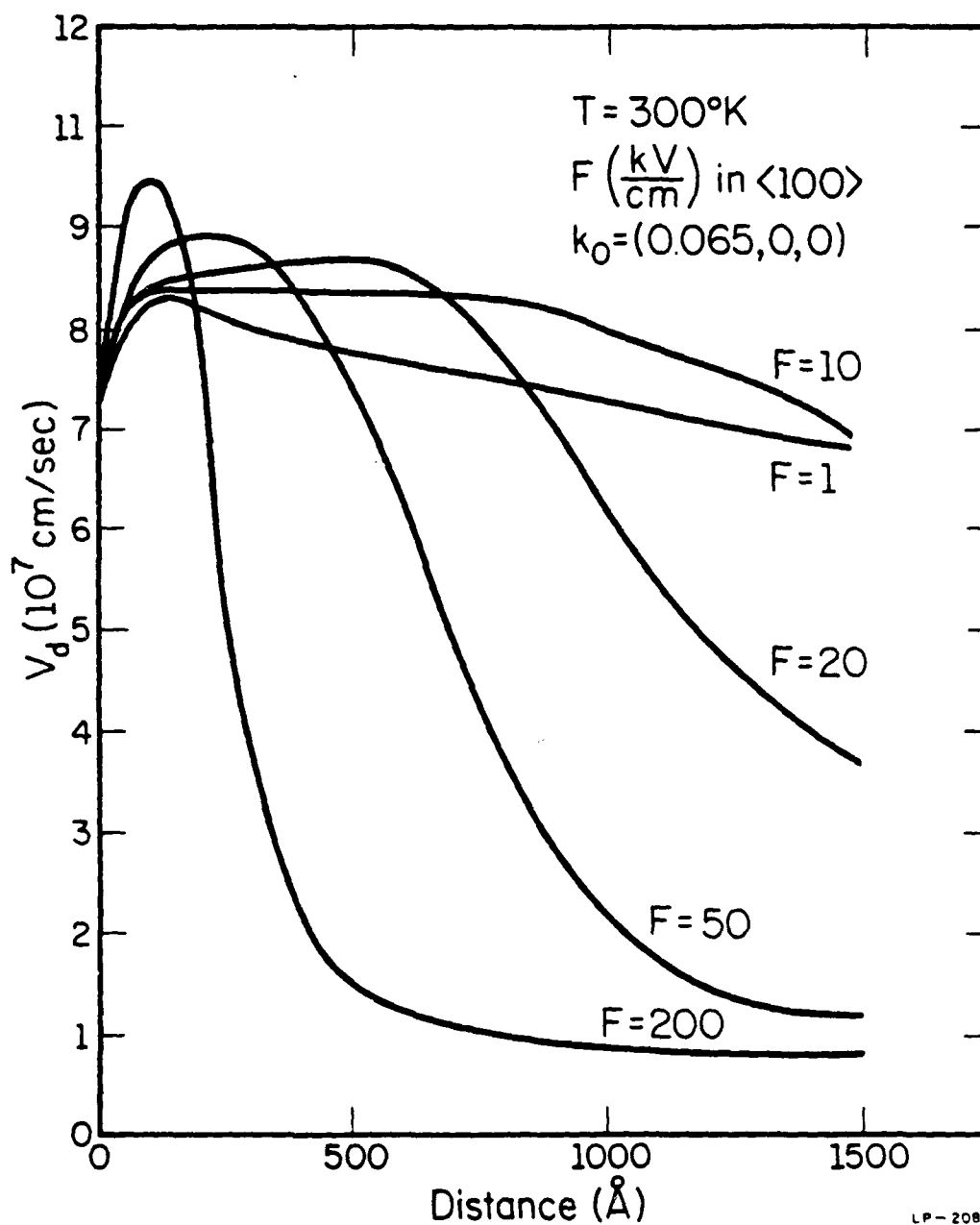
Figure 3.2(a): Average drift velocity versus the device length with the electric field as a parameter at T = 300 K. The initial k_0 is given in units of 2\pi/a , where "a" is the lattice constant. The injection energy corresponding to k_0 is E_0 = 0.24 eV.
