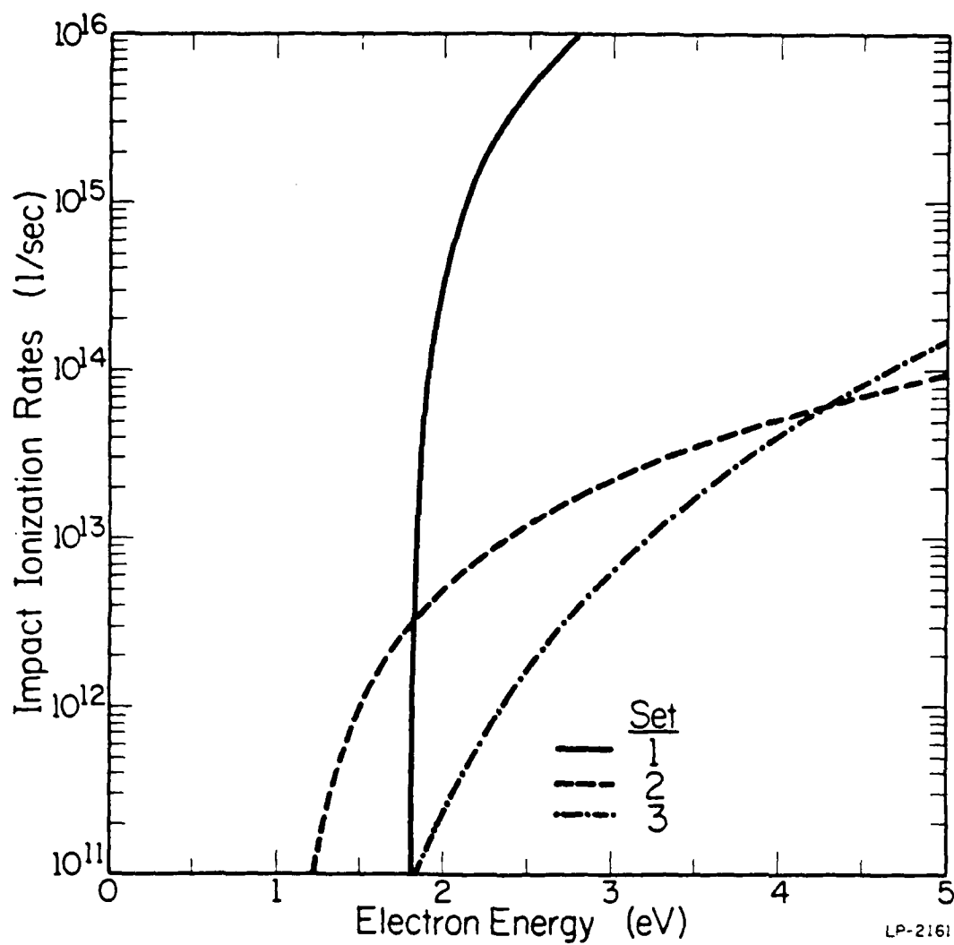
Figure 4.10: Impact ionization scattering rates for the three sets of transport parameters plotted as a function of energy.
