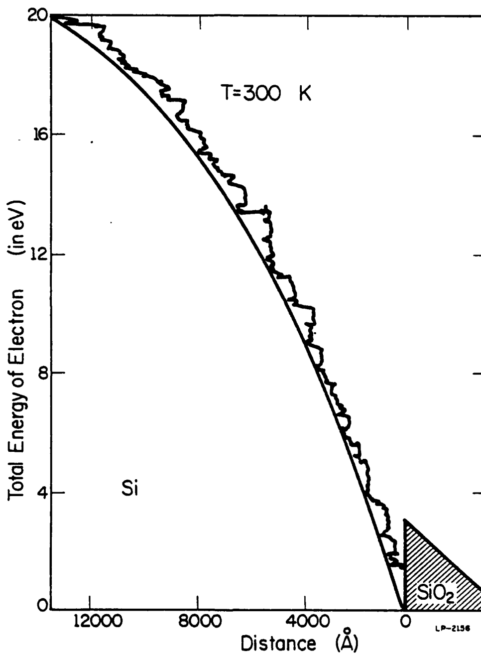
Figure 5.6: Energy histogram of an electron.
