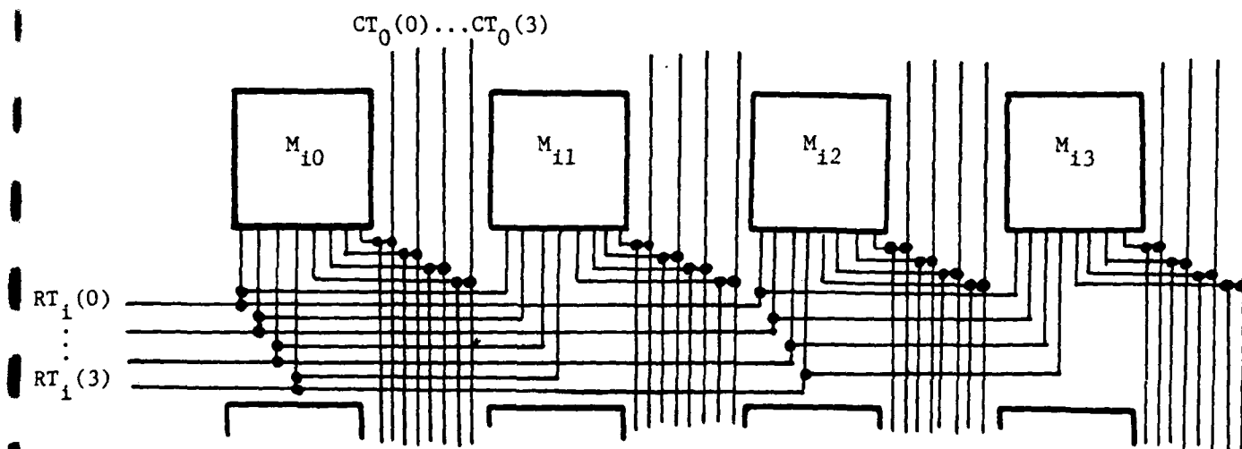
Figure 4. Interconnection of modules and trees.
