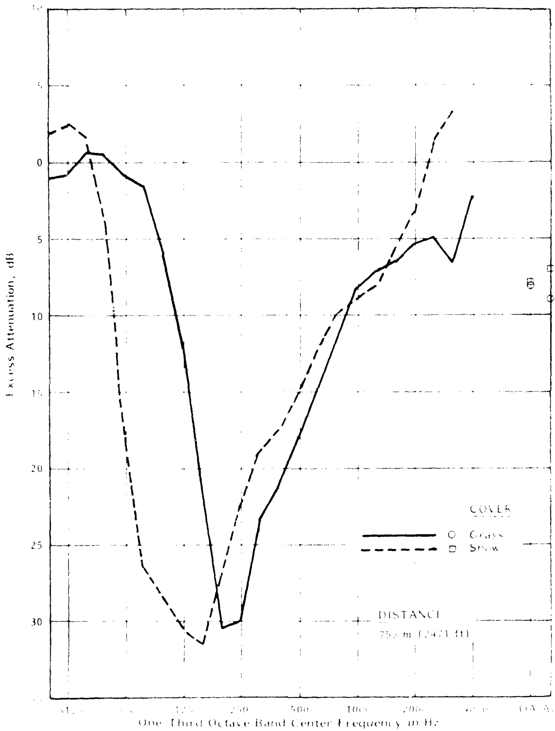
FIGURE 1-10. AVERAGE EXCESS ATTENUATION FOR GRASS OR SNOW COVER UNDER LOW WIND AND NEAR NEUTRAL TEMPERATURE GRADIENT CONDITIONS.
