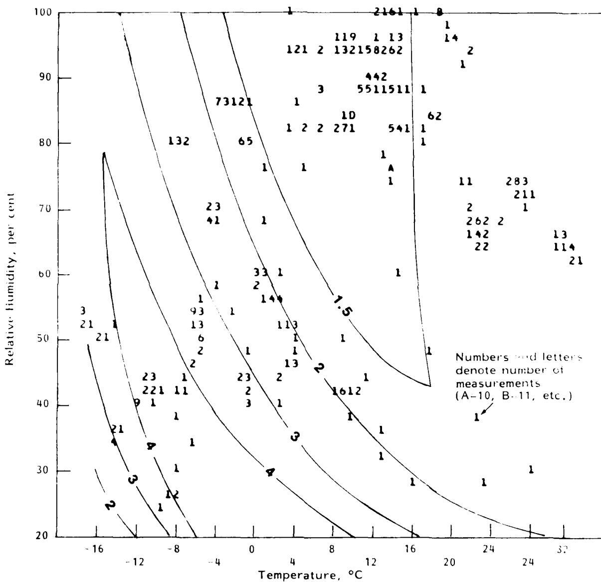
FIGURE 2. FIELD RELATIVE HUMIDITY VERSUS FIELD TEMPERATURE
