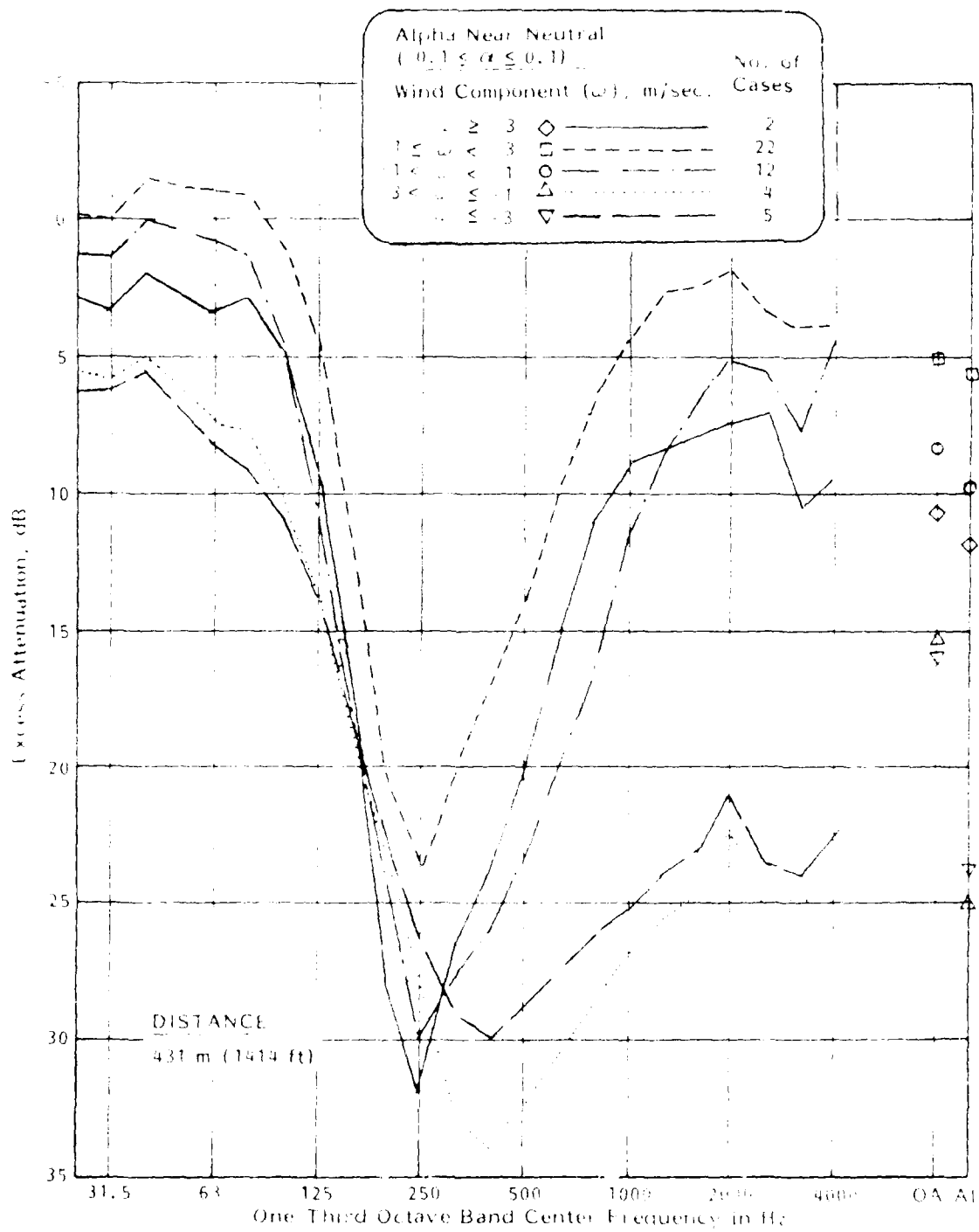
FIGURE 11. C VARIATION IN EXCESS ATTENUATION WITH WIND COMPONENT UNDER NEAR NEUTRAL TEMPERATURE/FABENT CONDITION. DISTANCE 431 m (1414 ft)
