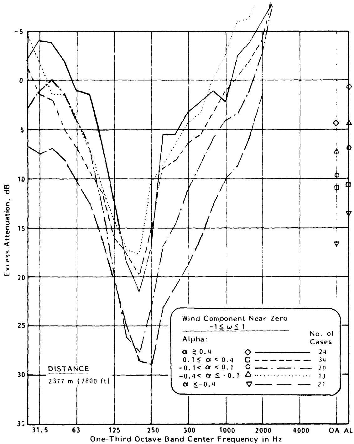
FIGURE 19 C. VARIATION IN EXCESS ATTENUATION WITH TEMPERATURE GRADIENT FOR SMALL WIND COMPONENT CONDITIONS - DISTANCE 2377 m (7800 ft)
