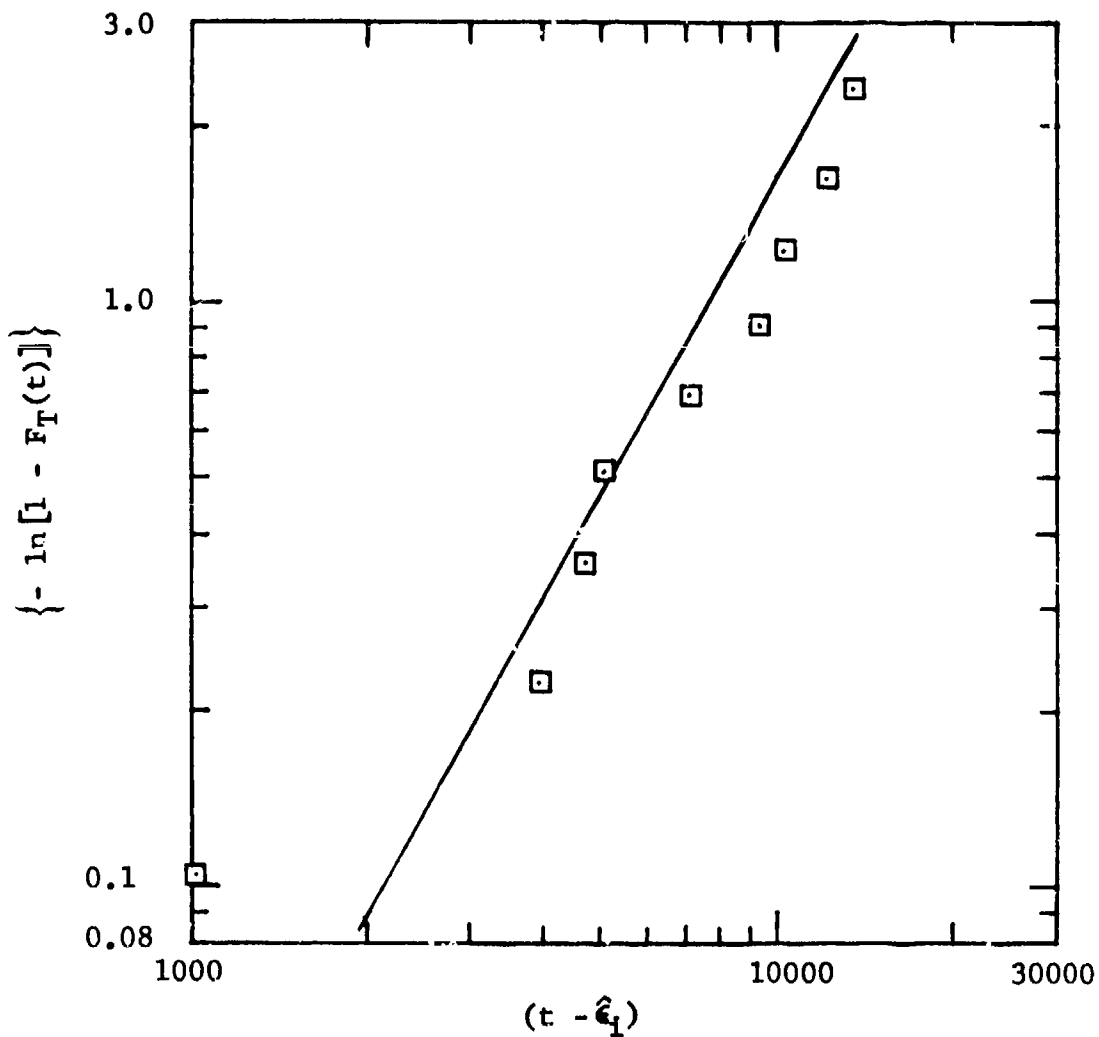
Fig. 4.15 TCI Goodness-of-Fit Plot for AFXMR4 Data Set Based on IFQ Model Parameters for Pooled Data Sets; a_0 = 0.050''
