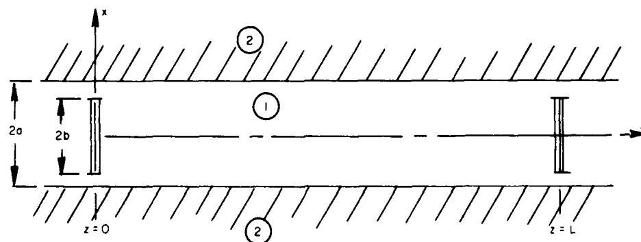
Figure A1. Configuration for Computing Diffraction Loss Due to Electrodes
