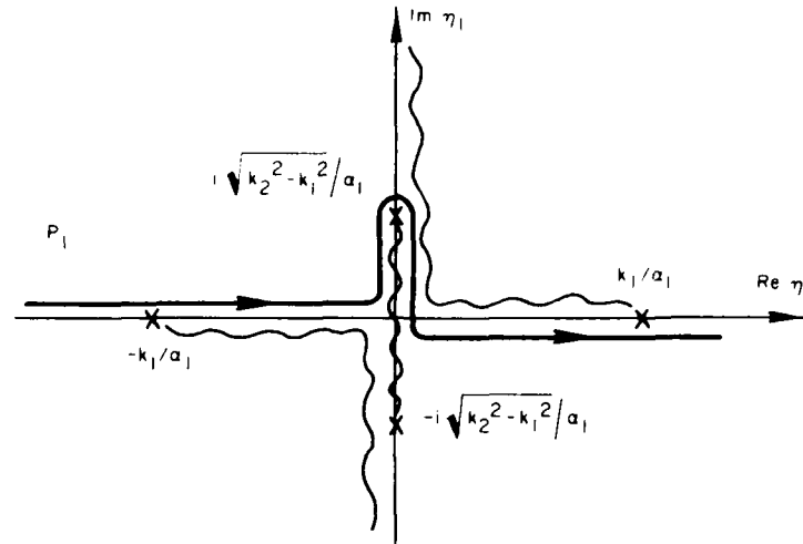
Figure A3. Integration Path in the Complex \eta Plane
