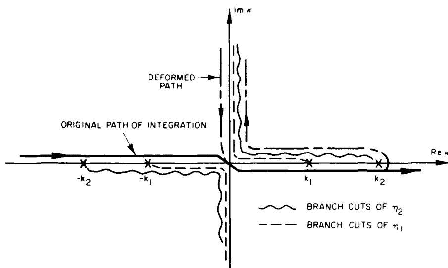
Figure A2. Integration Path in the Complex \kappa Plane
