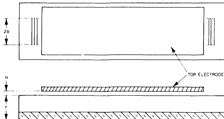
Figure 1. Top and Side Views of the Normal-field Electrode Configuration
