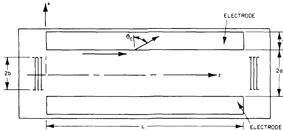
Figure 2. Top View of the Electrodes for the In-plane Field Configuration
