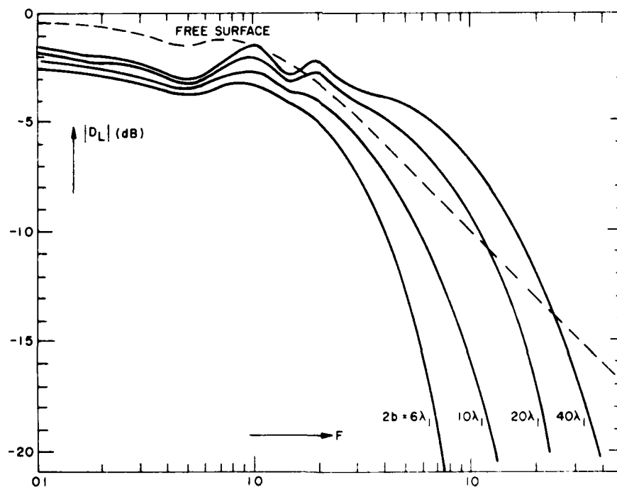
Figure 5. Variation of Diffraction Loss With Distance Parameter F for an Electrode Gap 2b
