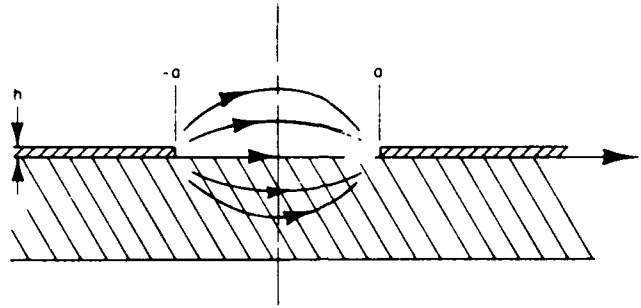
Figure 3. End View of the In-plane Field Configuration Showing the Fringing Static Electric Field
