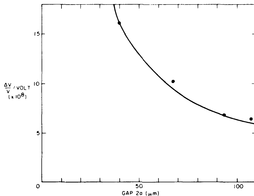
Figure 4. Variation of Voltage Sensitivity With Electrode Gap for the In-plane Field Configuration. Measured points are taken from Reference 11 for the 37-X cut of \text{LiNbO}_3
