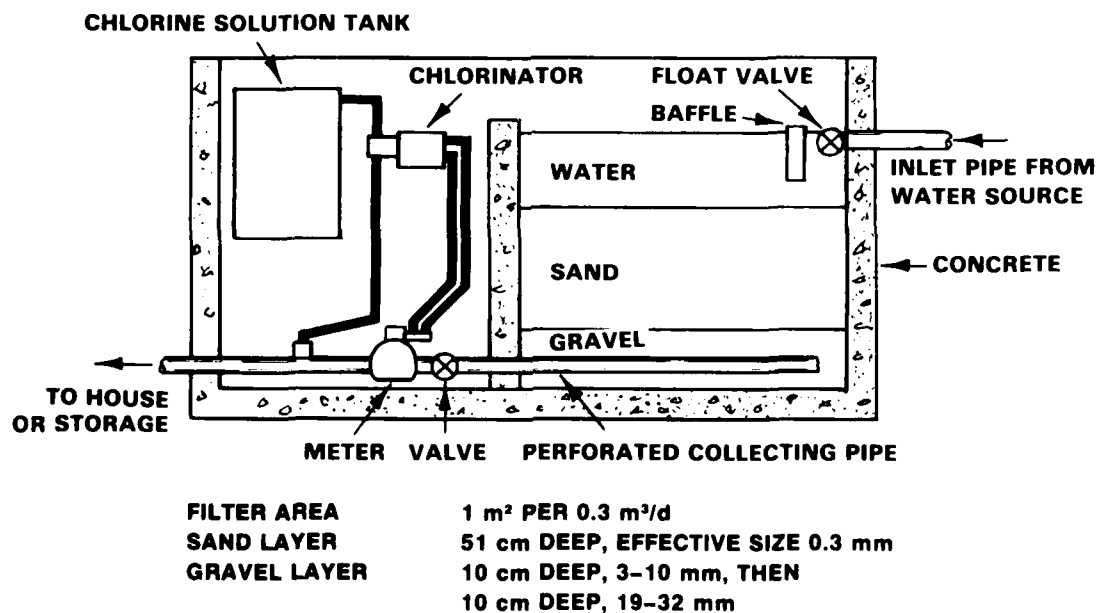
Figure 3. Filter-chlorinator for surface water and rainwater sources.
