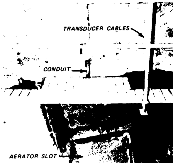
Figure 9. Entrance to aerator slot
