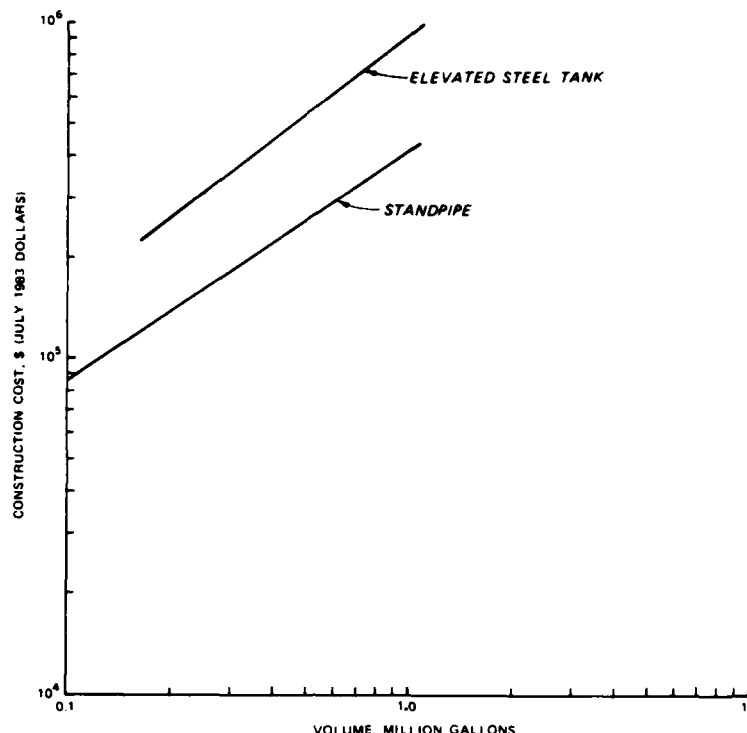
Figure 12. Typical construction costs for storage tanks
