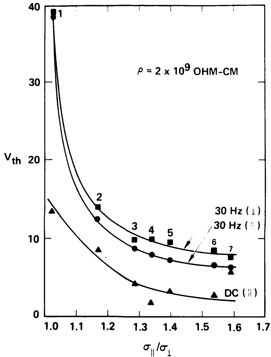
FIGURE 2 Dynamic scattering threshold voltage as a function of the conductivity anisotropy and surface alignment of HRL-2N25 containing the dopants in Table 1. (23°C, \rho_{\perp} = 2 \times 10^9 \text{ } \Omega\text{-cm} , ■-surface- \perp , ● and ▲-surface- \parallel ).
