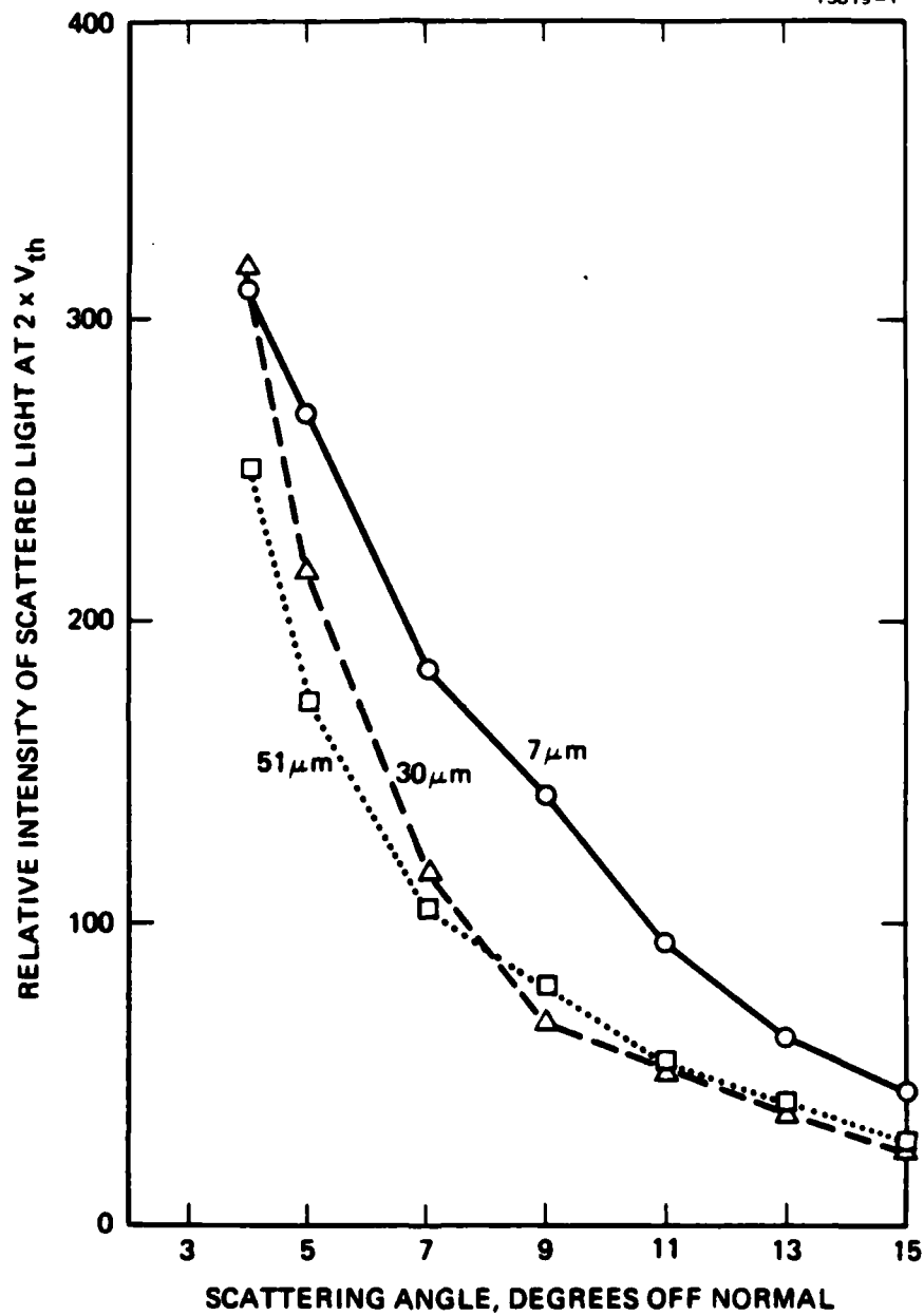
FIGURE 8 Cell thickness effect on off-angle DS intensity.
