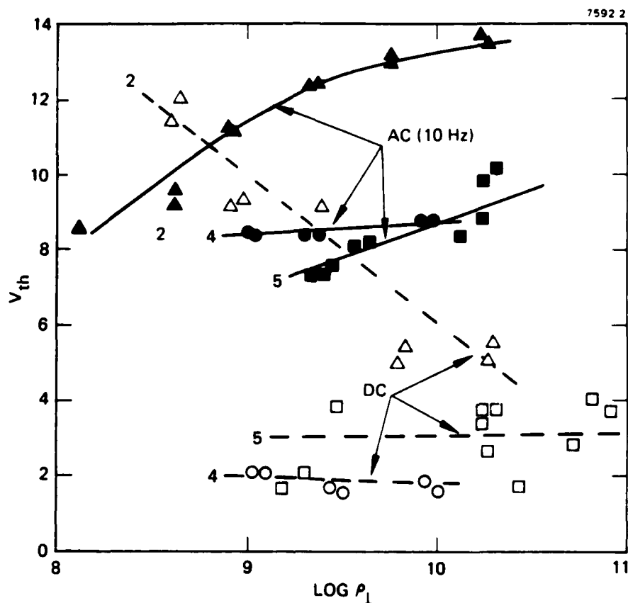
FIGURE 4 Effect of resistivity ( \rho_1 at 100 Hz) on dynamic scattering V_{th} of doped HRL-2N25 in 12.7 \mu\text{m} thick cells with surface-|| alignment, rubbed ITO. \circ, \bullet - TBATPB (4); \triangle, \blacktriangle - TBATMS (2); \square, \blacksquare - DBF/TFM (5).
