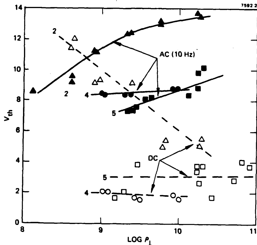
FIGURE 4 Effect of resistivity ( \rho_{\perp} at 100 Hz) on dynamic scattering V_{th} of doped HRL-2N25 in 12.7 \mu\text{m} thick cells with surface- \parallel alignment, rubbed ITO. \circ, \bullet - TBATPB (4); \Delta, \blacktriangle - TBATMS (2); \square, \blacksquare - DBF/TFM (5).
