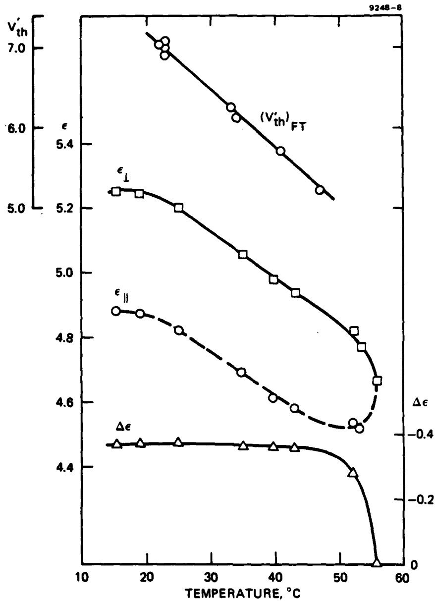
FIGURE 9 Temperature effects on dielectric properties and Fredericks transition of HRL-2N25 (undoped).
