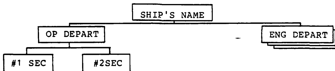
Figure 5.2 Hierarchical Model
