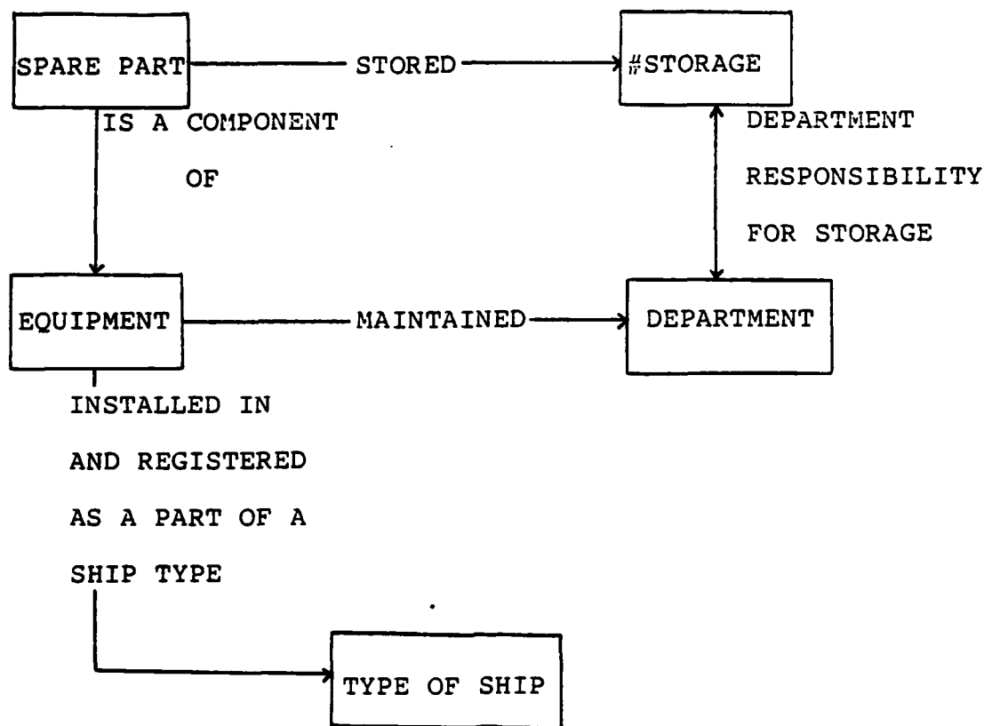
Figure 5.3 Network Model
