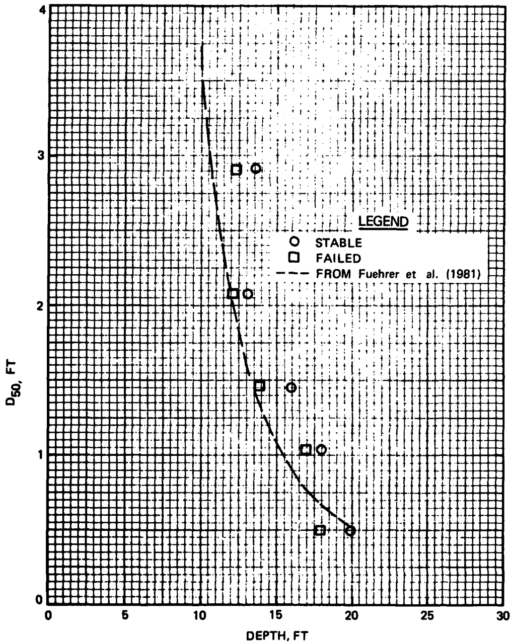
ROCK SIZE VS DEPTH COMPARISON OF MODEL RESULTS WITH FUEHRER'S DESIGN TECHNIQUE 5600-HP TOWBOAT STRAIGHT ATTACK W/O WALL EFFECTS SLACK-WATER CHANNEL
