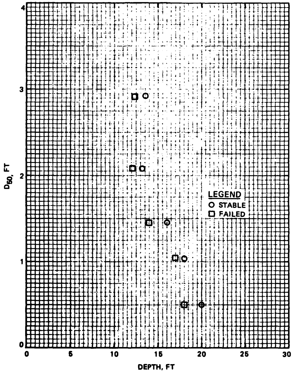
ROCK SIZE VS DEPTH MODEL RESULTS 5600-HP TOWBOAT STRAIGHT ATTACK W/O WALL EFFECTS SLACK-WATER CHANNEL
