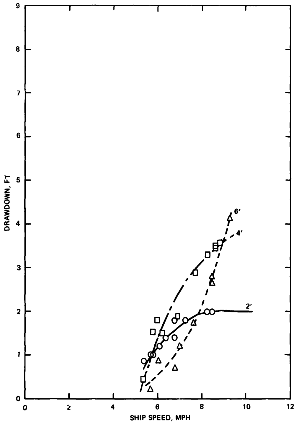
DRAWDOWN VS SHIP SPEED \eta = 4.3
