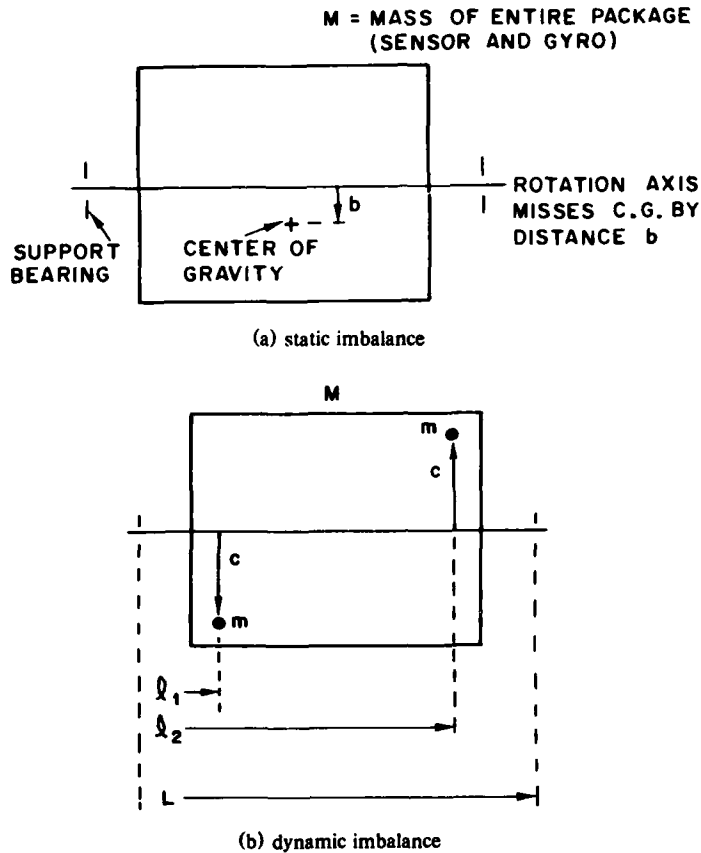
Fig. 5 - Geometry of (a) static and (b) dynamic imbalance. In (a), rotational motion of the package is induced by a translational acceleration of the support bearings perpendicular to the page, while in (b) a difference in the acceleration of the two bearings is required.
