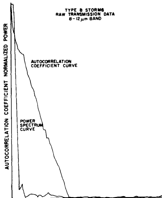
Figure 2a. Autocorrelation Coefficient Curve and Power Spectrum Curve of the Transmission Data in the 8-12 \mu\text{m} Band—Type B Storms
