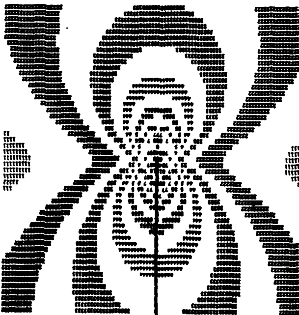
Figure 3. Pure Mode II ( K_{II} = 0.876 \text{ MPa}\sqrt{\text{m}} ) Isochromatics
