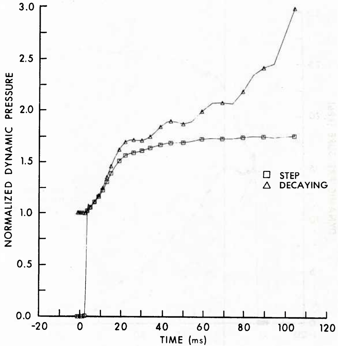
Figure 11. Normalized average dynamic pressure between the target and the outer boundary for 68.9 kPa shocks with 20 percent blockage.
