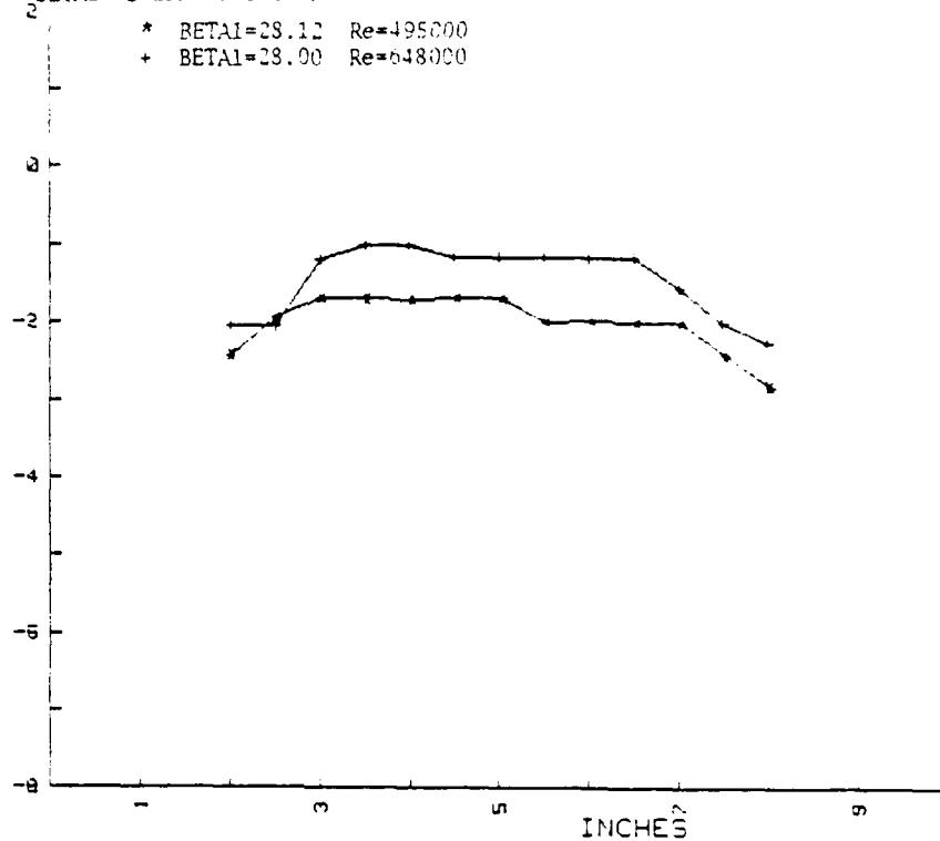
Q/Qref (lower plane) VS SPAN POSITION
