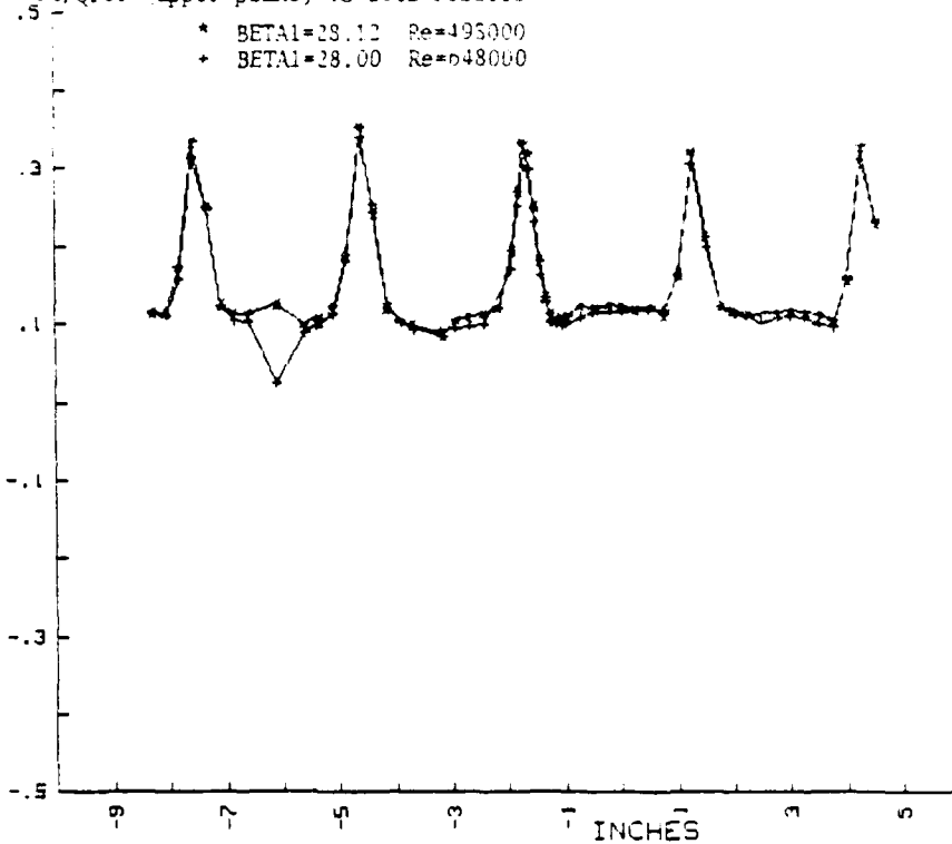
Figure A-33 X/X_{ref} (upper plane) VS BTOB POSITION
