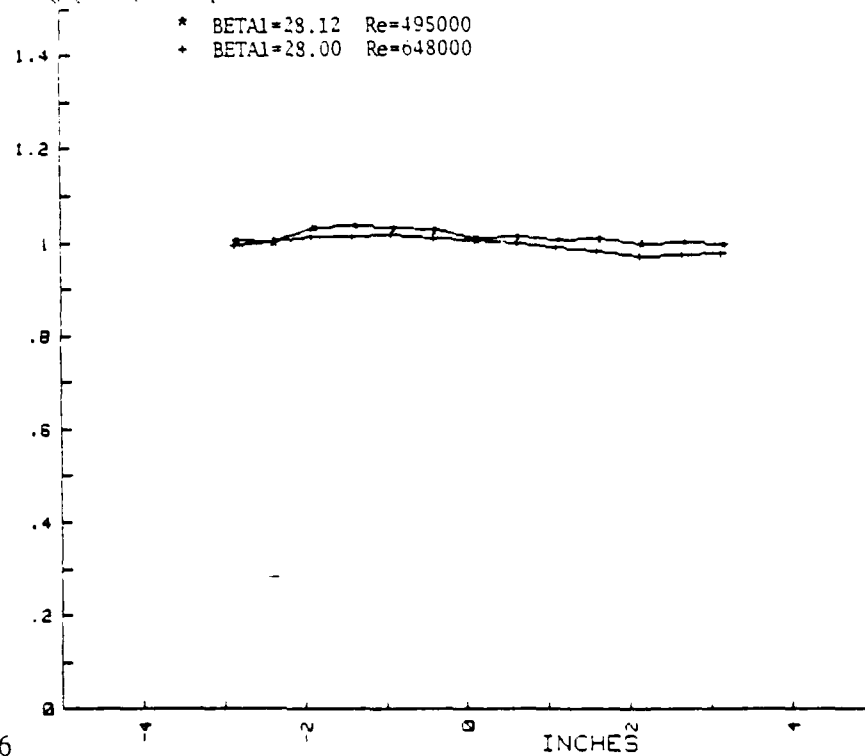
Q/Qref (lower plane) VS SPAN POSITION
