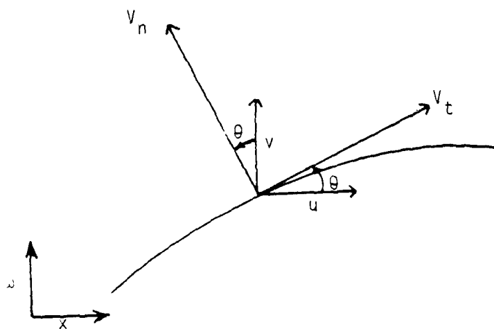
Figure 2. Velocity Components
